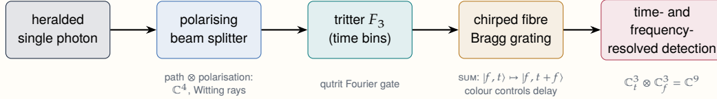
Figure 34. One photon, two qutrits. The controlled-add (sum) gate between the frequency and time qutrits has been demonstrated with a single passive element, a chirped fibre Bragg grating, at basis fidelity 0.92 \pm 0.01 [25].
