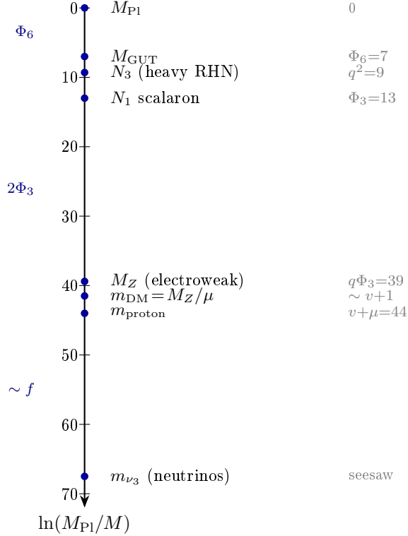
Figure 16: The mass spectrum of the universe as a cyclotomic descent from the Planck scale. Each scale sits at a substrate-integer depth \ln(M_{\text{Pl}}/M) : M_{\text{GUT}} at \Phi_6 = 7 , the heaviest right-handed neutrino N_3 at q^2 = 9 , the inflaton scalaron N_1 at \Phi_3 = 13 , the electroweak scale at q\Phi_3 = 39 , the dark matter M_Z/\mu just below, the proton at v + \mu = 44 , and the light neutrinos at the seesaw floor \sim 68 . The gaps between rungs are themselves cyclotomic ( \Phi_6, 2\Phi_3, \sim f ). One axis, one descent, the whole mass spectrum from q = 3 .
