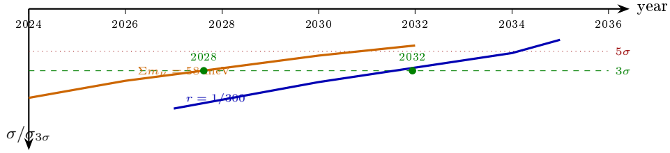
Figure 20: The kill-shot dashboard: computed discovery dates. Forecast \sigma(t) for the two clean discovery observables, each normalised to its own 3\sigma threshold ( \sigma_{3\sigma} = \text{pred}/3 ), declining as the experiments improve. Where a curve crosses the green dashed line the substrate prediction is a 3\sigma detection: \Sigma m_\nu = 58 \text{ meV} \sim 2028 (DESI+CMB-S4) and r = 1/300 \sim 2032 (SO→CMB-S4→LiteBIRD), with 5\sigma (red dotted) by \sim 2030 and \sim 2034 . The \Sigma m_\nu detection assumes the NH-minimum value is true (current data could instead yield an exclusion, which would falsify). Precision/coverage kill-shots (not shown): JUNO pins \Delta m_{31}^2/\Delta m_{21}^2 = 33 by \sim 2030 ; LZ covers m_{\text{DM}} = 22.8 \text{ GeV} by \sim 2028 .
