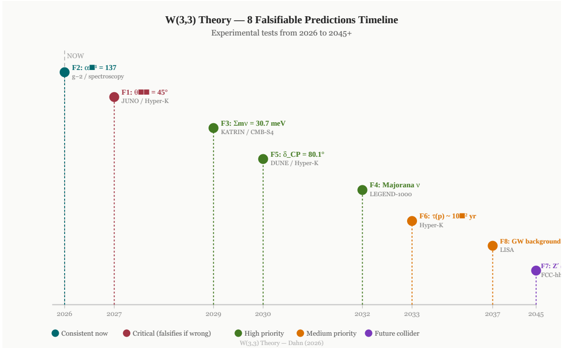
Figure 3: Timeline of the eight W(3, 3) -theory falsifiable predictions (2026–2045+). The vertical dashed line marks the present (2026). F1 ( \theta_{23} = 45^\circ , JUNO 2027) is the critical near-term test. F3 ( \Sigma m_\nu = 30.7 \text{ meV} , KATRIN/CMB-S4) and F5 ( \delta_{CP} = 80.1^\circ , DUNE) form a five-year conjunctive window. F7 ( Z' at 1094 GeV) requires FCC-hh.
