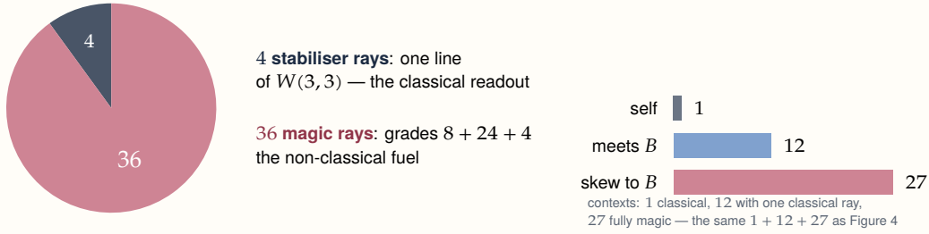
Figure 31. The machine’s quantum resource is the geometry itself: remove one line and every remaining point is a magic state.
