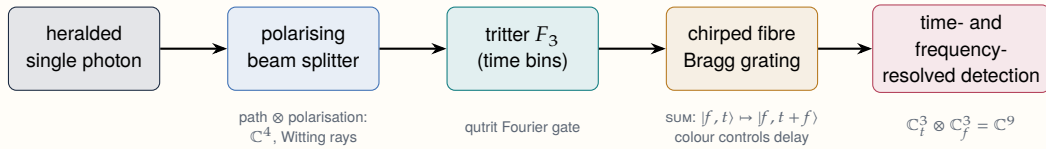
Figure 32. One photon, two qutrits. The controlled-add (sum) gate between the frequency and time qutrits has been demonstrated with a single passive element, a chirped fibre Bragg grating, at basis fidelity 0.92 \pm 0.01 [19].
