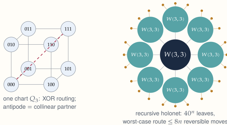
Figure 34. Left: a local routing chart. Each of the 540 pairs of disjoint lines of W(3, 3) carries a cube of eight points with XOR addressing. Right: substituting a copy of W(3, 3) at every point gives a network with 40^n leaves and logarithmic routing.
