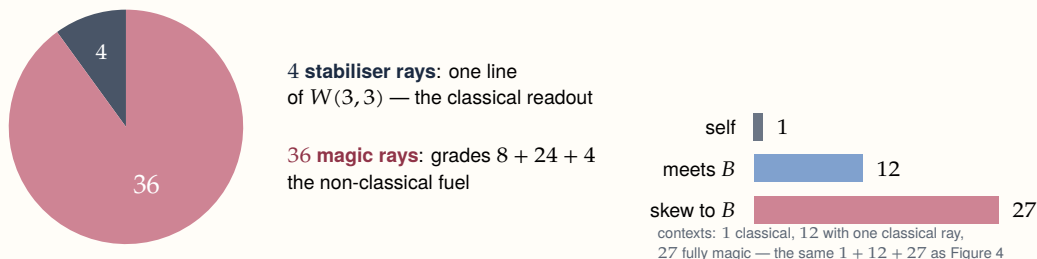
Figure 33. The machine’s quantum resource is the geometry itself: remove one line and every remaining point is a magic state.
