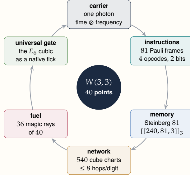
Figure 31. The Holonet stack. Every layer is a structure of W(3,3) read as engineering: the Pauli frames are the 81 points of \mathbb{F}_3^4 , the memory is the Steinberg module, the network is the geometry's atlas of cube charts, the fuel is its set of magic states, and the universal gate is the E_6 cubic of Section 5.
