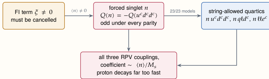
Figure 30. Why supersymmetric vacua of the class violate R -parity. The only fields that can cancel the Fayet–Iliopoulos term carry exactly the conjugate charge of the three dimension-four operators. Every string selection rule allows the resulting quartic couplings, so the vacuum turns the cubic operators back on.
