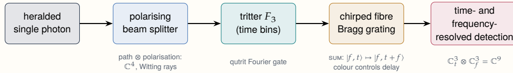
Figure 33. One photon, two qutrits. The controlled-add (sum) gate between the frequency and time qutrits has been demonstrated with a single passive element, a chirped fibre Bragg grating, at basis fidelity 0.92 \pm 0.01 [19].
