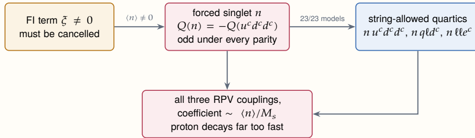
Figure 30. Why supersymmetric vacua of the class violate R -parity. The only fields that can cancel the Fayet–Iliopoulos term carry exactly the conjugate charge of the three dimension-four operators. Every string selection rule allows the resulting quartic couplings, so the vacuum turns the cubic operators back on.
