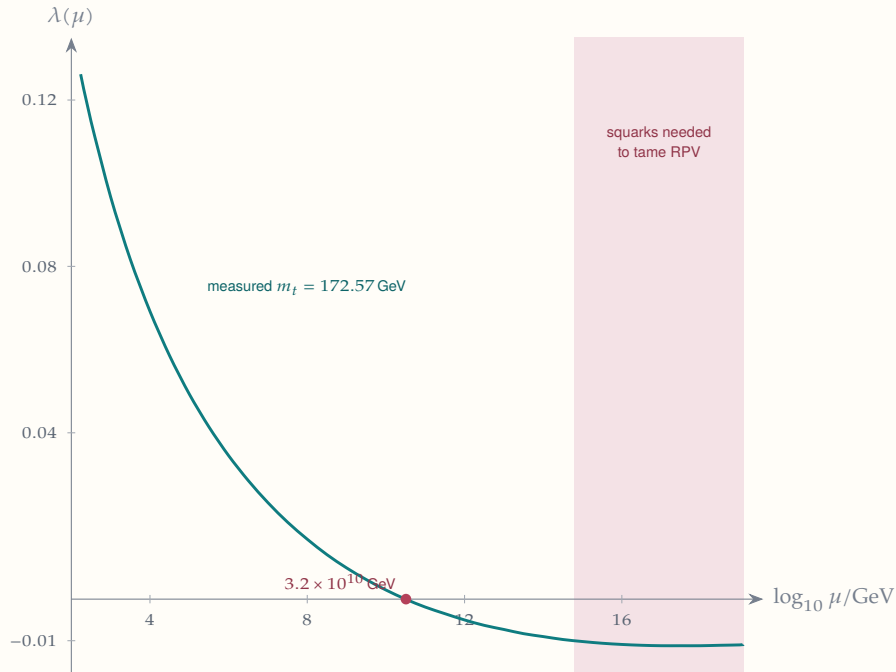
Figure 31. The Higgs self-coupling run to high energy (two loops, NNLO matching). It turns negative near 3 \times 10^{10} GeV, far below the \geq 6 \times 10^{14} GeV that heavy squarks would need to make the regenerated R -parity violation harmless (shaded).
