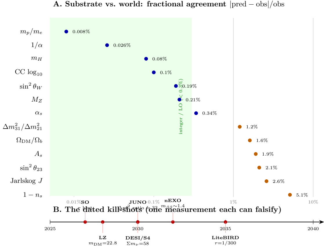
Figure 19: The whole substrate tower on one axis. A: every measured observable’s fractional agreement |\text{pred} - \text{obs}|/\text{obs} (log scale). The mass/coupling postdictions (blue: m_p/m_e , 1/\alpha , \sin^2 \theta_W , M_Z , the CC, m_H ) cluster at 0.01–0.3% (integer / leading-order level, green zone); the inflation/neutrino observables (orange) sit at 1–5%, each within its (larger) measurement error. The common axis is fractional deviation, not \sigma (the blue points are integer/LO postdictions whose residual is higher-order running; the orange points are measurement-limited). B: the dated falsification frontier — each future test is one measurement that can kill the theory: m_{\text{DM}} (LZ \sim 2028 ), the first r hint (SO \sim 2027 ), the \Delta m^2 ratio (JUNO), \Sigma m_\nu (DESI/CMB-S4), m_{\beta\beta} (nEXO/LEGEND), and the headline r = 1/300 (LiteBIRD \sim 2035 ). One q = 3 alphabet, \sim 20 numbers, all consistent — and decided by the mid-2030s.
