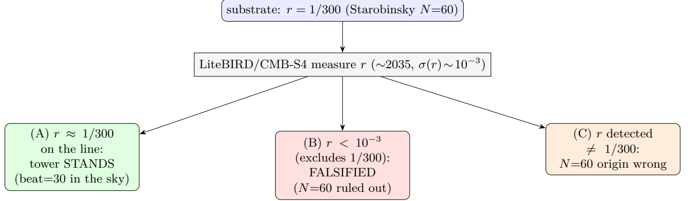
Figure 18: The theory lives or dies on r by \sim 2035 . The substrate predicts r = 12/N^2 = 1/300 ( N = 2 beat = 60, Starobinsky). A LiteBIRD/CMB-S4 measurement ( \sigma(r) \sim 10^{-3} , a 3\text{--}7\sigma detection of r = 1/300 ) yields three clean verdicts: (A) r \approx 1/300 on the line r = 3(1 - n_s)^2 confirms the tower; (B) r < 10^{-3} falsifies the Starobinsky N = 60 spectrum; (C) r detected away from 1/300 breaks the beat=30 \rightarrow N=60 origin.
