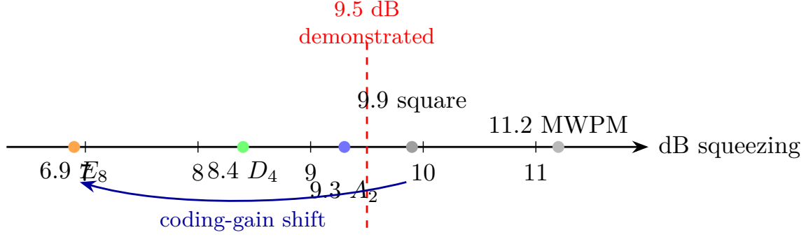
Figure 12: The fault-tolerance threshold as a lab number. The measured square-GKP + surface-code threshold (9.9 dB, Noh–Chamberland 2022; 11.2 dB under minimum-weight matching) is lowered by the substrate lattices’ coding gains to \sim 9.3/8.4/6.9 dB for A_2/D_4/E_8 — all at or below the 9.5 dB squeezing already demonstrated in hardware. (Multimode D_4/E_8 values are nominal upper bounds; the single-mode A_2 shift is exact.)
