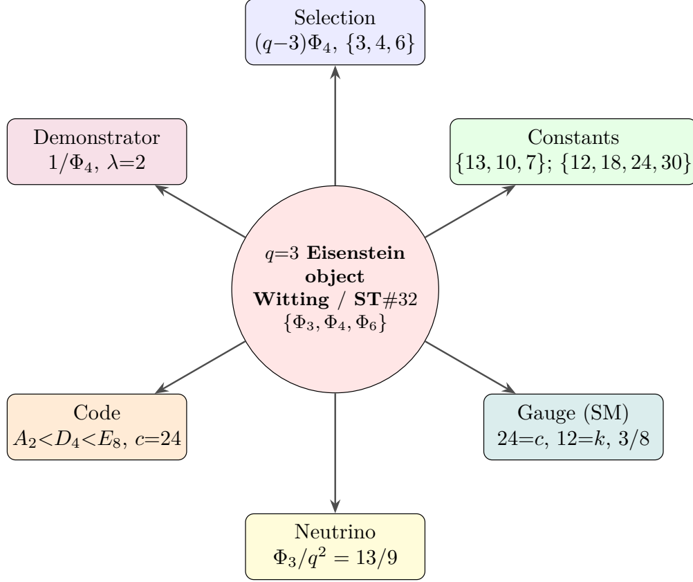
Figure 9: The q = 3 substrate is one Eisenstein object — the Witting polytope, its symmetry ST#32, the cyclotomic skeleton \{\Phi_3, \Phi_4, \Phi_6\} — seen from six sides. The selection of q = 3 , the substrate constants, the Standard-Model gauge group, the neutrino mass hierarchy, the fault-tolerant code lattice, and the benchtop experiment are faces of the same structure, sharing the same invariants ( 240 = E_8 roots, \{\Phi_3, \Phi_4, \Phi_6\} , the Witting degrees \{12, 18, 24, 30\} , 155520 = 3|\text{Aut}(W(3, 3))| ).
