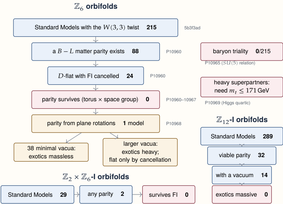
Figure 28. The vacuum gauntlet. Blue: filters passed; red: dead ends; gold: the one door still ajar. Every count is exact (Farkas certificates, Smith normal forms, lattice tests and integer programs), and each is regenerated by the script named in the ledger.
