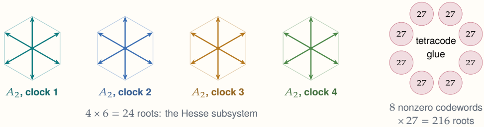
Figure 12. E_8 assembled from four clocks. Each Hesse clock contributes one A_2 root system (left). The remaining 216 roots come in eight sectors of 27, one for each nonzero word of the tetracone (right): 240 = 4 \cdot 6 + 8 \cdot 27 .
