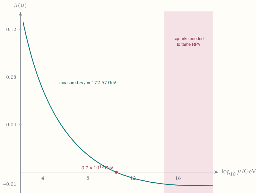
Figure 32. The Higgs self-coupling run to high energy (two loops, NNLO matching). It turns negative near 3 \times 10^{10} GeV, far below the \geq 6 \times 10^{14} GeV that heavy squarks would need to make the regenerated R -parity violation harmless (shaded).
