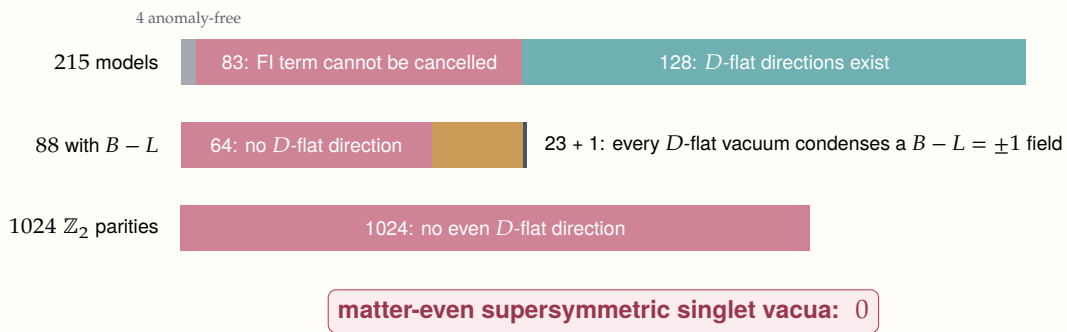
Figure 29. The exhaustive closure of Theorem 9.6. Every one of the 215 models is accounted for; no branch leaves a matter-parity-preserving supersymmetric vacuum in singlet directions.
