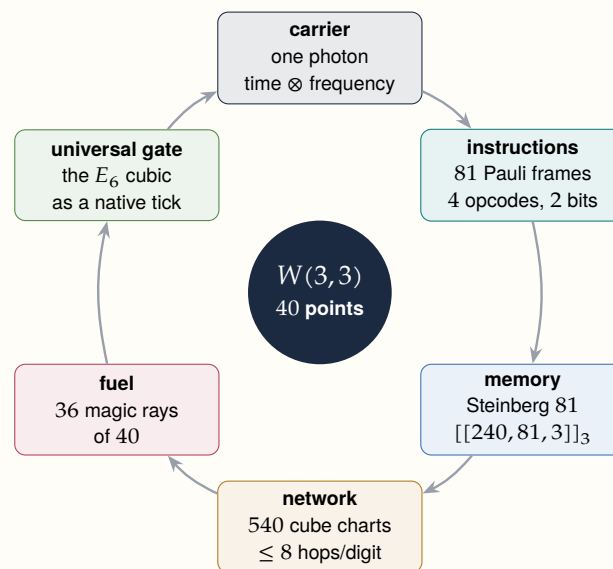
Figure 33. The Holonet stack. Every layer is a structure of W(3,3) read as engineering: the Pauli frames are the 81 points of \mathbb{F}_3^4 , the memory is the Steinberg module, the network is the geometry’s atlas of cube charts, the fuel is its set of magic states, and the universal gate is the E_6 cubic of Section 5.
