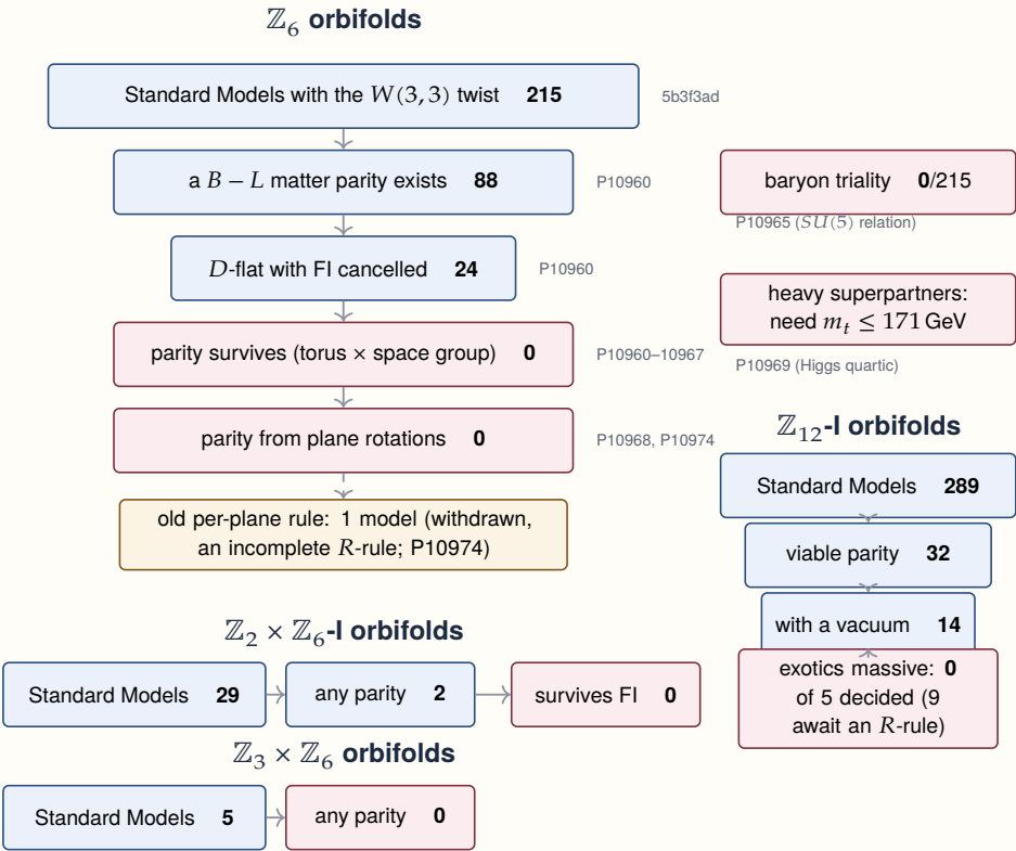
Figure 28. The vacuum gauntlet. Blue: filters passed; red: dead ends; gold: a door that looked open and was withdrawn. Every count is exact (Farkas certificates, Smith normal forms, lattice tests and integer programs), and each is regenerated by the script named in the ledger.
