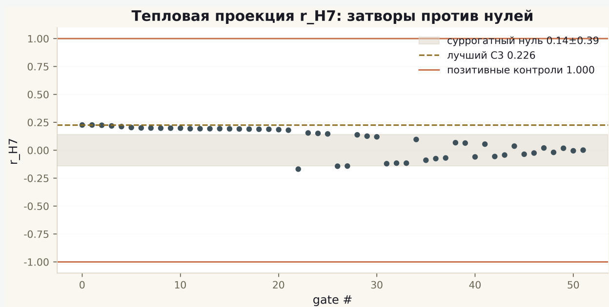
Fig. 1. r_{H7} across the 52 gates: grey band — null zone, gold line — best gate 0.226, copper lines — positive controls \pm 1 .
