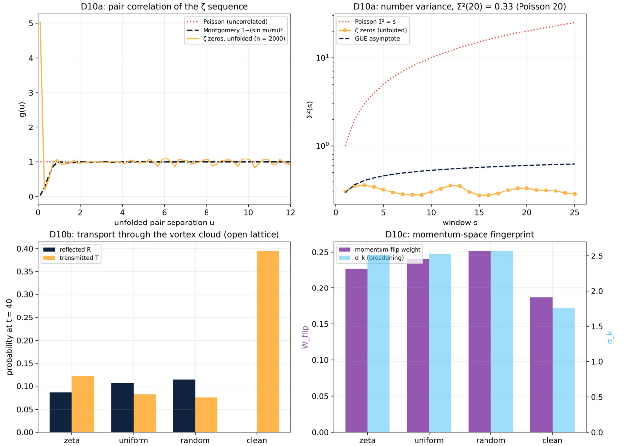
Figure 10. Test D10. Top left: the pair correlation g(u) of the unfolded zeta sequence against the Montgomery form and the Poisson baseline. Top right: the number variance \Sigma^2(s) - 0.33 at s = 20 against the Poisson value 20. Bottom left: reflected and transmitted probability for the four equal-density configurations - the zeta cloud is the most transparent. Bottom right: the momentum-space fingerprint - flip weight and packet broadening ordered zeta < uniform < Poisson.
