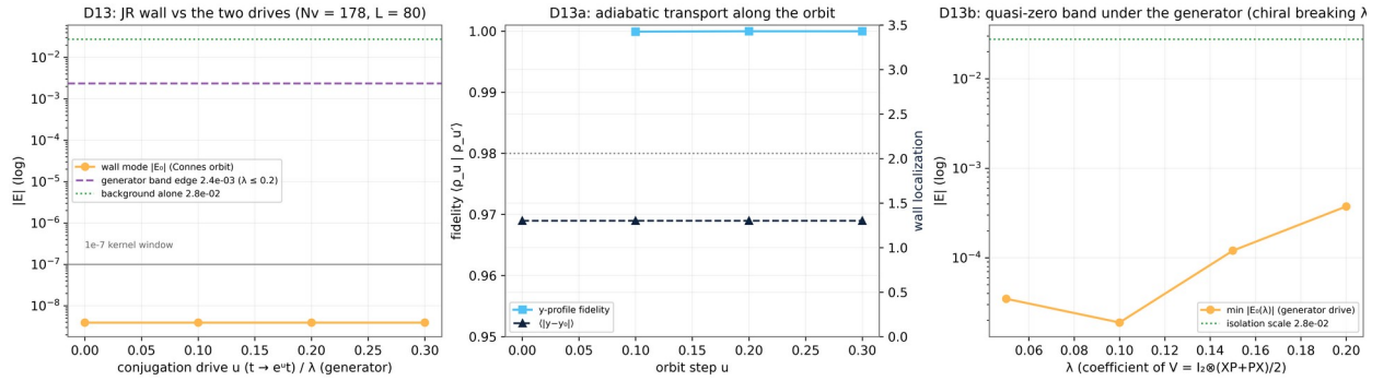
Figure 13. Test D13. Left: the wall-mode energy under both drives - pinned at 3.9e-9 along the Connes orbit, lifted only to \text{gap}/679 by the generator at \lambda = 0.2 , with the background control and the 1e-7 kernel window marked. Center: the adiabatic transport along the orbit (y-profile fidelity and wall localization). Right: the quasi-zero band under the generator against the isolation scale.
