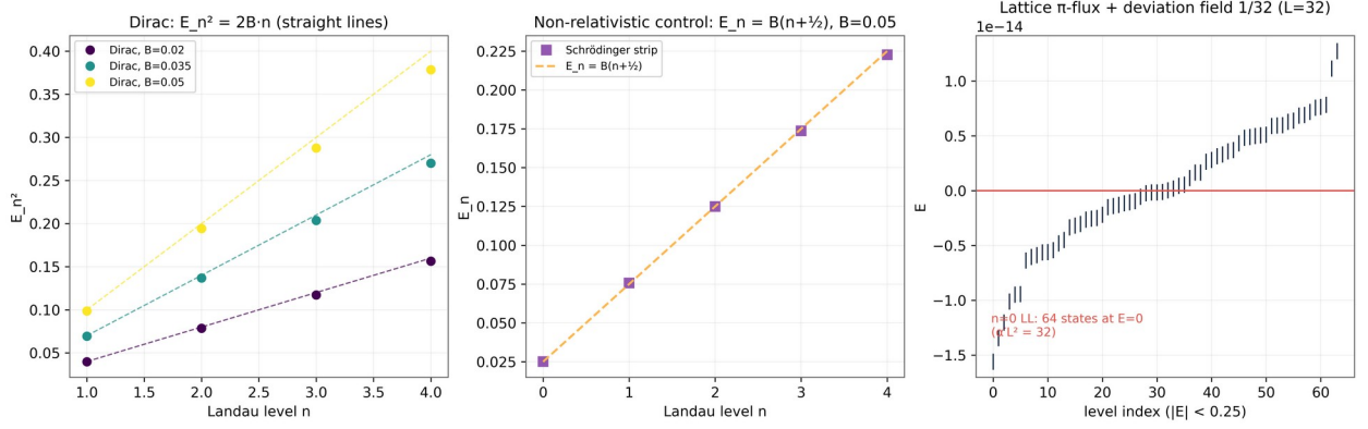
Figure 4. Test D4, Left: Dirac Landau ladders E_n -squared against n for three field strengths - straight lines through the origin, slopes matching 2 \nu_F -squared B . Center: the Schrodinger control ladder E_n = B(n + 1/2) on the identical strip. Right: the lattice \pi -flux model with deviation field 1/q - the chiral n = 0 Landau level pinned at E = 0 .
