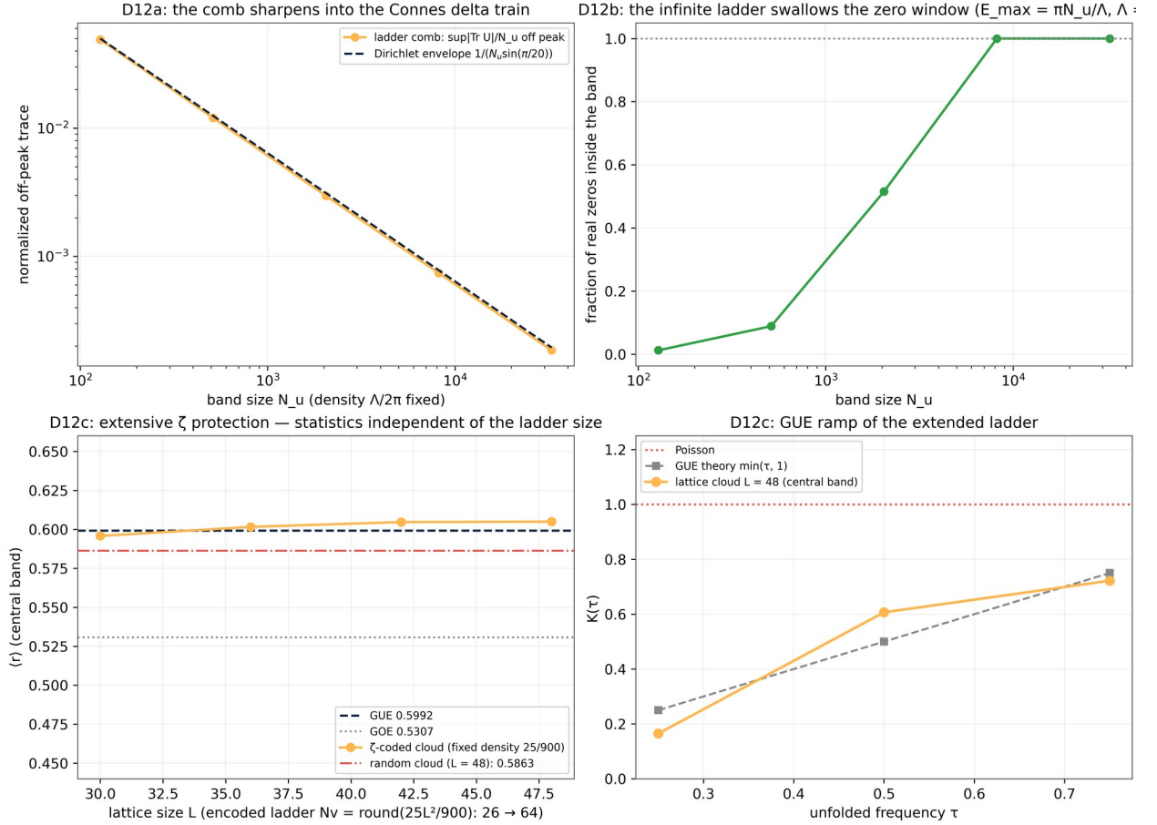
Figure 12. Test D12. Top left: the off-peak trace of the conjugation action follows the Dirichlet envelope 1/(N_u \sin(\pi/20)) over two decades of band size - the comb sharpens into the Connes delta train. Top right: the extending band swallows the real-zero window (coverage = 1 at N_u = 8192 ). Bottom left: the GUE statistics are L -independent at fixed vortex density while the encoded ladder grows N_v = 25 \rightarrow 64 (clean and random baselines shown). Bottom right: the GUE ramp of the L = 48 cloud form factor.
