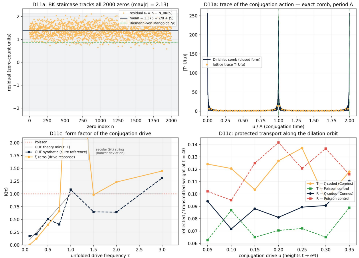
Figure 11. Test D11. Top left: the Berry-Keating staircase residual r_n = n - (t_n/2\pi) \cdot \ln(t_n/2\pi e) over the real zero ladder - mean 1.3750 ( 7/8 + \langle S \rangle ), max 2.13. Top right: the trace of the conjugation action against the closed-form Dirichlet comb, two exact periods \Lambda . Bottom left: the drive form factor K(\tau) - zeta zeros against the suite's synthetic GUE reference and the Poisson line; the shaded region \tau \geq 1 carries the secular S(t) string
