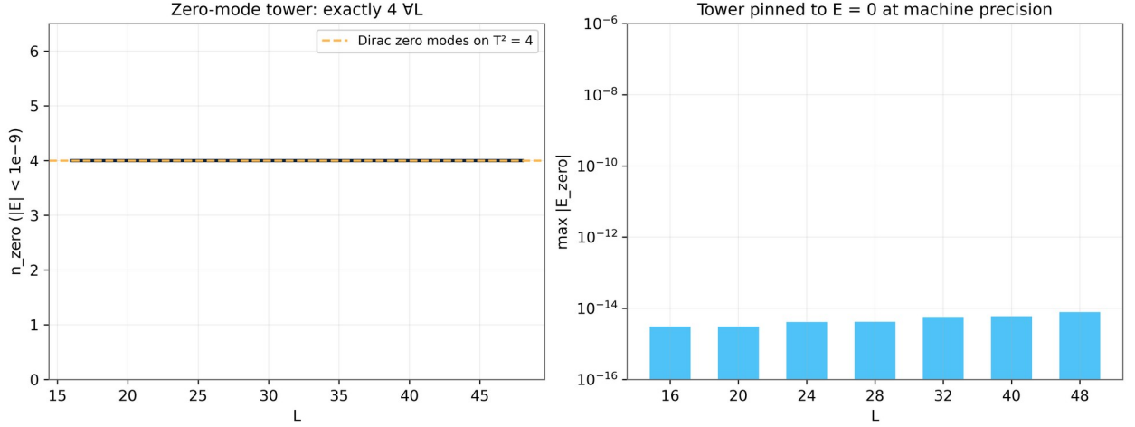
Figure 2. Test D2. Left: the zero-mode count across the L -ladder - exactly four modes at every size (dashed line: the Dirac zero modes on the torus). Right: the maximal |E| inside the tower, at machine precision (log scale).
