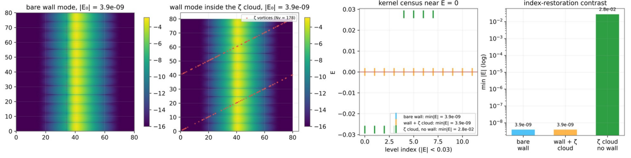
Figure 9. Test D9. Left: the wall-mode density (log scale) for the bare Jackiw-Rebbi wall, |E_0| = 3.9\text{e-}09 . Center-left: the same mode inside the full zeta-vortex background ( N_v = 178 , red dots) - unchanged. Center-right: the kernel census near E = 0 for the bare wall, the wall in the zeta cloud, and the wall-less control. Right: the restoration contrast on a log scale - the wall rebinds the zero mode 7 \times 10^6 below the bare background sector.
