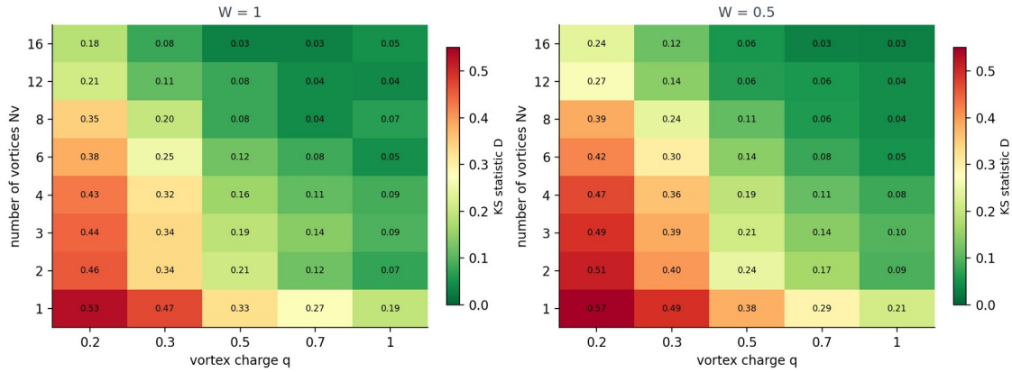
Fig. 20. The KS-distance landscape D(N_v, q) on the L = 24 scan (Stage A; open boundaries, protocol placement, \alpha = 0.5 ): left — W = 1.0 , right — W = 0.5 . The valley N_v \approx 8 – 16 at q \approx 0.7 – 1.0 is visible in both slices; the pure lattice N_v = 0 sits at D \approx 0.73 , far off the color scale.
