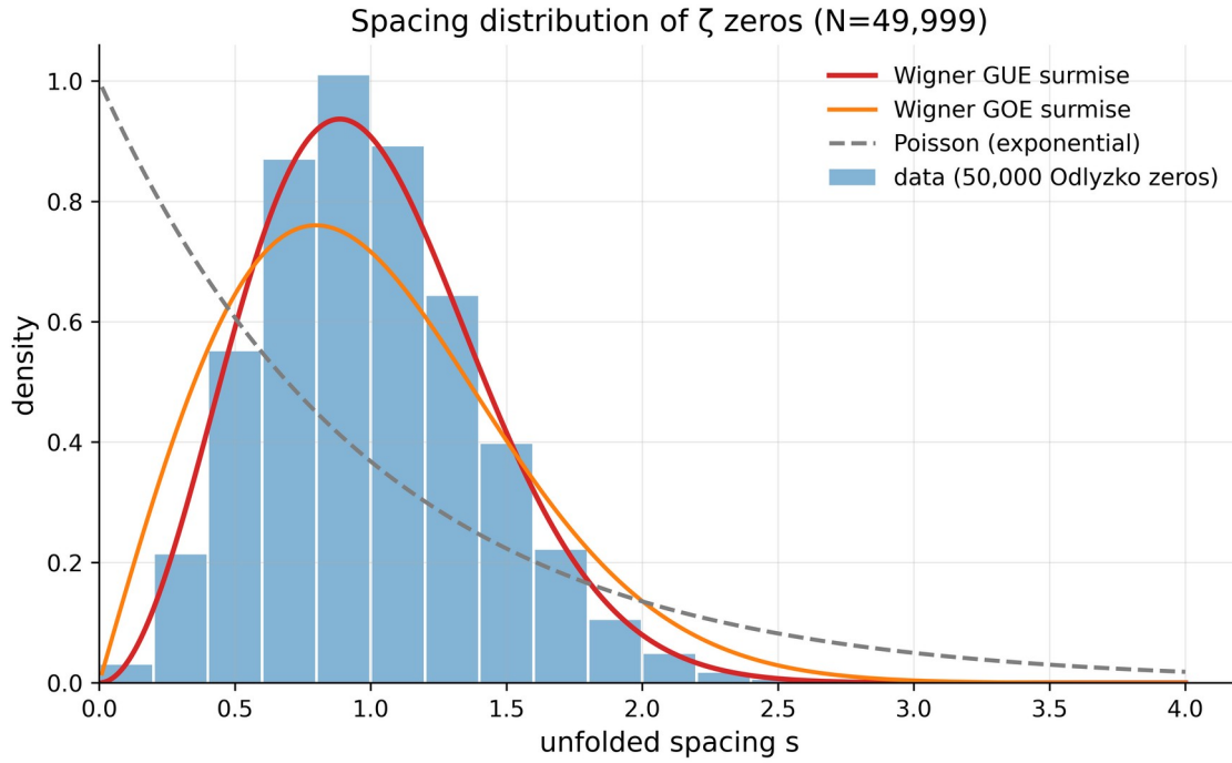
Fig. 2. Histogram of 49,999 \zeta -zero spacings against the Wigner surmises (GUE, GOE) and the Poisson exponential: a typically “matrix-like” shape with level repulsion.
