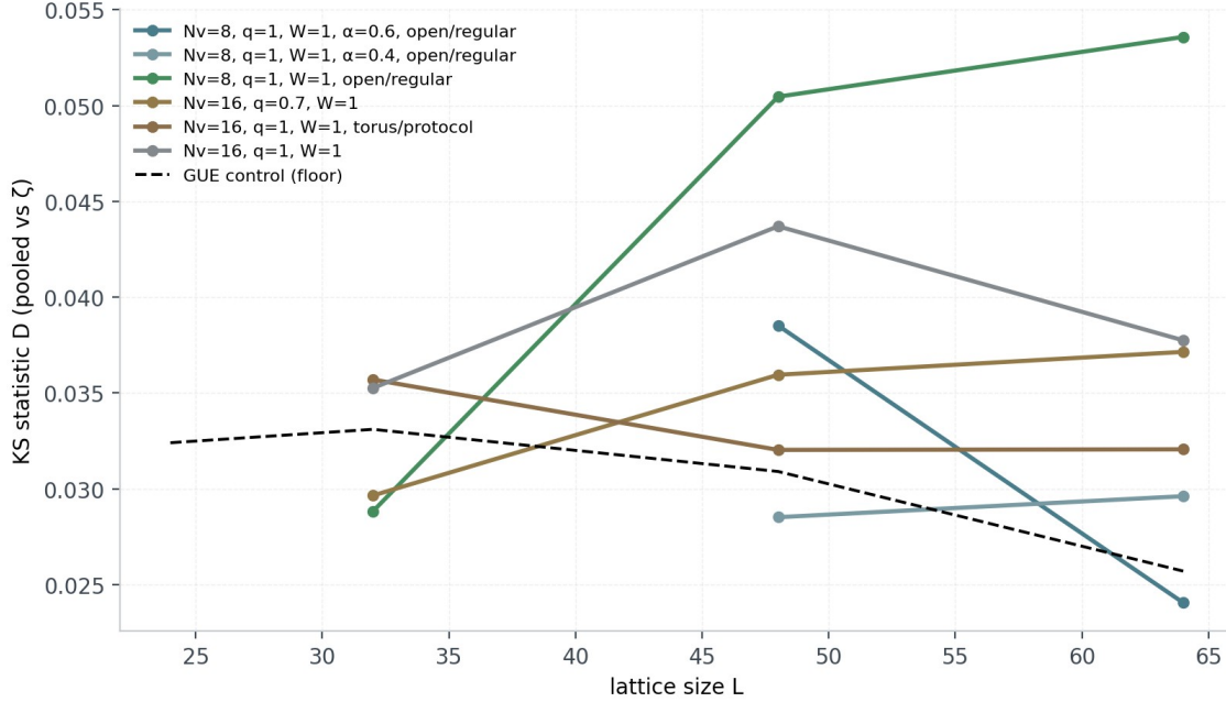
Fig. 21. The size ladder L = 24 \rightarrow 64 for the six leading Stage-B configurations (pooled D per lattice size; solid curves) against the per- L GUE floor (dashed). The optimized window stays at or near the floor as the lattice grows; the dilute configurations plateau roughly three times above it.
