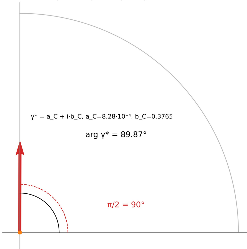
Fig. 17. The spinorial phase \gamma^i = a_C + i b_C : argument 89.87^\circ against the reference 90^\circ ; the dominance of b_C presses the phase to \pi/2 .
