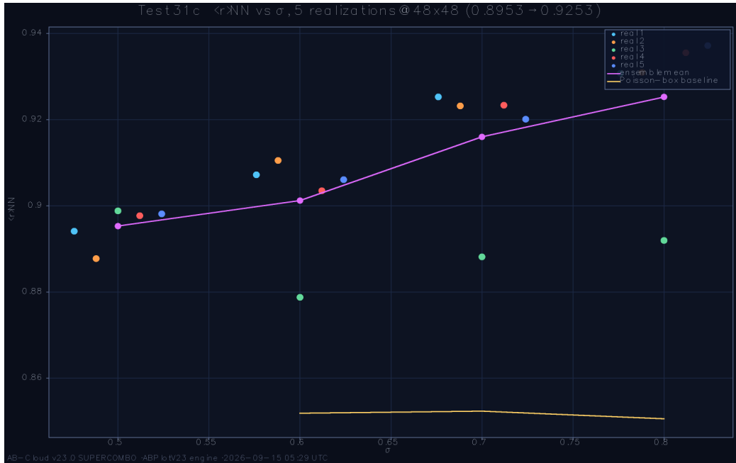
Figure 39: The Hatano-Nelson series: spectral statistics across the non-Hermitian deformation, from the GUE basin toward Poisson.
