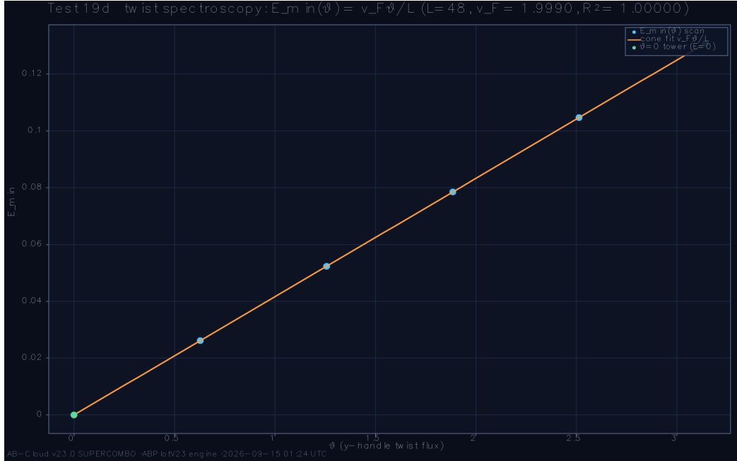
Figure 14: The Dirac cone at self-dual flux: band crossing at zero energy with linear dispersion.
