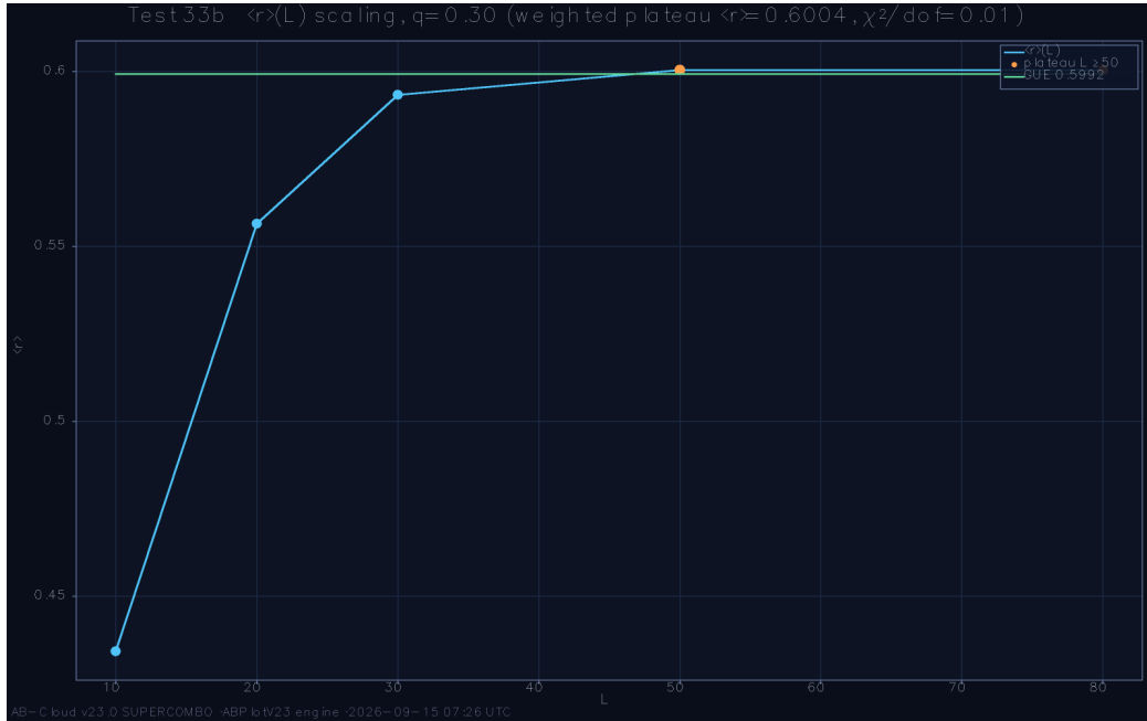
Figure 41: The L-scaling of \langle r \rangle : 0.434 to 0.6004 across the size ladder, with the GUE \chi^2 comparison at the plateau.
