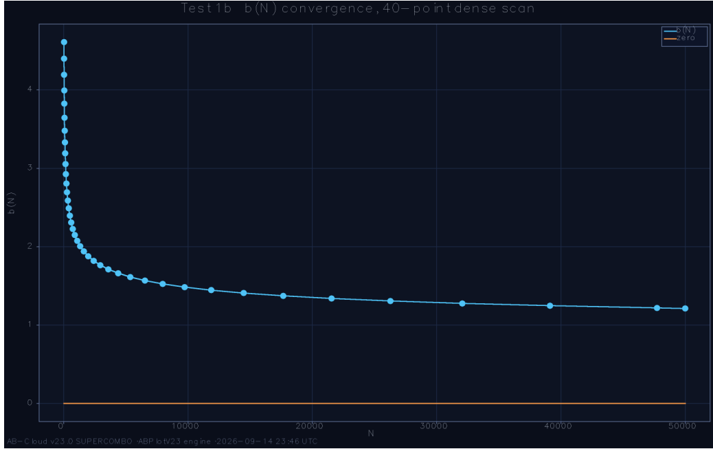
Figure 1: Convergence of the dictionary displacement b(N) : the cumulative deviation between the paired Gram-point and zero sequences as the pairing proceeds across the first 50,000 zeros.
