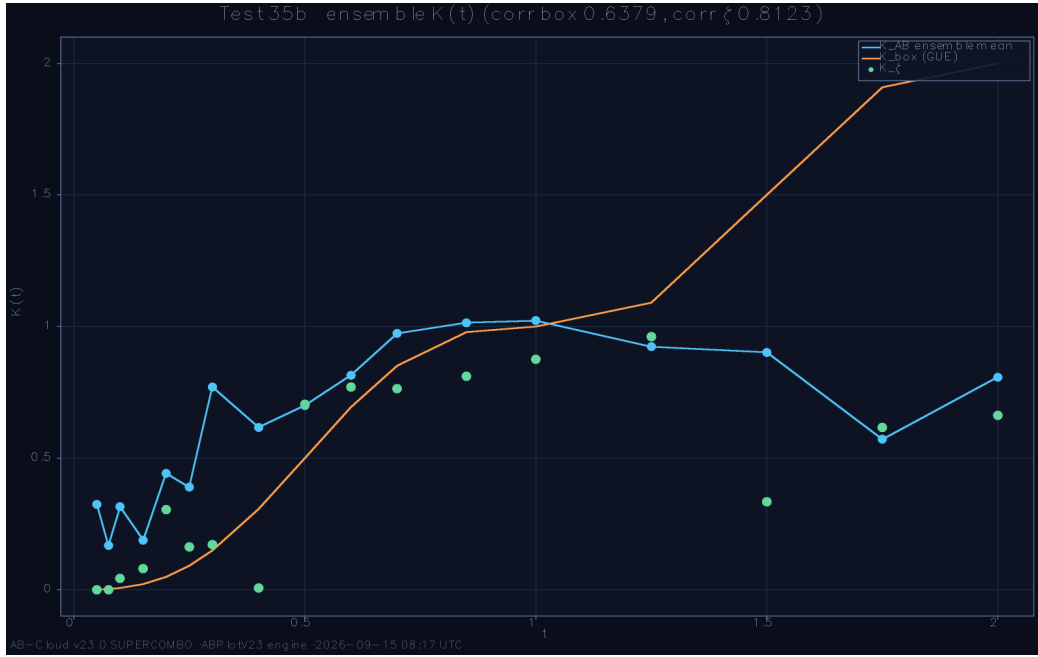
Figure 42: The spectral form factor K(t) : ramp and plateau against the GUE prediction; the knee sits at the predicted Heisenberg time.
