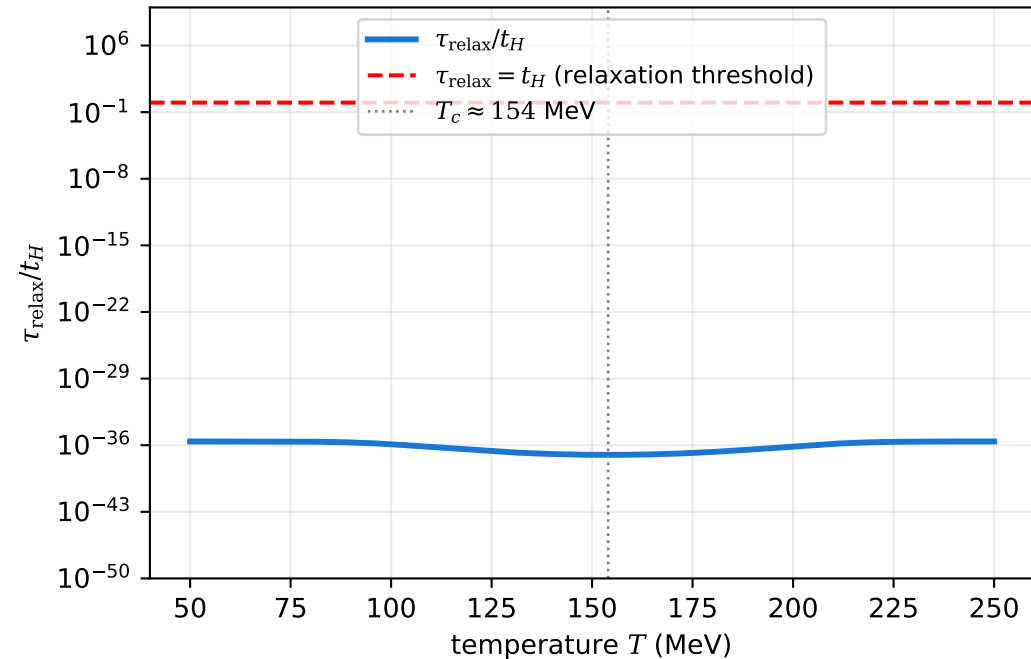
(a) Dynamic relaxation timescale near T_c
