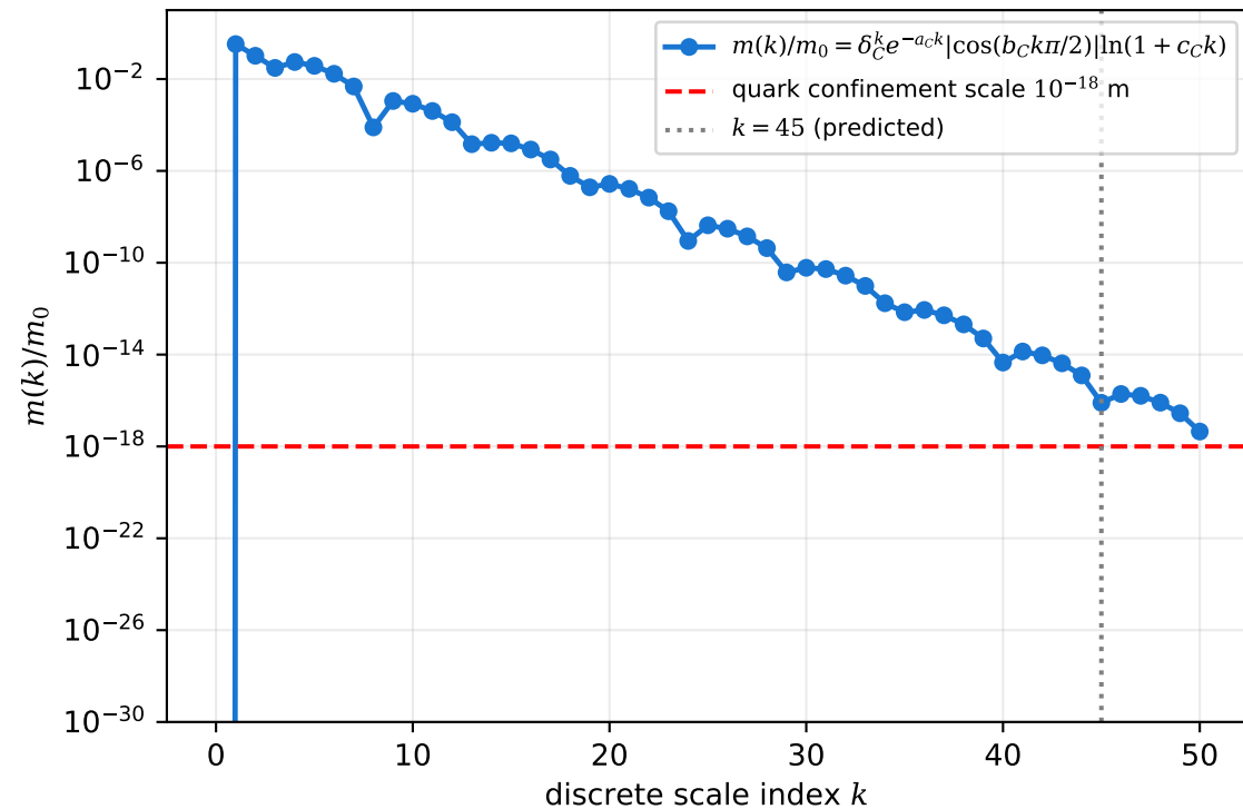
(a) 4D-PSL(2,7) jet-wake mass ladder
