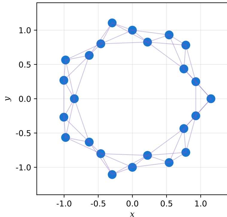
(b) 24 vertices of the PSL(2, 7)/ C_7 lattice
