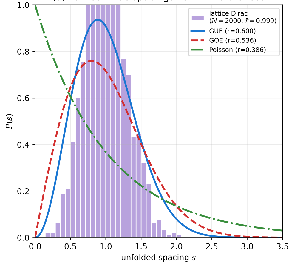
(a) Lattice Dirac spacings vs RMT references
