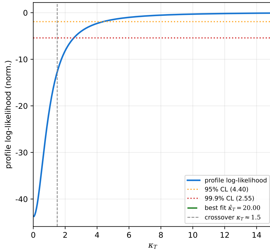
(b) Pandey--Mehta fit: \kappa_T for real QCD
