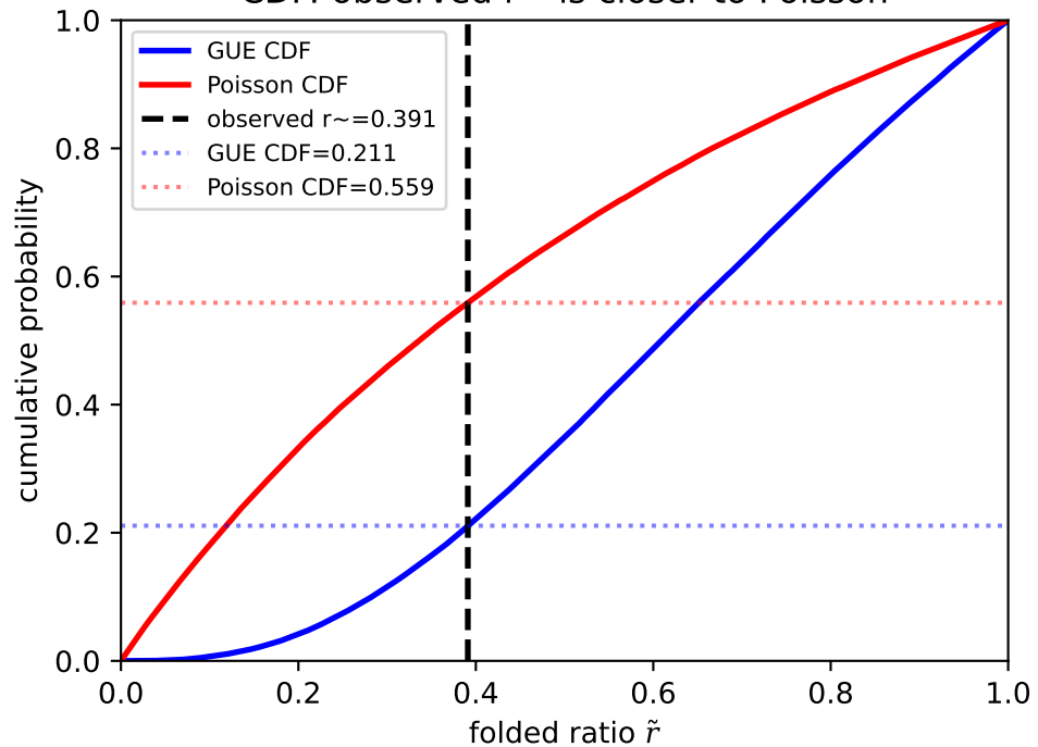
CDF: observed r\sim is closer to Poisson
