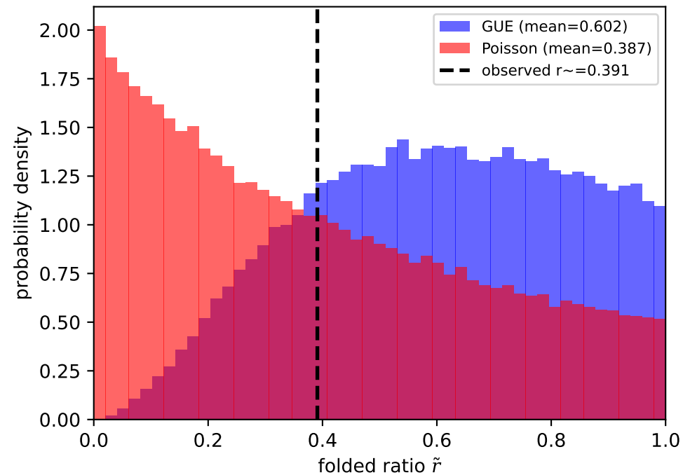
N=3: GUE vs Poisson distributions of r\sim
