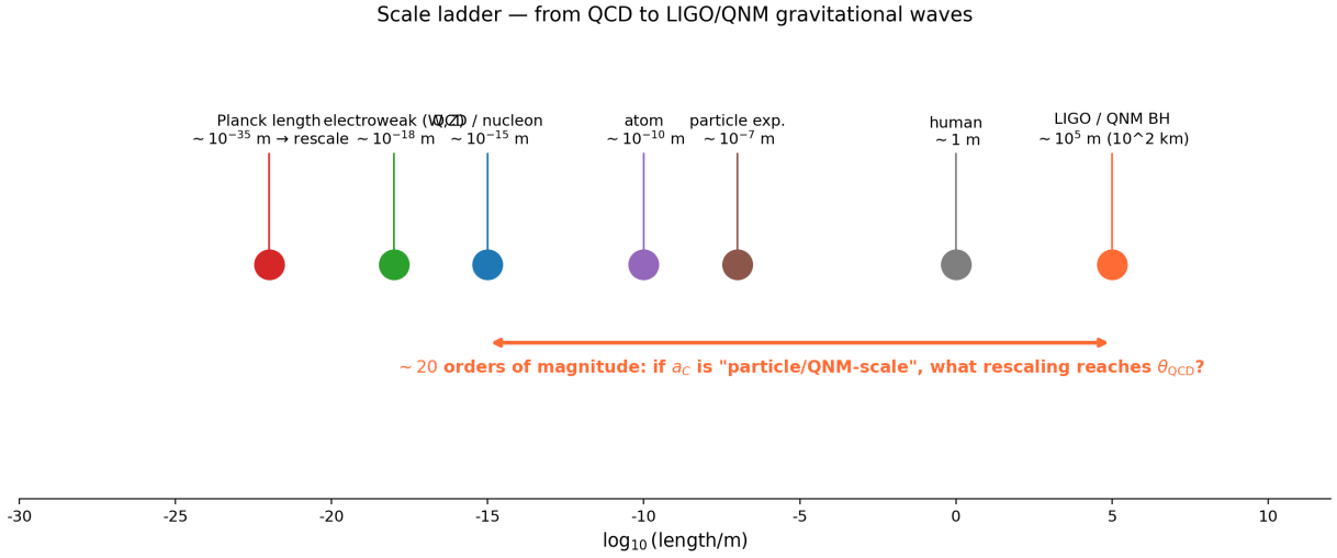
Figure 3. The \sim 20 orders of magnitude separating the QCD scale ( \sim 10^{-15} m) from the LIGO/QNM scale ( \sim 10^5 m). The user’s hypothesis: a-C acts at the latter scale and must be rescaled to reach the former. The Planck-scale rescaling (\Lambda_{\text{QCD}}/M_{\text{Pl}})^{1/3} closes the gap to within a factor of 2 of the \theta bound.
