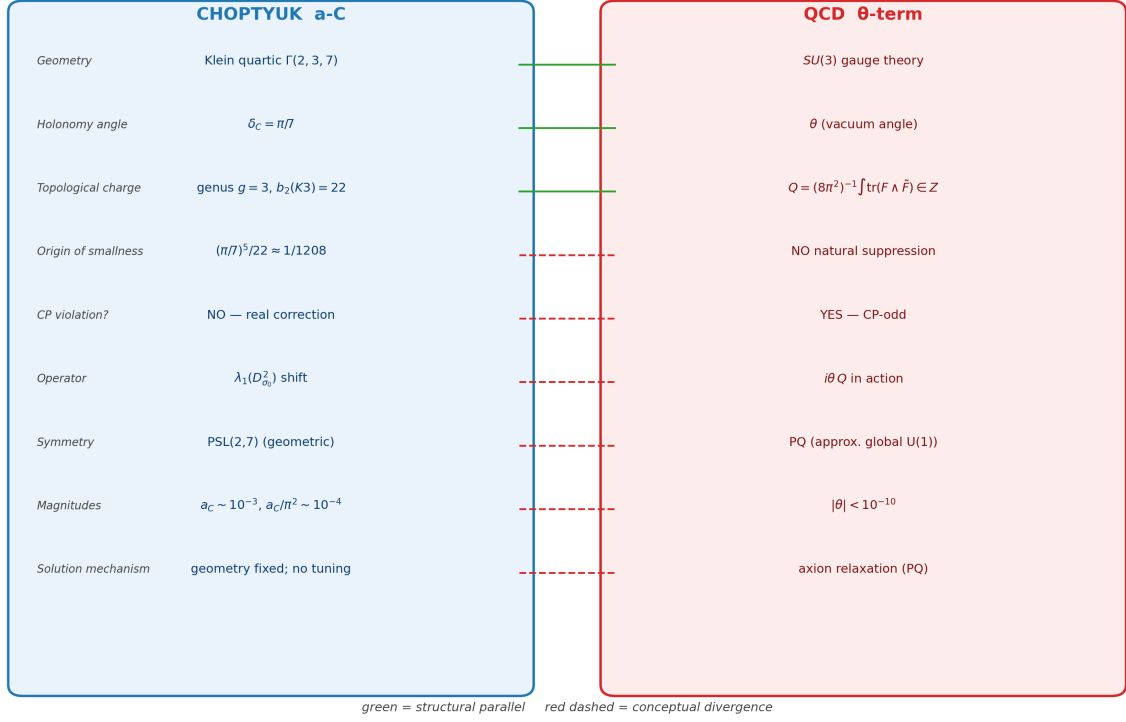
Figure 4. Structural comparison of the Choptuyuk framework (left) and the QCD \theta -term (right). Green lines mark structural parallels (geometric origin, topological charge, holonomy angle); red dashed lines mark conceptual divergences (CP properties, magnitude, solution mechanism). The bridge hypothesis seeks to convert a green line into a derivation; the current evidence does not support such a conversion.
