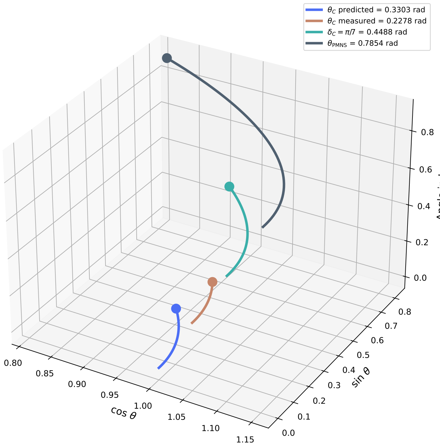
3D: Cabibbo angle predicted vs measured vs framework inputs
