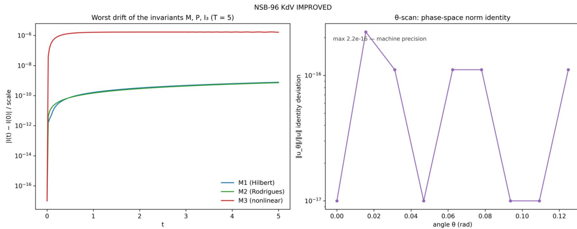
Fig. 16.78. Invariant drift and the \theta -scan of the improved scheme. Left — drift of M , P , I_3 for the M1/M2/M3 mechanisms; the DRAW of M3 is explained by the factor (1 - \cos \theta_b) \approx 1.9 \cdot 10^{-3} . Right — phase-space norm identity over 9 angles: 2.2 \cdot 10^{-16} (machine precision).
