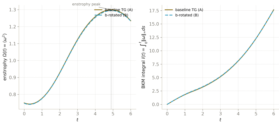
Fig. 8. P5, runs A and B: enstrophy \Omega(t) with the peak at t = 4.90 (left) and the Beale-Kato-Majda envelope I(t) (right). The two trajectories are statistically indistinguishable.
