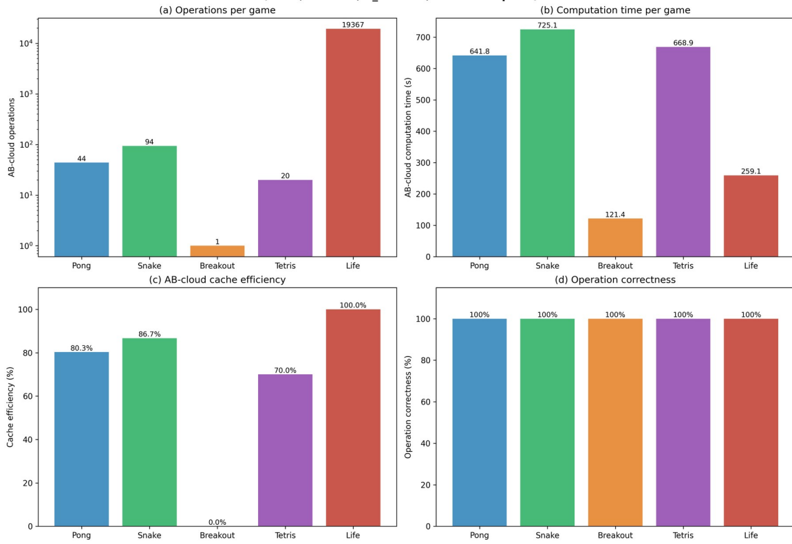
Fig. 23.1. Tournament summary: (a) operations, (b) computation time, (c) cache efficiency, (d) correctness.
