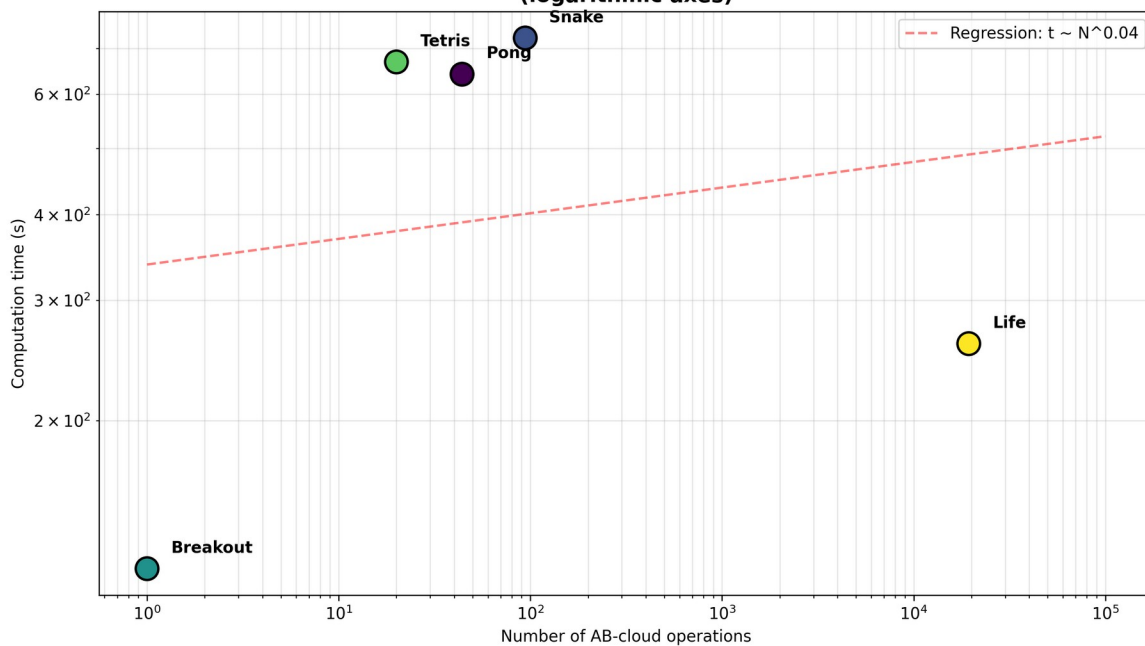
Fig. 23.6. Computation time vs number of operations (logarithmic axes).
