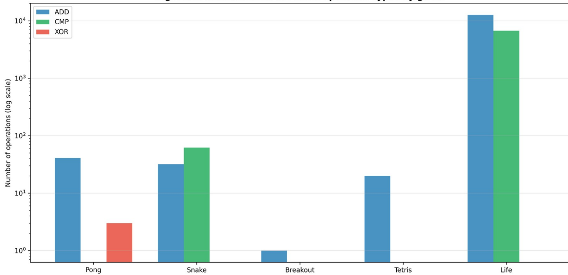
Fig. 23.2. Distribution of AB-cloud operation types by game (logarithmic scale).
