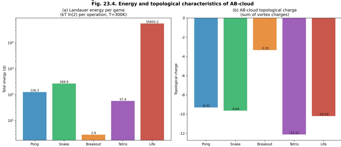
Fig. 23.4. Energy and topological characteristics of AB-cloud: (a) total Landauer energy; (b) topological charge.
