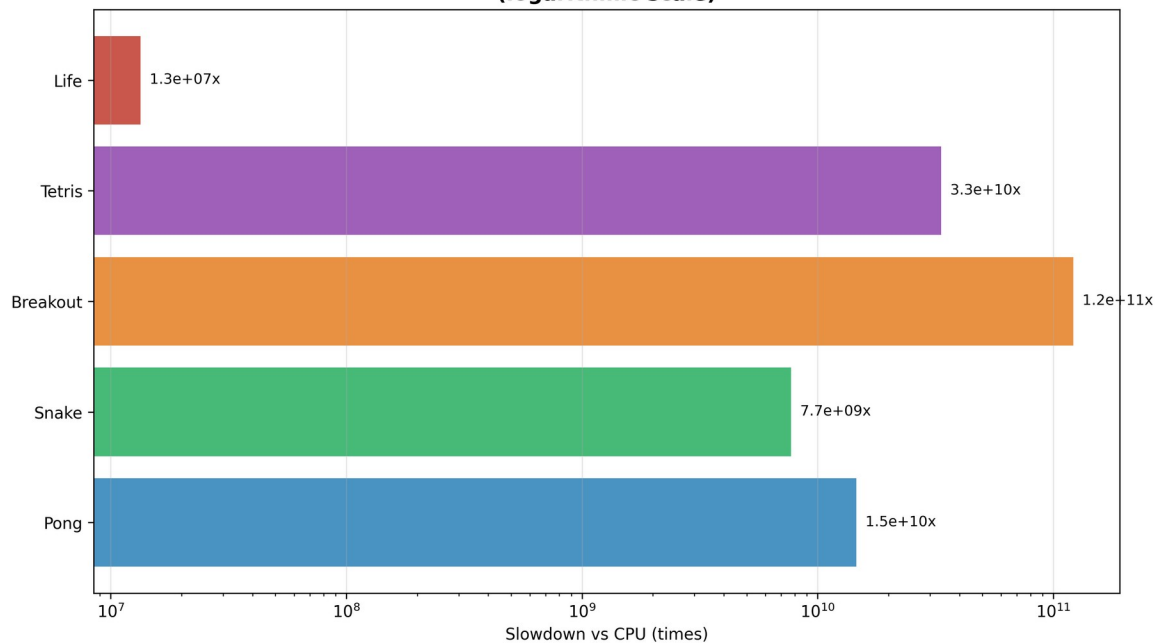
Fig. 23.3. AB-cloud slowdown relative to classical CPU (logarithmic scale).
