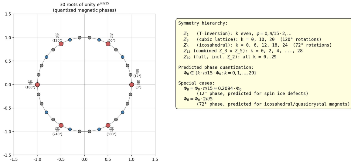
Figure E.4: Quantization of magnetic phase via \pi/15
