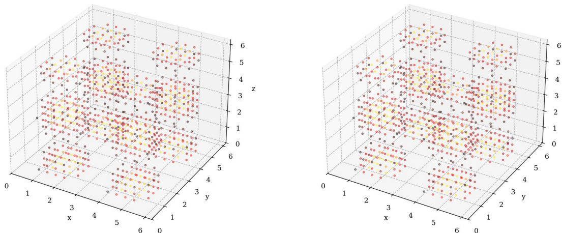
Fig. 16.74. |\omega| isosurfaces (50% of max) at t=T for true_nse (left) and b_rodrigues (right).
