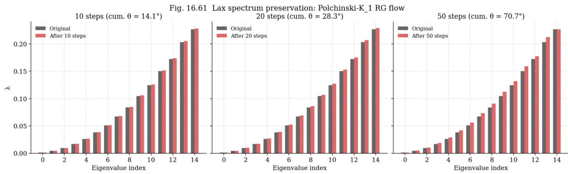
Fig. 16.61. Lax spectrum evolution under Polchinski-K 1 RG flow.
