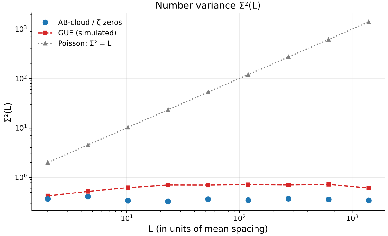
Figure 6: Fig. 6. Number variance \Sigma^2(L) : the data (flat) against logarithmic GUE and linear Poisson — closer to GUE in 9/9 points.
