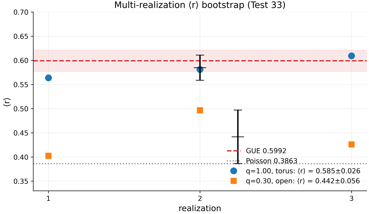
Figure 9: Fig. 9. Test 33: three \angle r \angle realizations for q = 1 (torus) and q = 0.3 (open boundaries) against the GUE and Poisson lines.
