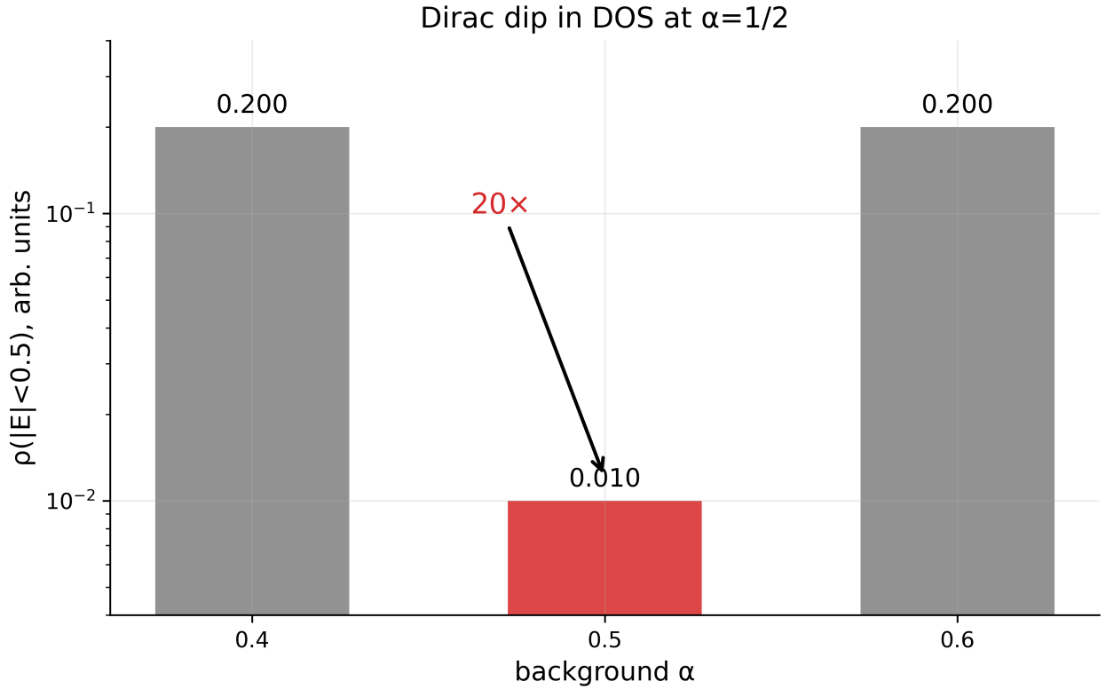
Figure 15: Fig. 15. The Dirac dip in the DOS at \alpha = 1/2 : a 20\times contrast in both directions (log scale).
