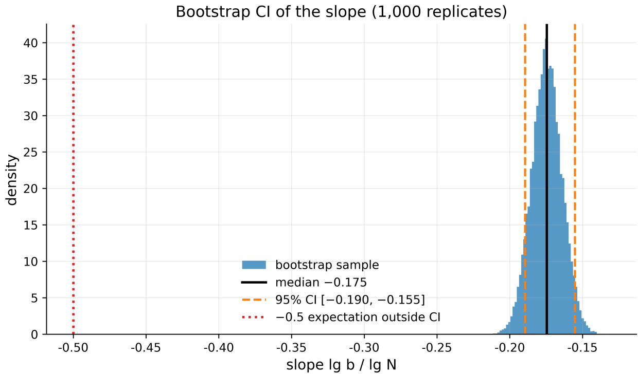
Figure 5: Fig. 5. Bootstrap distribution of the slope (1,000 replicates): the 95% CI is [-0.190; -0.155] ; the value -0.5 lies far outside.
