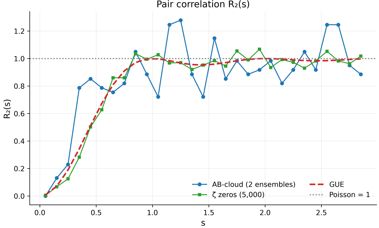
Figure 12: Fig. 12. Pair correlation R_2(s) : the AB-cloud against the \zeta zeros, GUE and Poisson — the correlation hole is reproduced by both branches.
