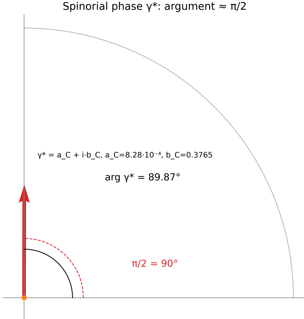
Figure 17: Fig. 17. The spinorial phase \gamma^* = a_C + ib_C : argument 89.87^\circ against the reference 90^\circ ; the dominance of b_C presses the phase to \pi/2 .
