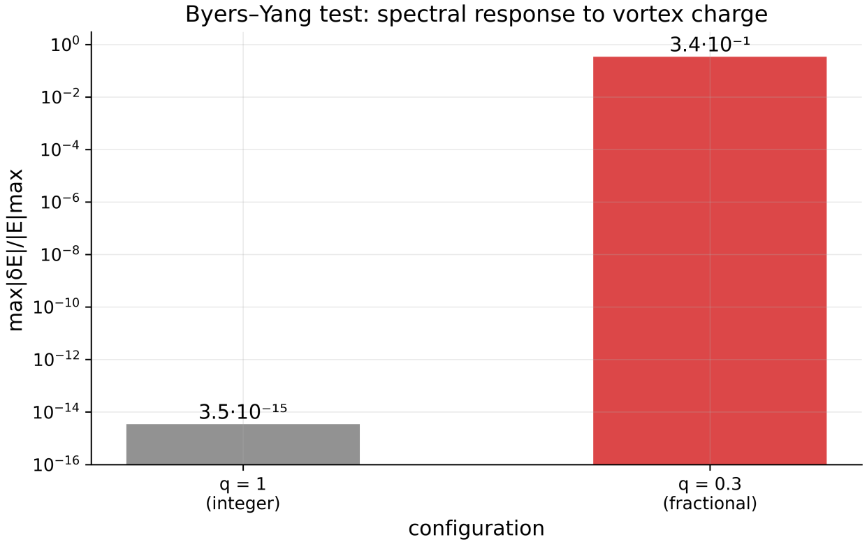
Figure 8: Fig. 8. The Byers-Yang test: integer charge is spectrally invisible ( 3.5 \cdot 10^{-15} ), fractional charge is physical (0.34); log scale.
