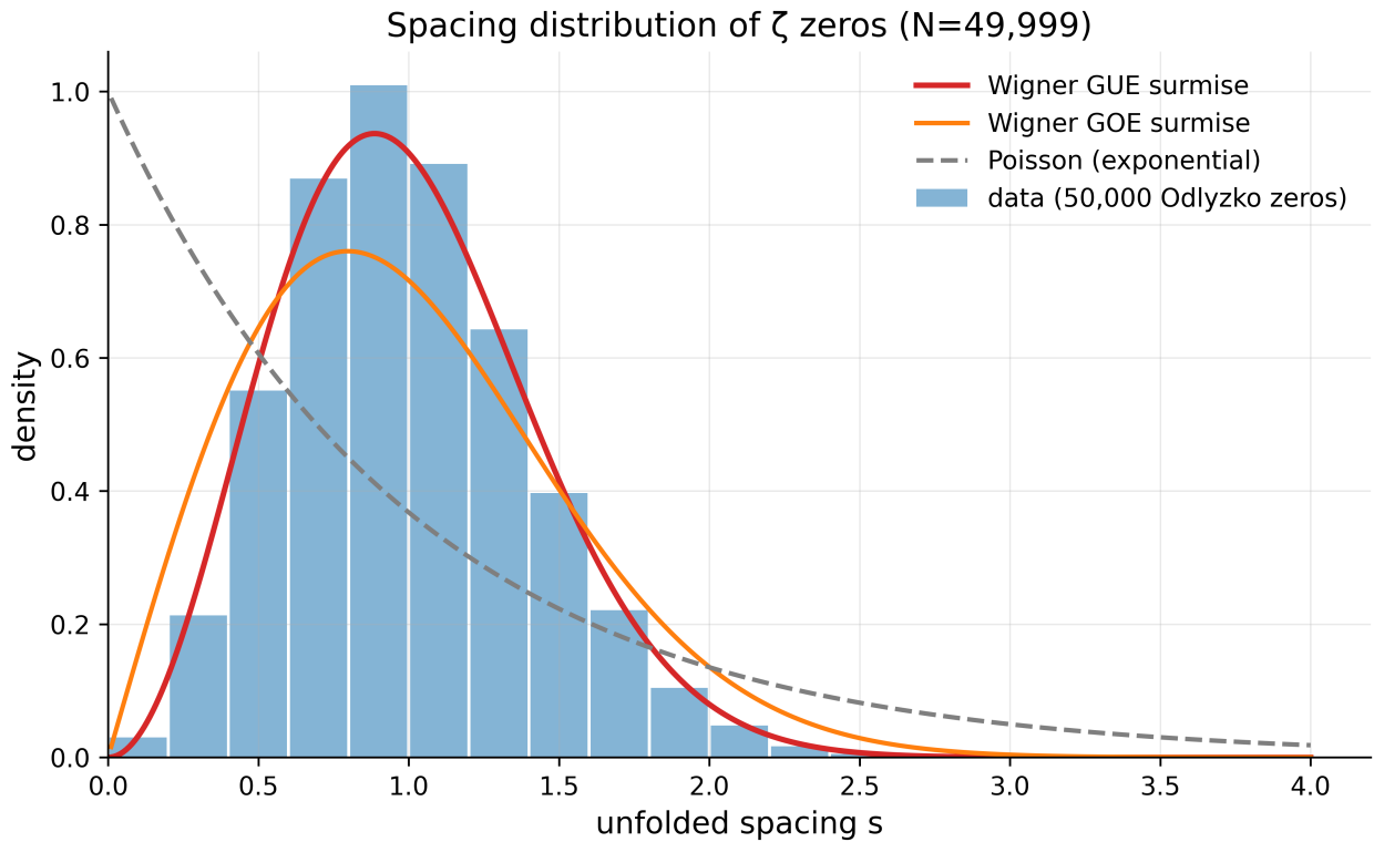
Figure 2: Fig. 2. Histogram of 49,999 \zeta -zero spacings against the Wigner surmises (GUE, GOE) and the Poisson exponential: a typically “matrix-like” shape with level repulsion.
