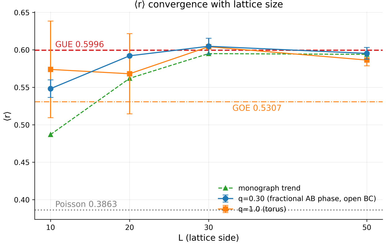
Figure 10: Fig. 10. Test 34: convergence of \langle r \rangle with lattice size; both branches settle onto the GUE plateau \approx 0.60 .
