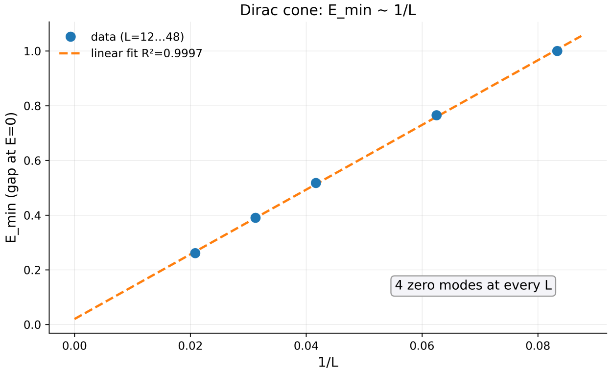
Figure 14: Fig. 14. The Dirac cone: E_{\min} = 0.02 + 11.83/L , R^2 = 0.9997 — linearity in 1/L with four zero modes at every point.
