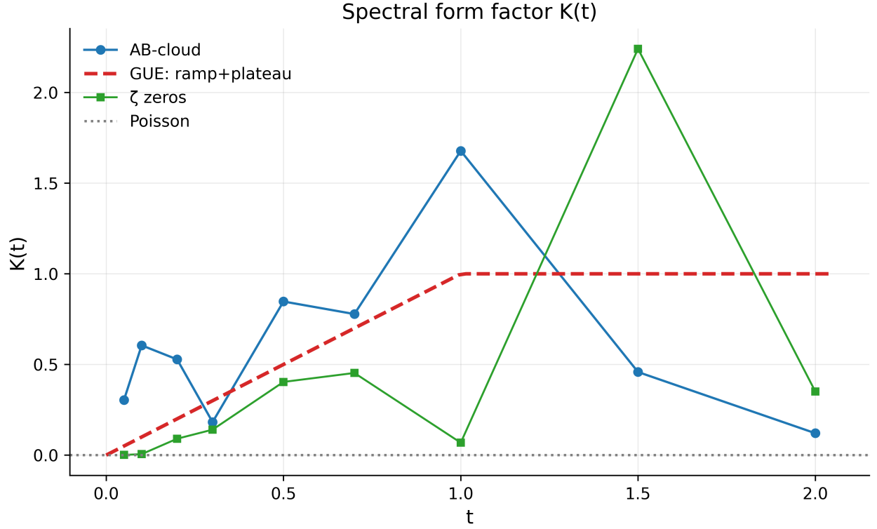
Figure 13: Fig. 13. Spectral form factor K(t) : the GUE ramp+plateau, the AB-cloud data and the \zeta zeros; small ensembles show the right trend with outliers.
