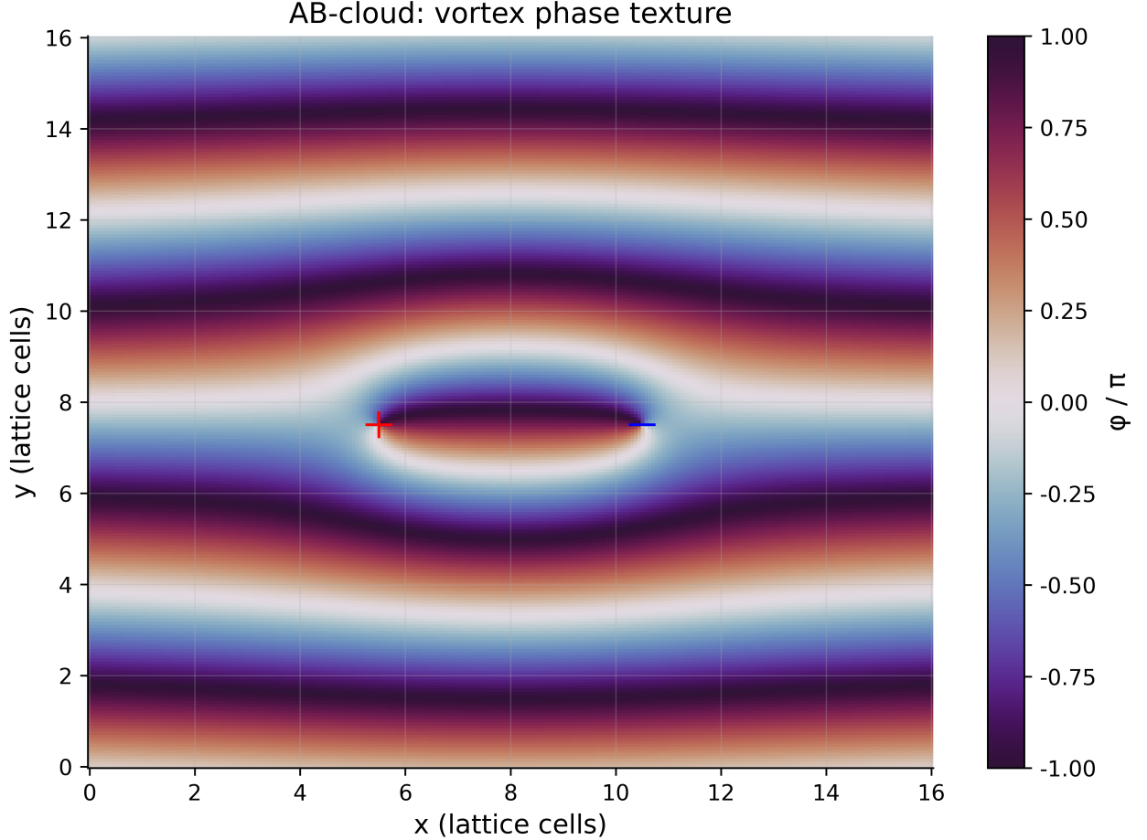
Figure 18: Fig. 18. The phase texture of a vortex pair q = \pm 1 over the Landau gauge: the phase “cloud” that generates the observed statistics.
