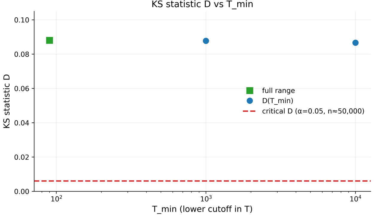
Figure 3: Fig. 3. The KS statistic D against the lower cutoff T_{\min} : a slow drift toward the critical line — the numerical expression of GUE asymptoticity.
