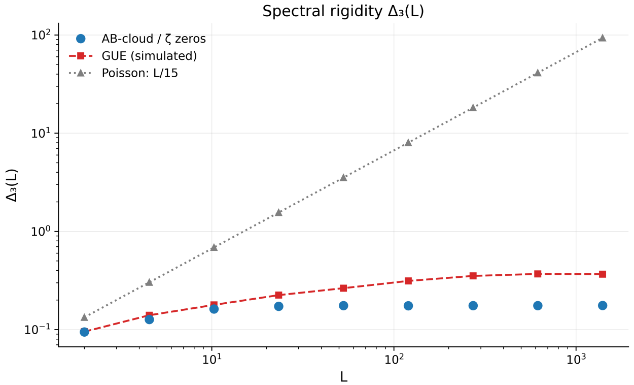
Figure 7: Fig. 7. Spectral rigidity \Delta_3(L) : super-rigidity of the data relative to even the simulated GUE at large L .
