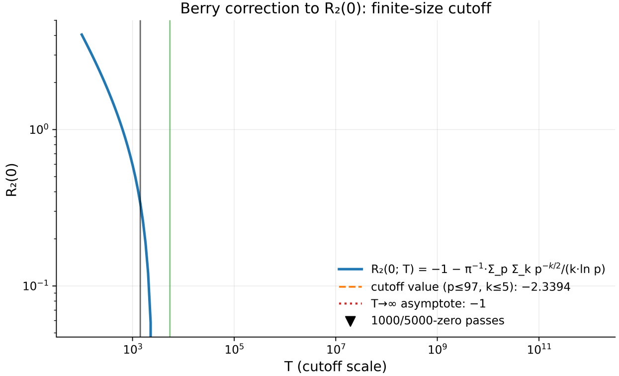
Figure 11: Fig. 11. The Berry correction R_2(0; T) : the finite-sample cutoff and the slow approach to the -1 asymptote; verticals mark the two pass heights (1000/5000 zeros).
