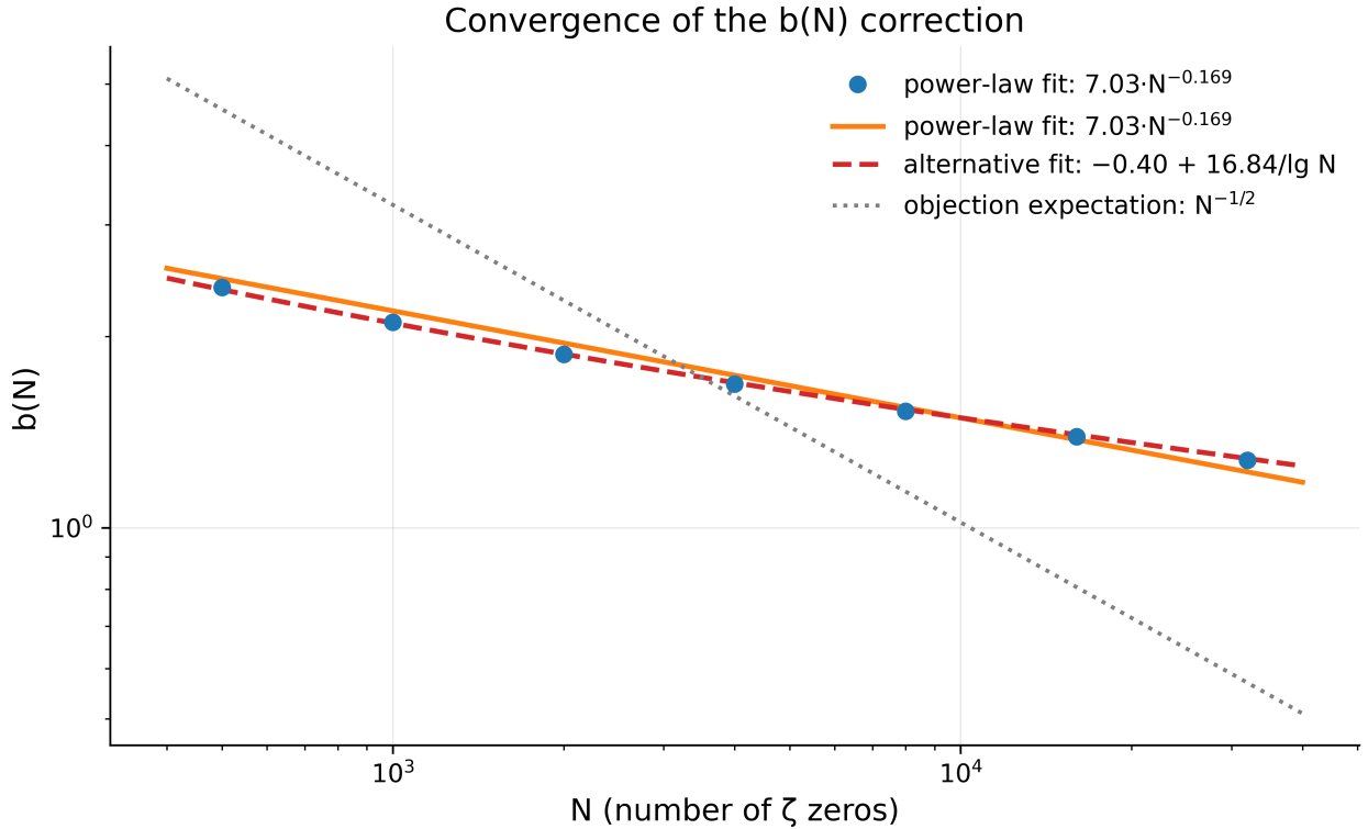
Figure 1: Fig. 1. Convergence of the b(N) correction: data and two competing fits (power law and 1/\ln N ). The critics' N^{-1/2} expectation is excluded by the data.
