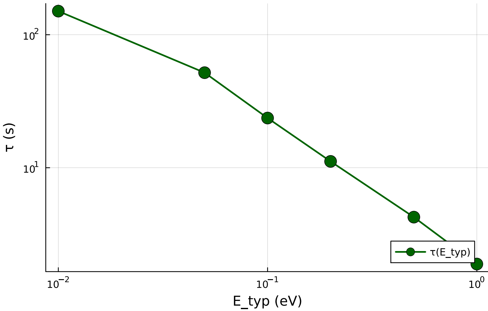
Decay time \tau = \hbar / |\text{Im } E| vs E_{\text{typ}} | slope=-0.967
