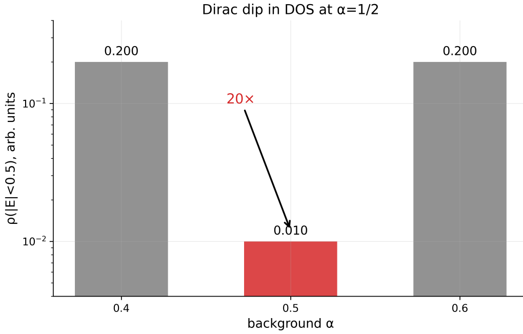
Fig. 15. The Dirac dip in the DOS at \alpha = 1/2 : a 20 \times contrast in both directions (log scale).
