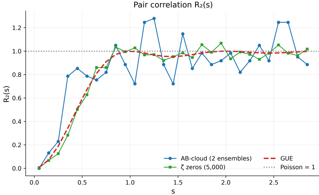
Fig. 12. Pair correlation R_2(s) : the AB-cloud against the \zeta zeros, GUE and Poisson — the correlation hole is reproduced by both branches.
