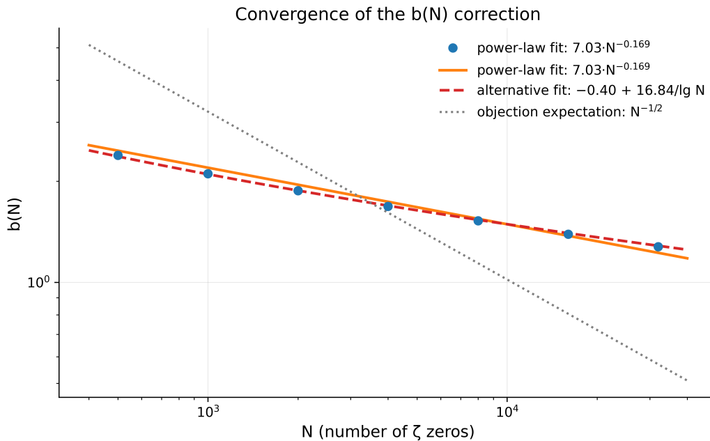
Fig. 1. Convergence of the b(N) correction: data and two competing fits (power law and 1/\ln N ). The critics' N^{-1/2} expectation is excluded by the data.
