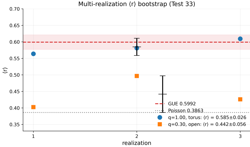
Fig. 9. Test 33: three \langle r \rangle realizations for q = 1 (torus) and q = 0.3 (open boundaries) against the GUE and Poisson lines.
