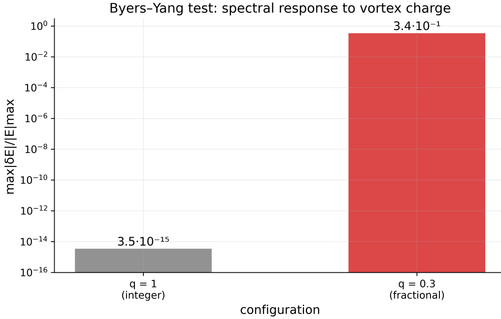
Fig. 8. The Byers–Yang test: integer charge is spectrally invisible ( 3.5 \cdot 10^{-15} ), fractional charge is physical (0.34); log scale.
