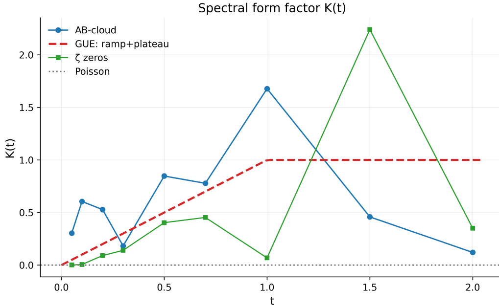
Fig. 13. Spectral form factor K(t) : the GUE ramp+plateau, the AB-cloud data and the \zeta zeros; small ensembles show the right trend with outliers.
