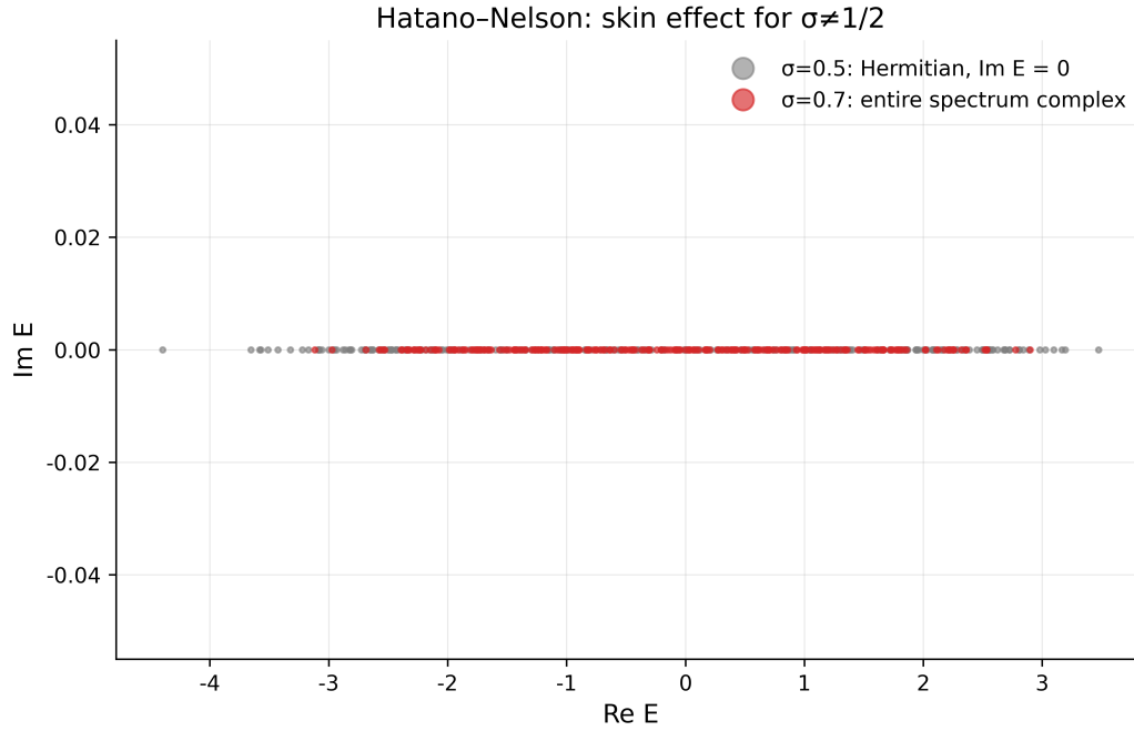
Fig. 16. Hatano–Nelson: \sigma = 0.5 — real spectrum; \sigma = 0.7 — the entire spectrum in the complex plane (skin effect).
