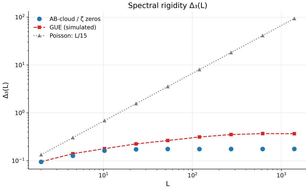
Fig. 7. Spectral rigidity \Delta_3(L) : super-rigidity of the data relative to even the simulated GUE at large L .
