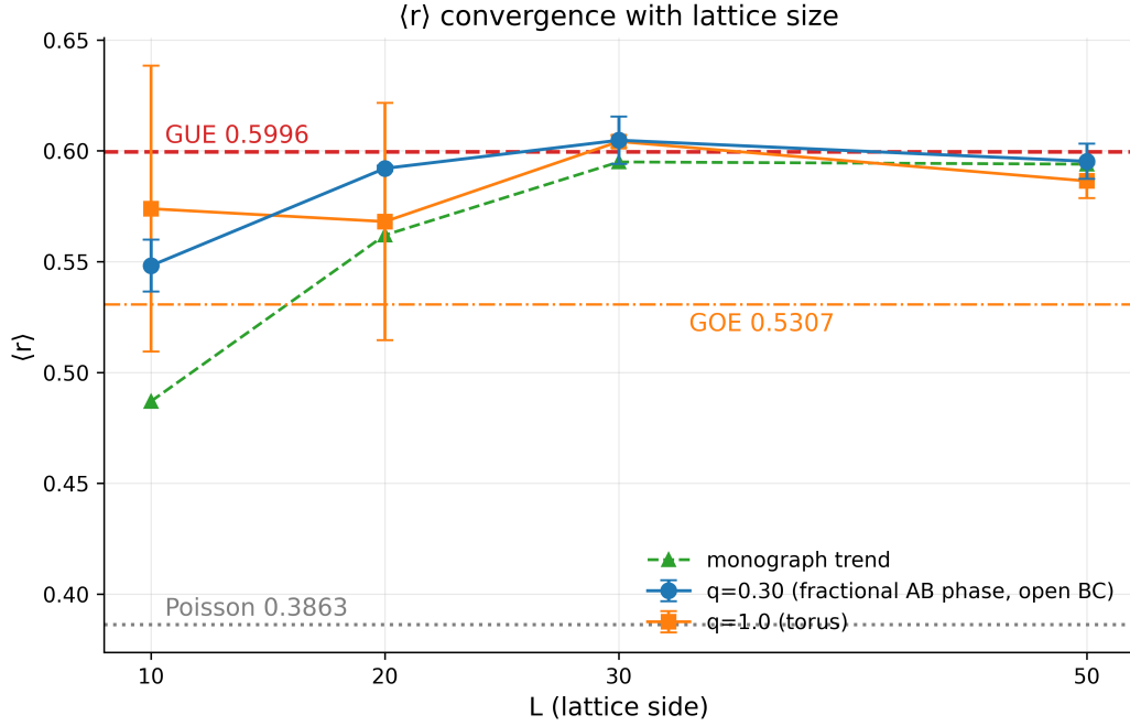
Fig. 10. Test 34: convergence of \langle r \rangle with lattice size; both branches settle onto the GUE plateau \approx 0.60 .
