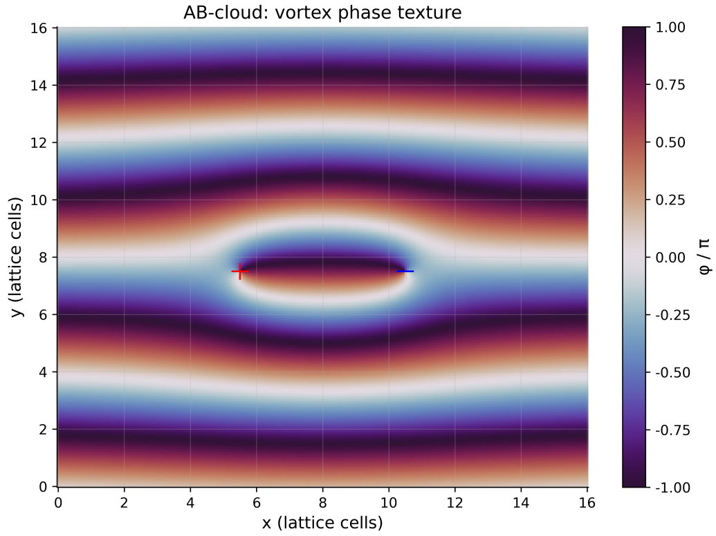
Fig. 18. The phase texture of a vortex pair q = \pm 1 over the Landau gauge: the phase “cloud” that generates the observed statistics.
