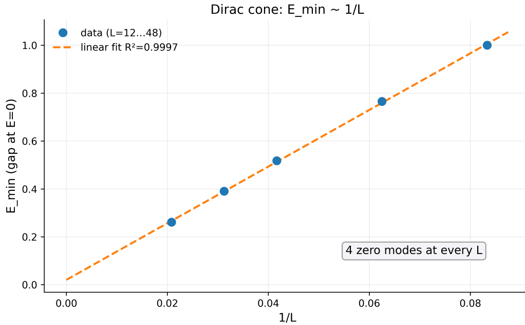
Fig. 14. The Dirac cone: E_{\min} = 0.02 + 11.83/L , R^2 = 0.9997 — linearity in 1/L with four zero modes at every point.
