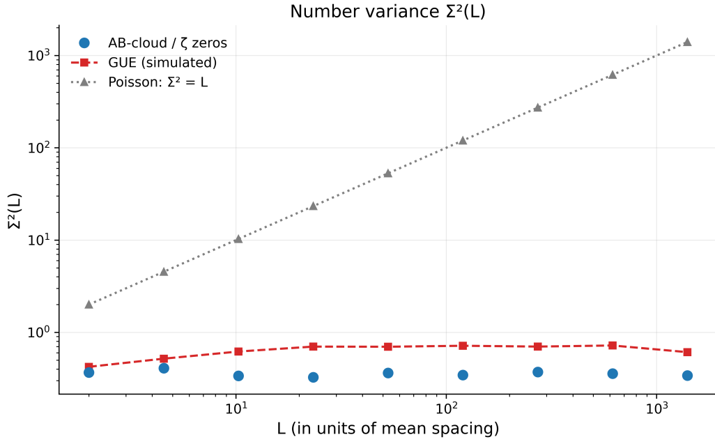
Fig. 6. Number variance \Sigma^2(L) : the data (flat) against logarithmic GUE and linear Poisson — closer to GUE in 9/9 points.
