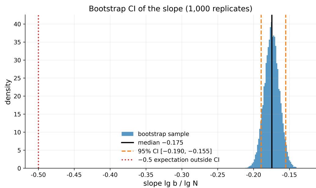
Fig. 5. Bootstrap distribution of the slope (1,000 replicates): the 95% CI is [-0.190; -0.155] ; the value -0.5 lies far outside.
