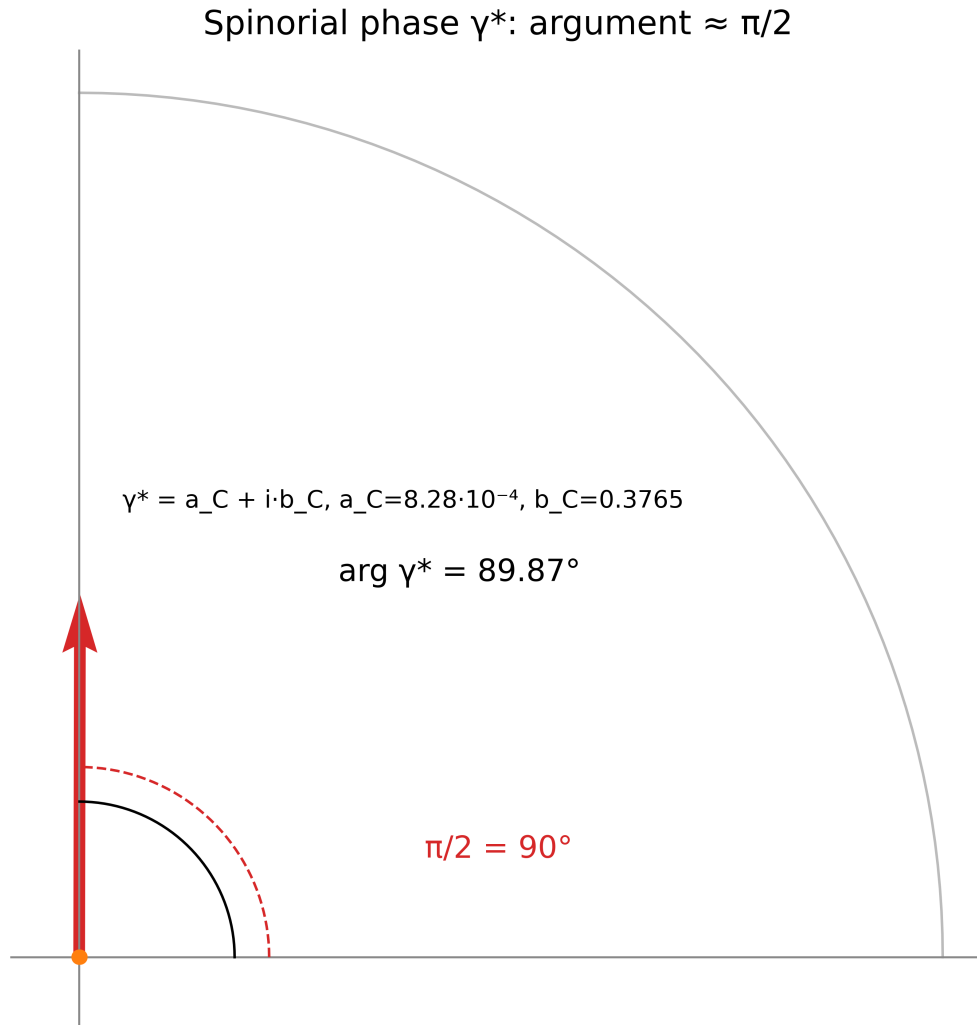
Fig. 17. The spinorial phase \gamma^* = a_C + ib_C : argument 89.87^\circ against the reference 90^\circ ; the dominance of b_C presses the phase to \pi/2 .
