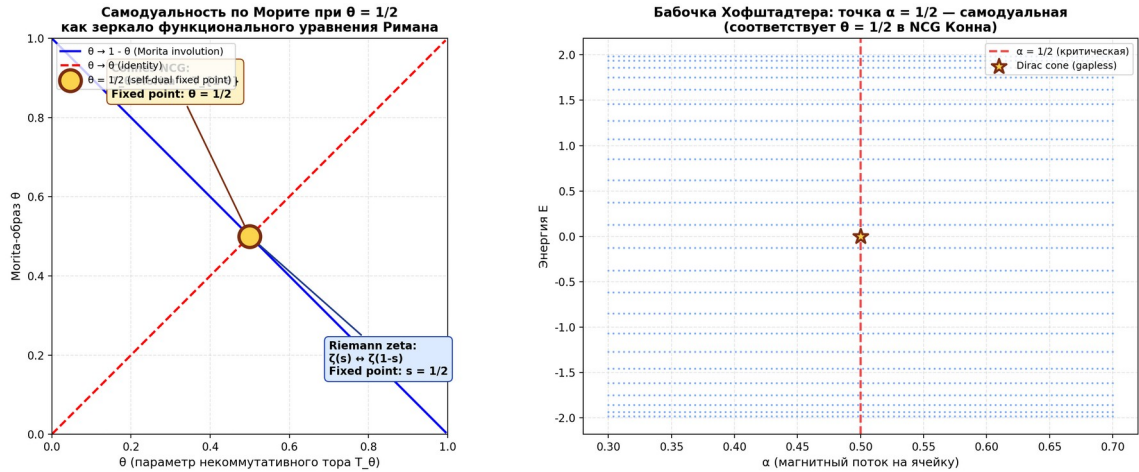
Fig. 6.3. Left: Morita involution \theta \rightarrow 1-\theta with fixed point \theta = 1/2 (self-duality of T_{1/2} ), parallel to the involution s \rightarrow 1-s with fixed point s = 1/2 (Riemann functional equation). Right: Hofstadter butterfly; the point \alpha = 1/2 is self-dual (Dirac cone without a gap).
