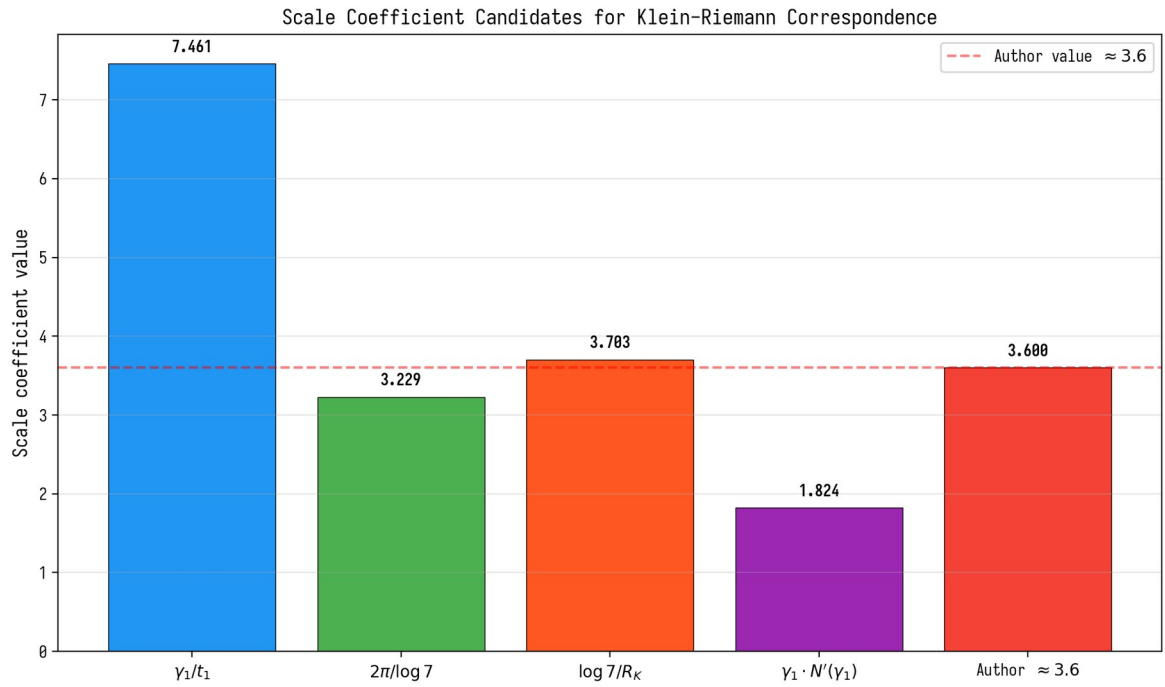
Figure 2.2. Candidates for the scaling coefficient.
