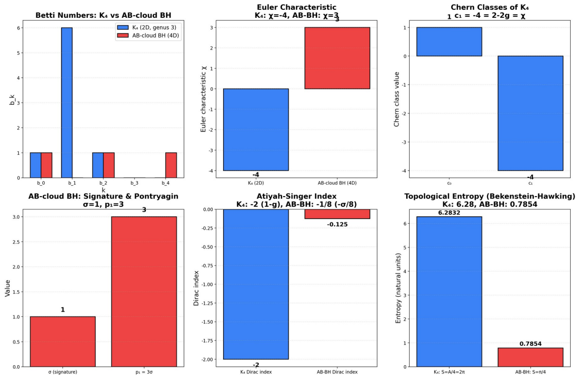
Fig. 15.1. Topological invariants: Betti numbers ( K_4 vs AB-BH), Euler characteristic, Chern and Pontryagin classes, Dirac index, topological entropy.
