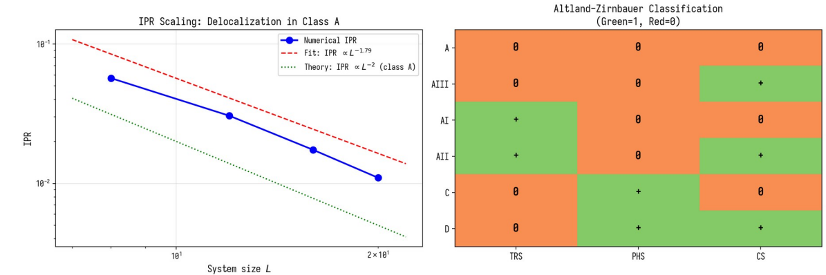
Figure 4.1. IPR-scaling and Altland-Zirnbauer classification.
