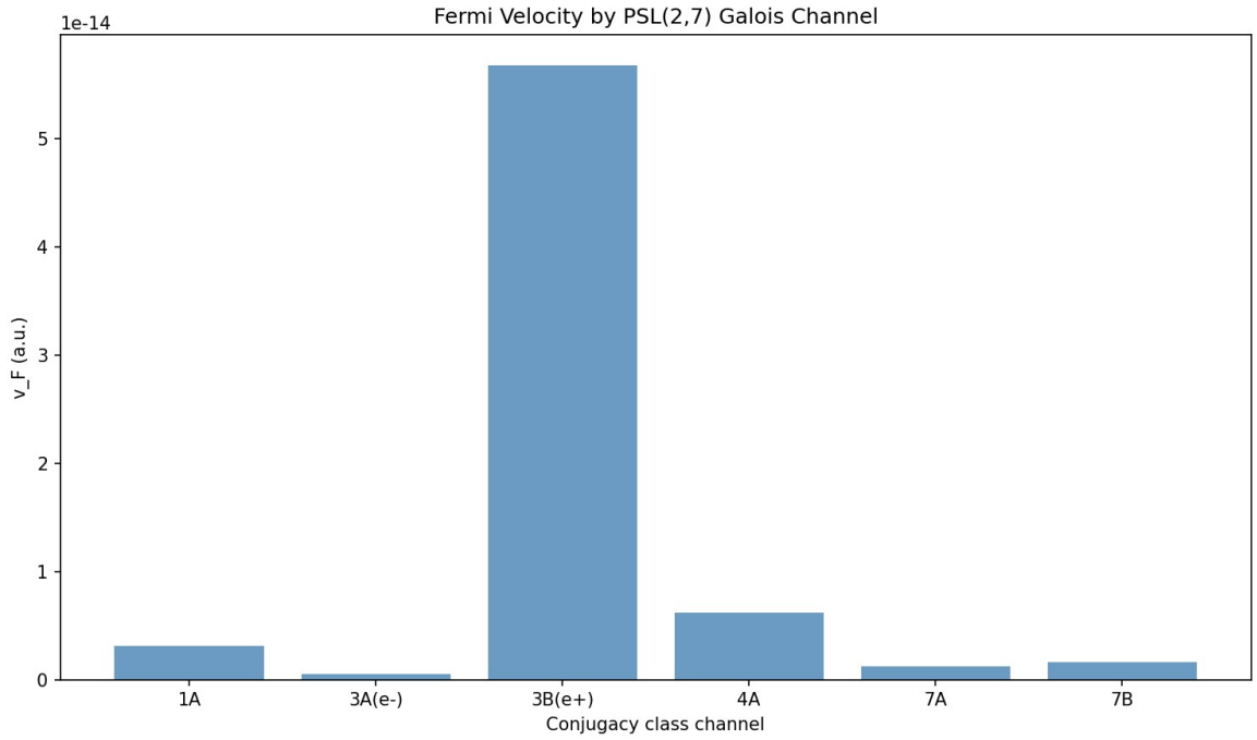
Figure 11.1. Fermi velocity across 6 Galois channels of \text{PSL}(2,7) .
