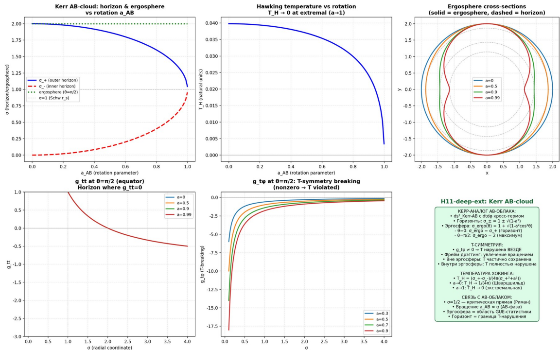
Fig. 13.3. Kerr-AB-cloud: horizons \sigma_{\pm} = 1 \pm \sqrt{1-a^2} , ergosphere \sigma_{\text{ergo}}(\theta) = 1 + \sqrt{1-a^2\cos^2\theta} , T-violation ( g_{t\phi} \neq 0 ).
