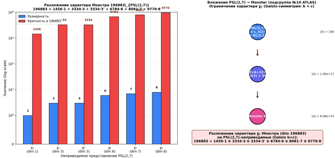
Fig. 2.6. Left: dimensions and multiplicities of the irreducible representations of \text{PSL}(2,7) in the decomposition of 196883. Right: the chain of embeddings \text{PSL}(2,7) \rightarrow 2^{\{3+6+12+18\}} \cdot (\text{L}_3(2) \times 3\text{S}_6) \rightarrow M (ATLAS subgroup №10). The restriction of the character \chi_2 (dim 196883) to \text{PSL}(2,7) is approximately 1456 \cdot 1 + 3334 \cdot 3 + 3334 \cdot 3' + 6784 \cdot 6 + 8081 \cdot 7 + 9770 \cdot 8 .
