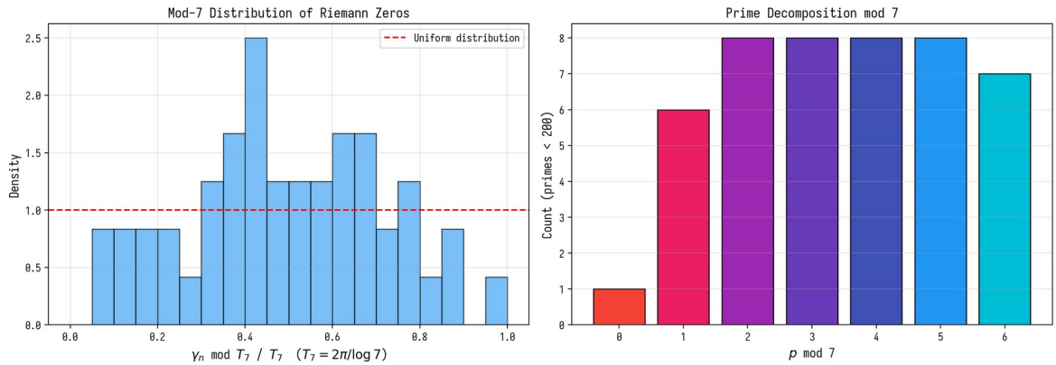
Fig. 8.2. Mod-7 distribution of Riemann zeros and prime numbers.
