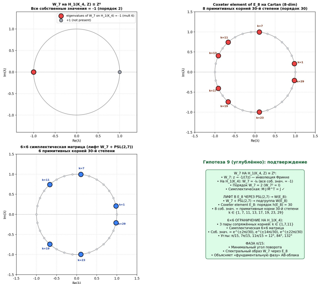
Fig. 6.5. Top left: W_7 = -I_6 on H_1(K_4, \mathbb{Z}) (all eigenvalues -1 ). Top right: 8 primitive 30th roots — eigenvalues of the E_8 Coxeter element on the Cartan. Bottom left: 6×6 restriction with 3 pairs of roots (angles 12^\circ , 84^\circ , 132^\circ ). Bottom right: summary — the phase \pi/15 as the minimal rotation angle of the W_7 lift to E_8 .
