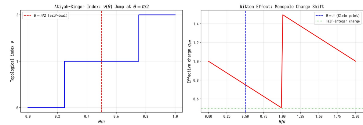
Fig. 7.1. Atiyah-Singer theorem and Witten effect.
