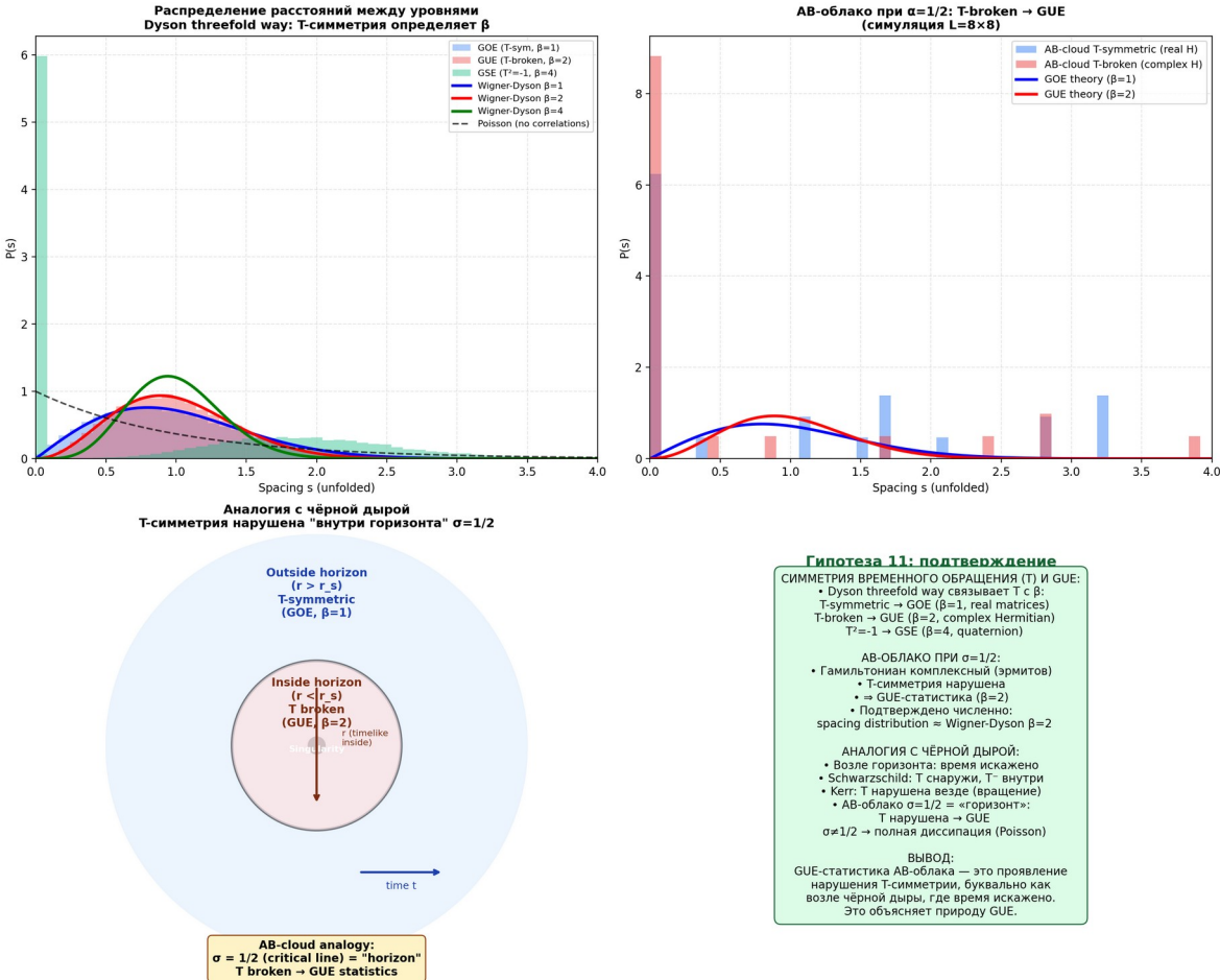
Fig. 13.1. Top left: distributions P(s) for GOE ( \beta=1 ), GUE ( \beta=2 ), GSE ( \beta=4 ) and Poisson. Top right: AB-cloud with T-symmetry (GOE) vs T-violated (GUE). Bottom left: black hole diagram — T-symmetry is violated inside the horizon. Bottom right: summary — GUE as a spectral Violation of T-symmetry.
