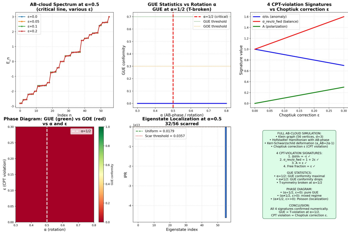
Fig. 16.1. Full AB-cloud simulation: spectra at various \varepsilon , GUE-conformity vs \alpha , 4 CPT-violation signatures, phase diagram ( \alpha vs \varepsilon ), IPR of eigenfunctions.
