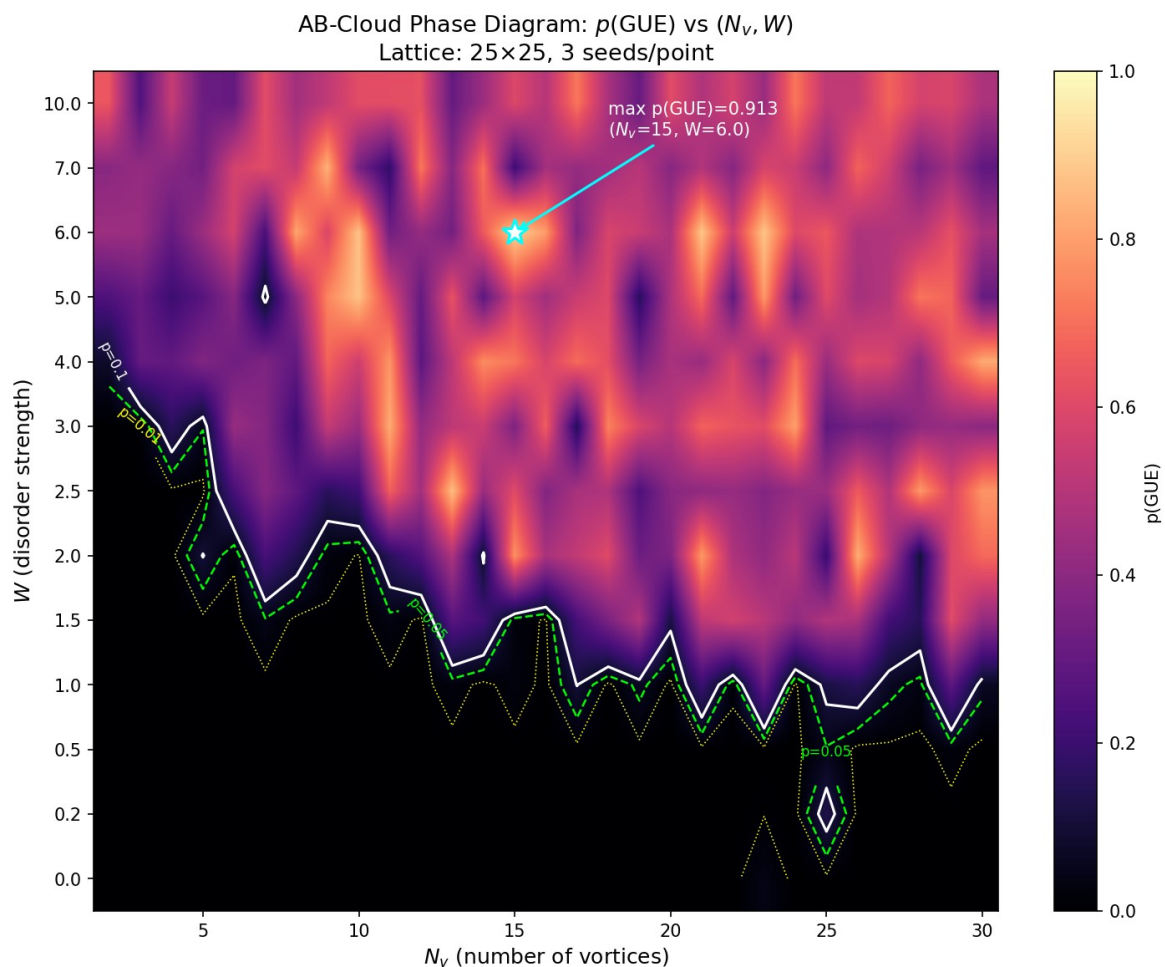
Figure 3. Phase diagram p(\text{GUE})(N_v, W) . GUE — broad plateau at W \geq 2 , N_v \geq 5 .
