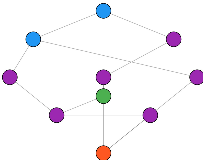
Grand Synthesis: Hidden Connections Network
