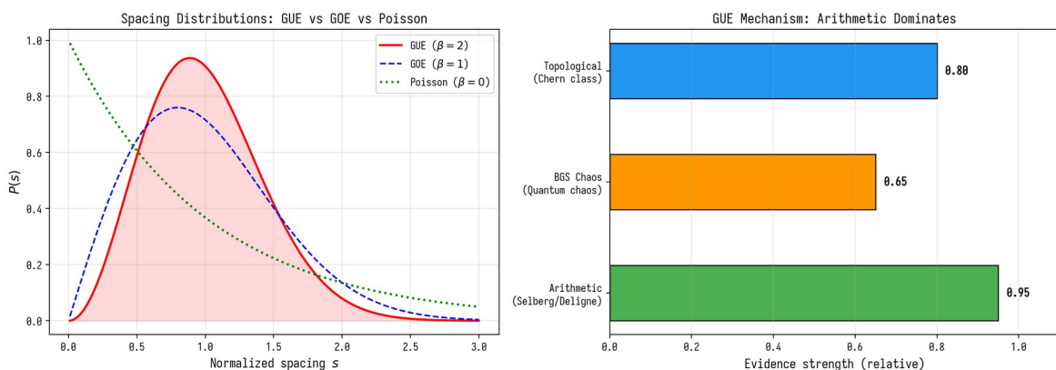
Figure 5.2. GUE mechanism: arithmetic dominance.
