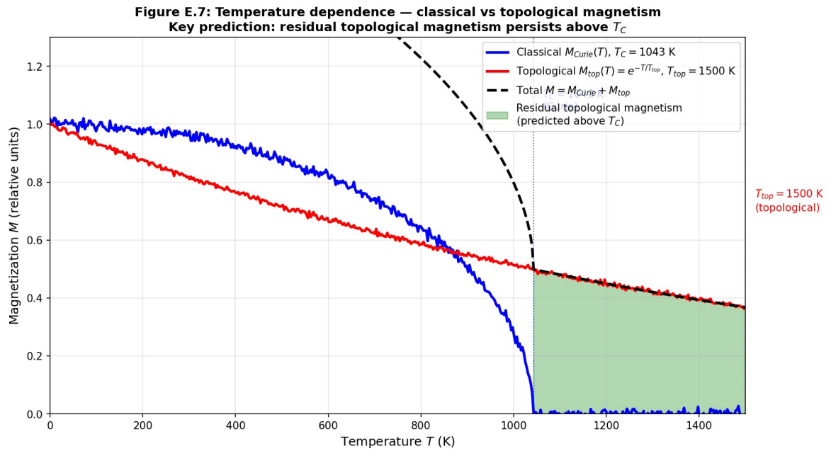
Figure E.7. Temperature dependence of magnetism: classical ( M_{\text{Curie}} , blue) and topological ( M_{\text{top}} , red) components. The green area is the "topological window" T_C < T < T_{\text{top}} , where residual topological magnetization is observed (key prediction).
