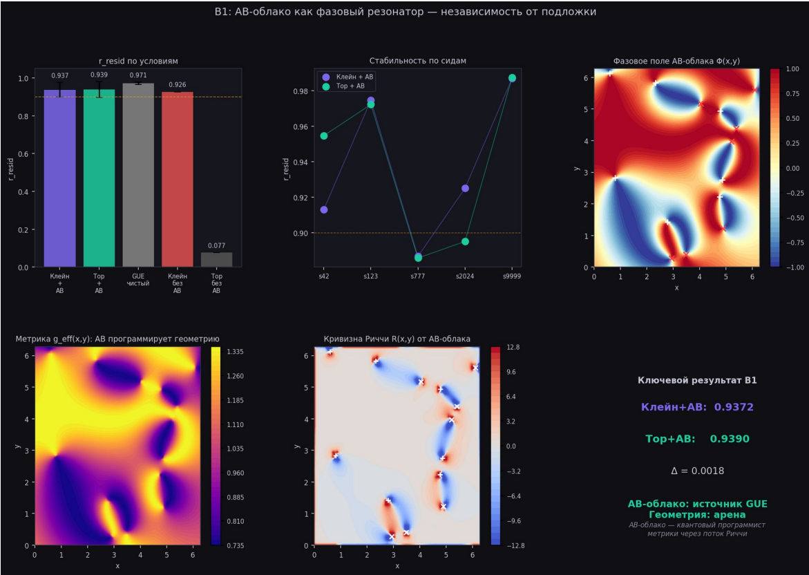
Figure 2. B1: r_{\text{resid}} for different substrates. Klein+AB \approx Torus+AB. Torus without AB = 0.077.
