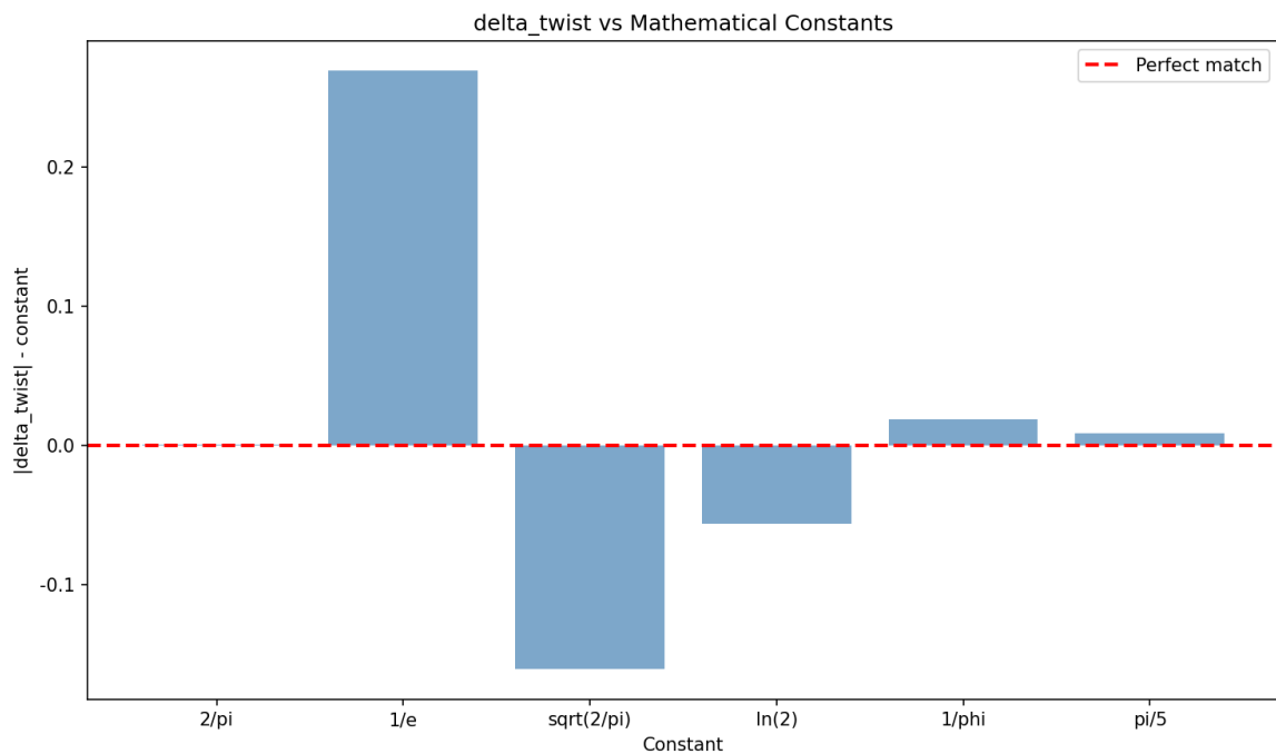
Figure 11.9. \delta_{\text{twist}} vs mathematical constants: 2/\pi — the best approximation.
