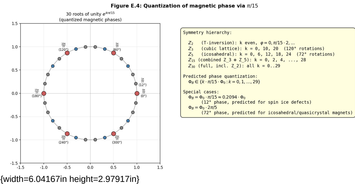
Figure E.4. Quantization of magnetic phase by \pi/15 . Left: 30 roots of 30th unity on the unit circle ( e^{ik\pi/15} , k=0..29 ), special phases Z_2 ( k even), Z_3 ( k\equiv 0 \bmod 10 ), Z_5 ( k\equiv 0 \bmod 6 ) are highlighted. Right: hierarchy of symmetries and predicted quantization of magnetic flux.
