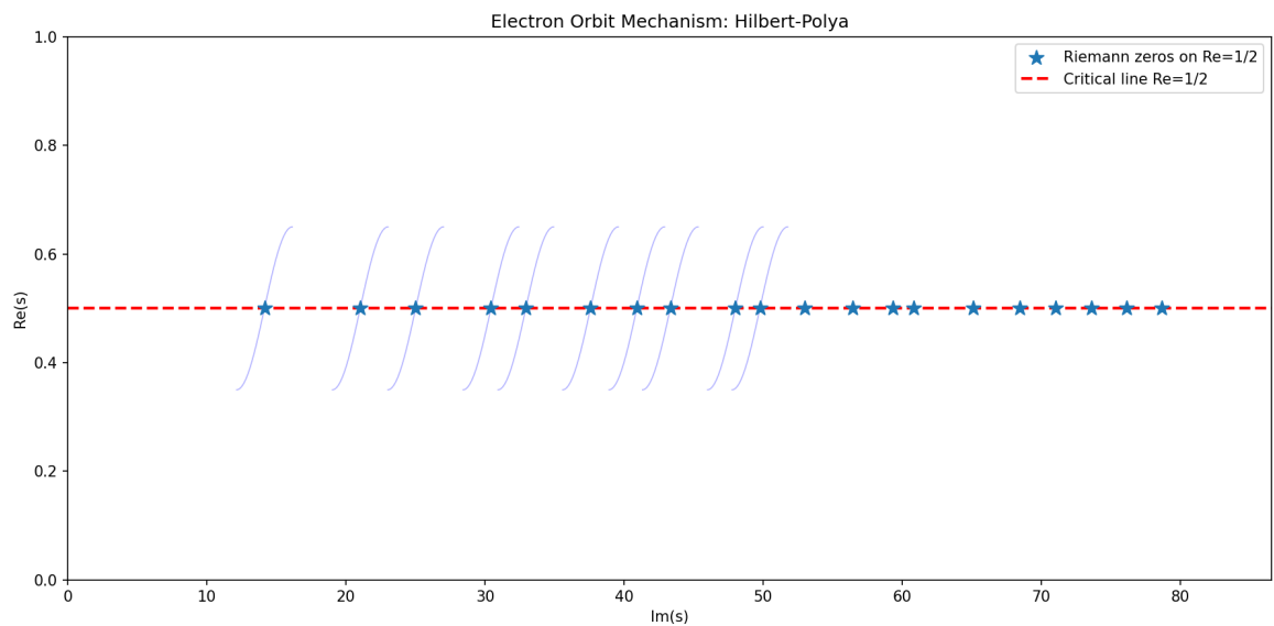
Figure 11.14. Crossings of the critical line by eigenstates vs zeros of \zeta .
