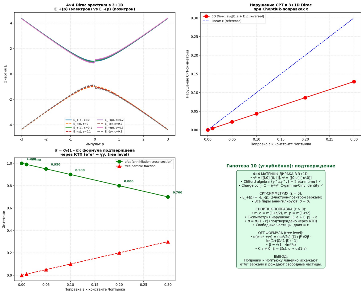
Fig. 11.14. Top left: 4x4 spectrum of Dirac in 3+1D for various \varepsilon . Top right: linear violation of CPT symmetry. Bottom left: \sigma/\sigma_0=1-\varepsilon and fraction of free particles as functions of \varepsilon . Bottom right: summary — QFT verification of the formula \sigma=\sigma_0(1-\varepsilon) .
