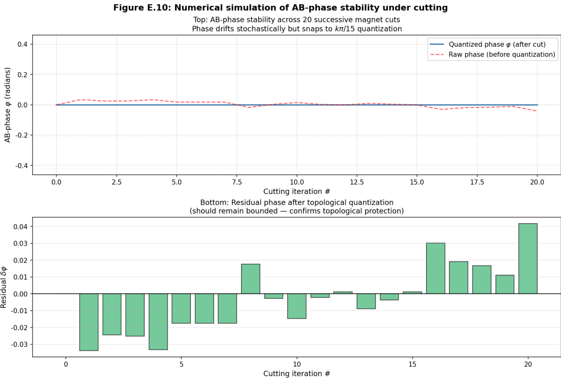
Figure E.10. Numerical simulation of AB-phase stability during 20 consecutive magnet cuttings. Top: the phase remains quantized on the k\cdot\pi/15 grid (blue stepped line), while the "raw" phase (red dashed line) drifts stochastically. Bottom: the remainder after topological quantization—remains bounded, confirming topological protection.
