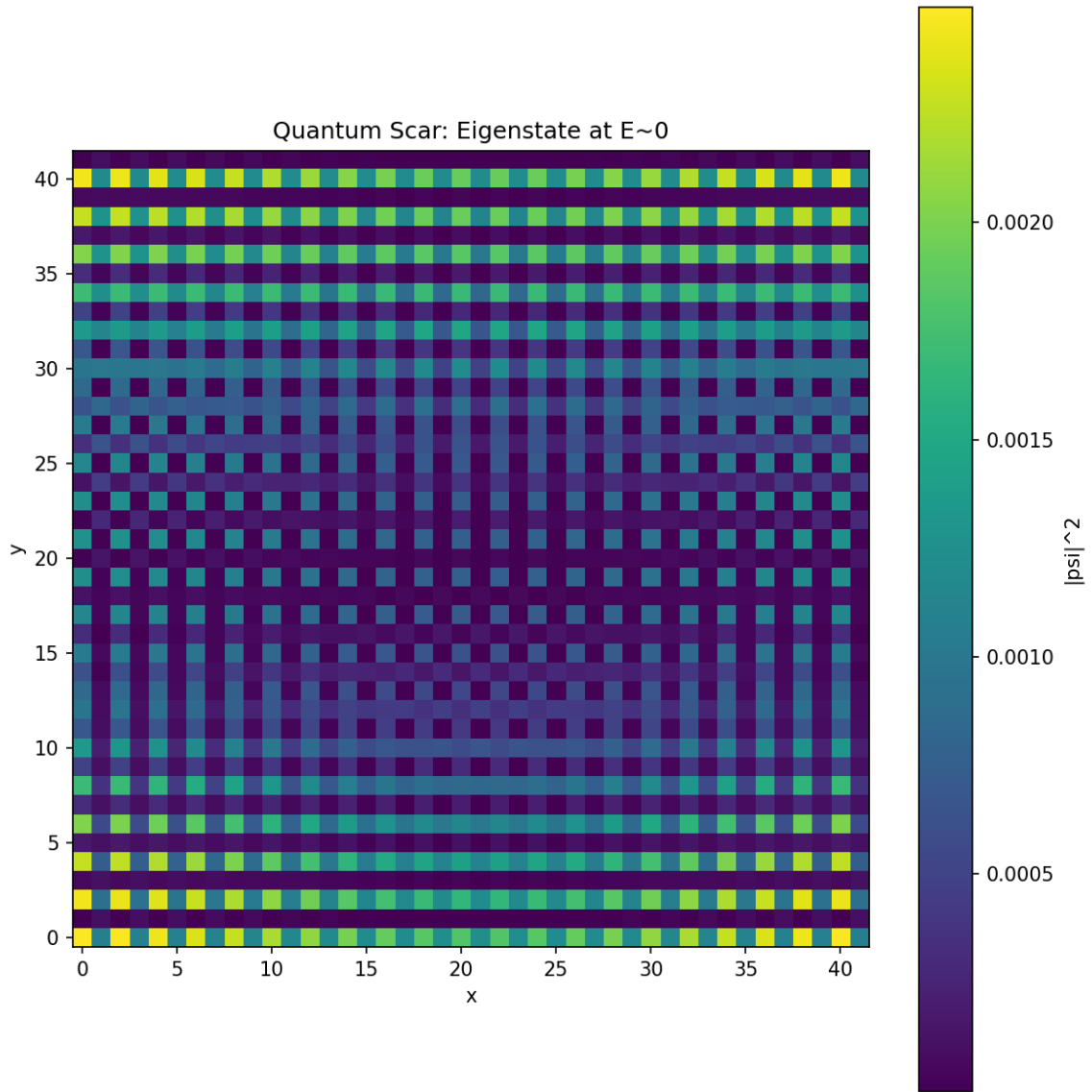
Figure 11.13. Quantum scar: eigenstate at E \approx 0 .
