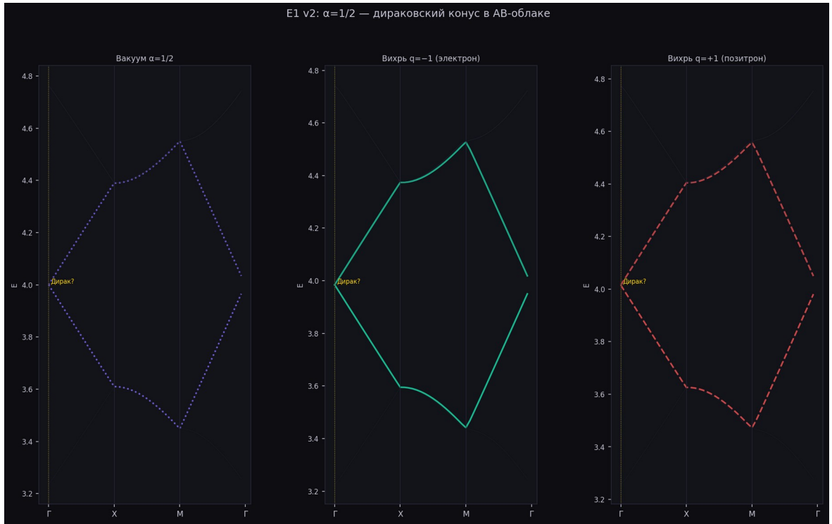
Fig. E1 v2: vortex dispersion at \alpha=1/2 . Dirac cone.
