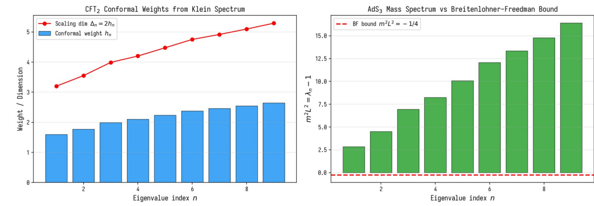
Fig. 7.2. CFT 2 conformal weights and BF-bound in AdS 3 .
