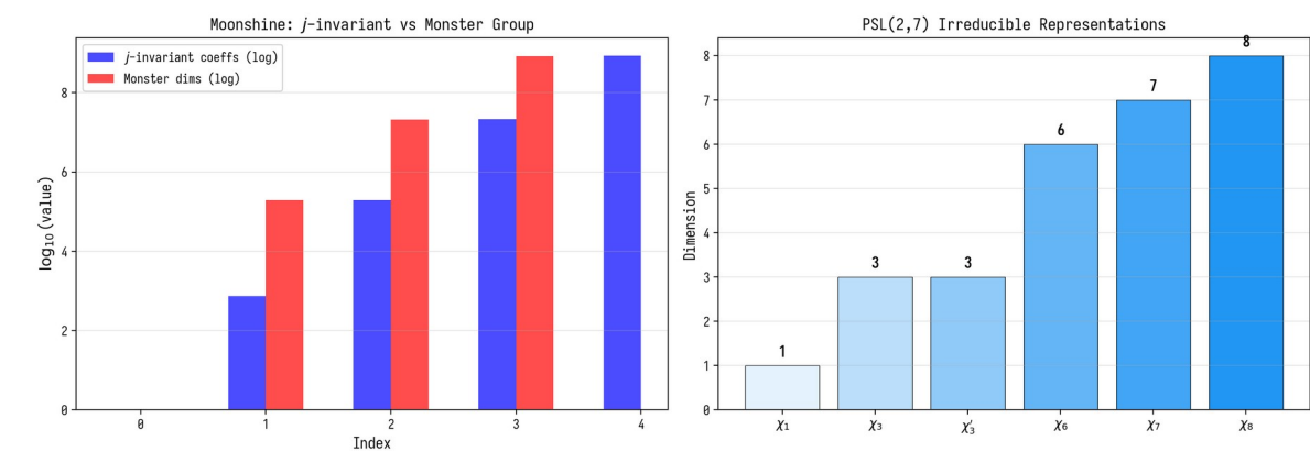
Figure 2.4. Moonshine connection: j -invariant and Monster group; representations of PSL(2,7) .
