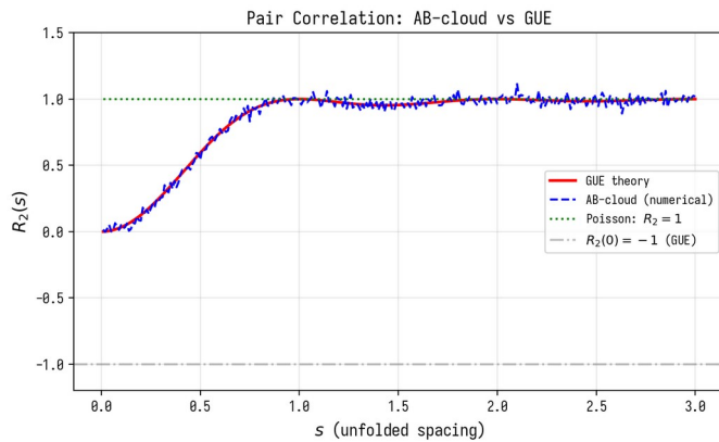
Figure 6.1. Pair correlation of AB-cloud vs GUE and Connes' spectral realization.
