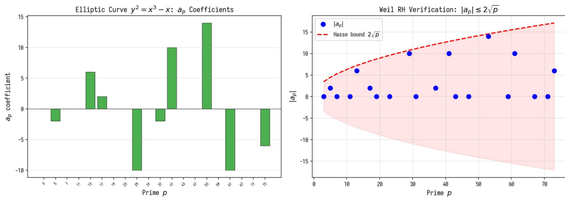
Fig. 7.3. RH for y^2=x^3-x : a_p and Hasse bound.
