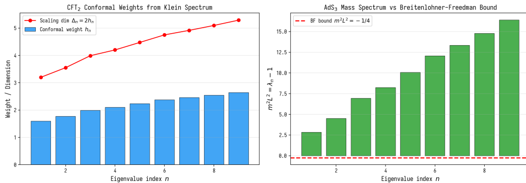
Fig. 7.2. CFT 2 conformal weights and BF-bound in AdS 3 .
