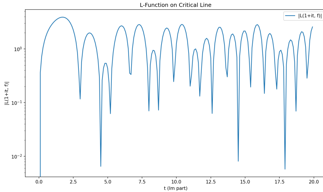
Figure 11.7. |L(1+it, f)| on the critical line: 18 zero candidates.
