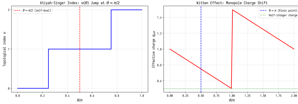
Fig. 7.1. Atiyah-Singer theorem and Witten effect.
