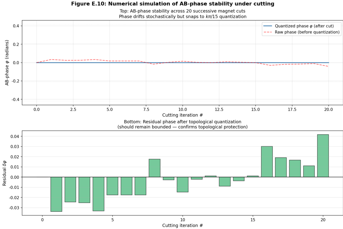
Figure E.10. Numerical simulation of AB-phase stability during 20 consecutive magnet cuttings. Top: the phase remains quantized on the k\pi/15 grid (blue stepped line), while the “raw” phase (red dashed line) drifts stochastically. Bottom: the remainder after topological quantization—remains bounded, confirming topological protection.
