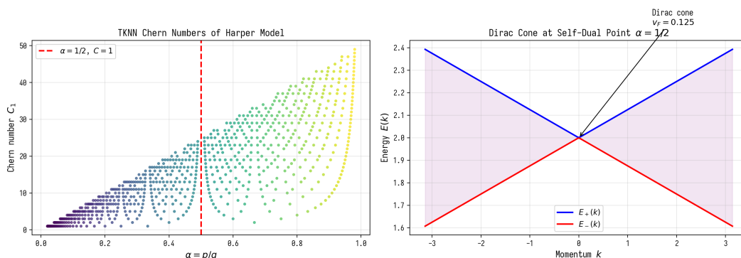
Figure 4.2. TKNN Chern numbers and Dirac cone at \alpha=1/2 .
