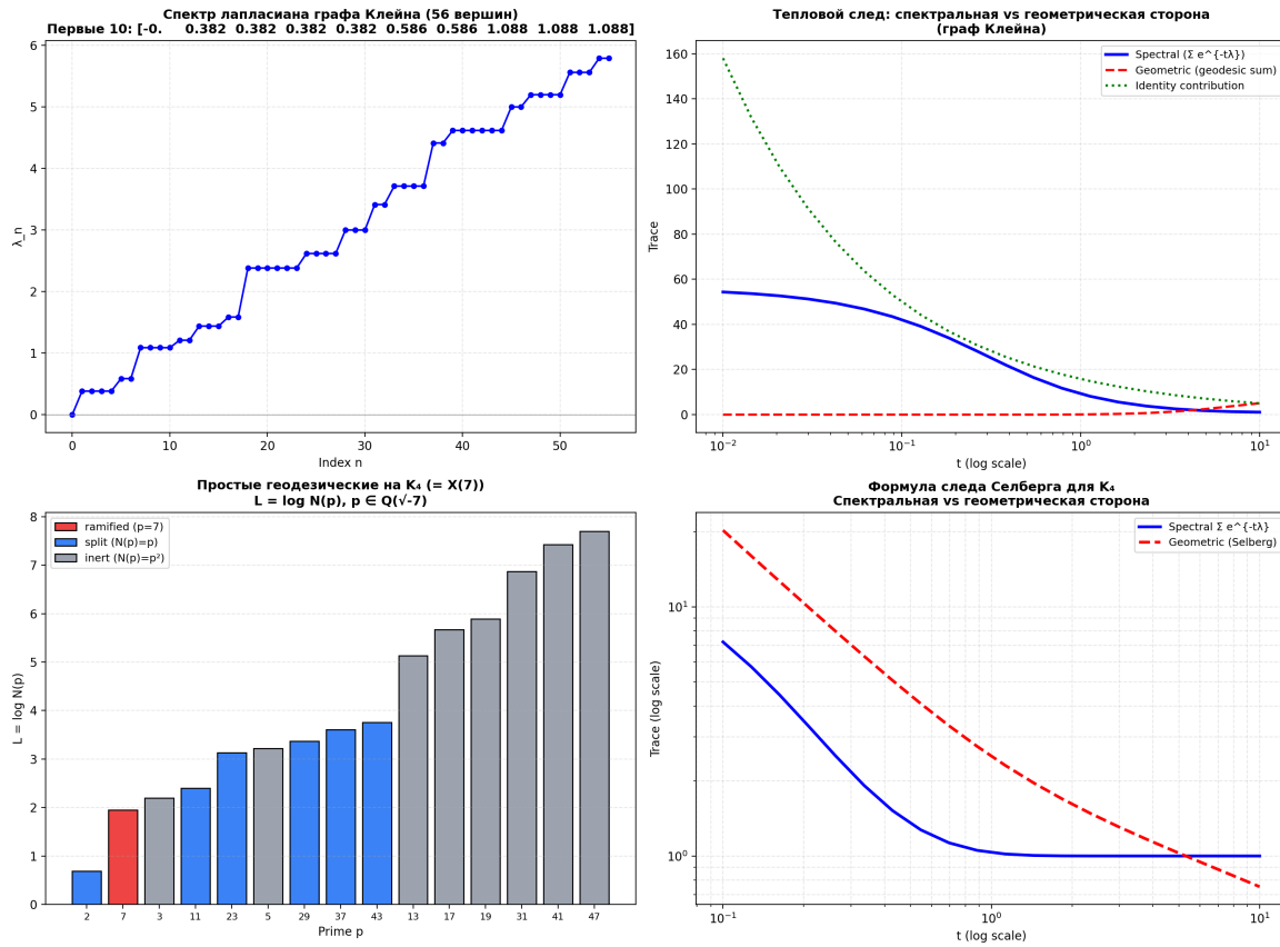
Fig. 6.6. Top left: spectrum of the Klein graph Laplacian. Top right: heat trace — spectral vs geometric side. Bottom left: prime geodesics on K_4 (ramified, split, inert). Bottom right: Selberg formula verification (log-log).
