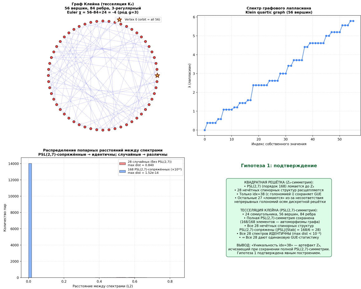
Fig. 3.4. Top left: Klein graph (56 vertices, 84 edges, 3-regular, \chi = -4 ). Top right: spectrum of the graph Laplacian. Bottom left: distribution of pairwise distances between spectra — PSL(2,7)-conjugate (blue) have distance \sim 10^{-14} , random (red) — \sim 0.84 . Bottom right: conceptual summary confirming Hypothesis 1.
