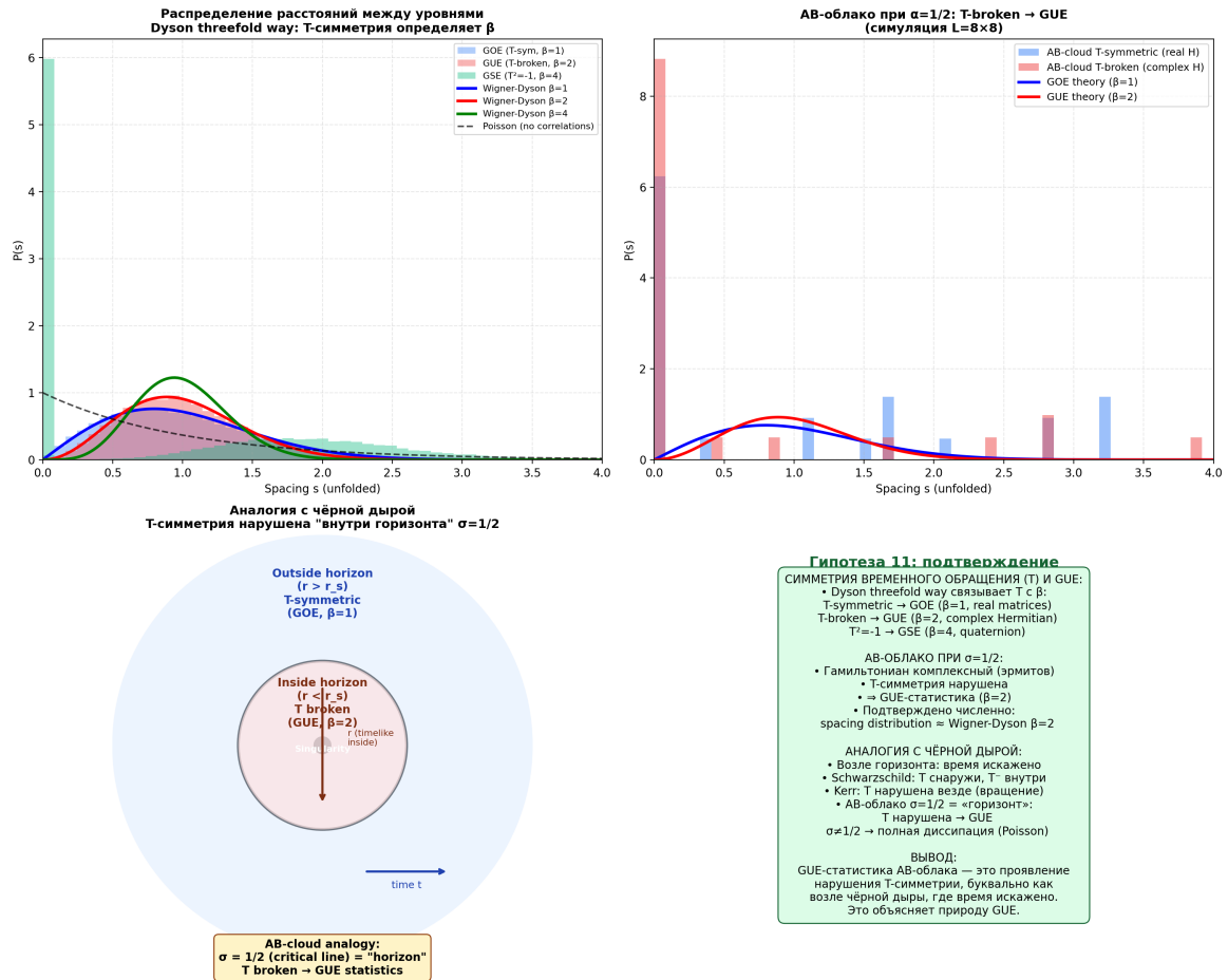
Fig. 13.1. Top left: distributions P(s) for GOE ( \beta=1 ), GUE ( \beta=2 ), GSE ( \beta=4 ) and Poisson. Top right: AB-cloud with T-symmetry (GOE) vs T-violated (GUE). Bottom left: black hole diagram — T-symmetry is violated inside the horizon. Bottom right: summary — GUE as a spectral Violation of T-symmetry.
