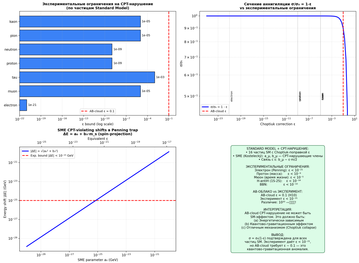
Fig. 11.15. Top left: experimental constraints \epsilon for SM particles. Top right: \sigma/\sigma_0 = 1 - \epsilon . Bottom left: SME shifts in Penning trap. Bottom right: summary — AB-cloud requires a quantum-gravitational regime.
