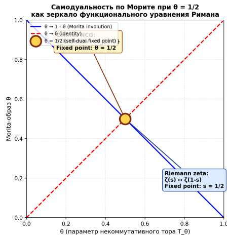
Fig. 6.3. Left: Morita involution \theta \rightarrow 1-\theta with fixed point \theta = 1/2 (self-duality of T_{\{1/2\}} ), parallel to the involution s \rightarrow 1-s with fixed point s = 1/2 (Riemann functional equation). Right: Hofstadter butterfly; the point \alpha = 1/2 is self-dual (Dirac cone without a gap).
