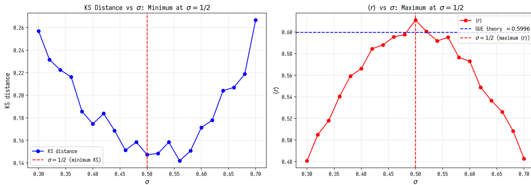
Fig. 6.3. KS and r_{\text{mean}} vs \sigma : optimum at \sigma=1/2 .
