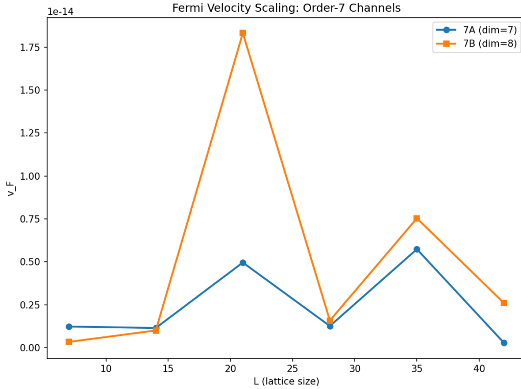
Figure 11.2. Scaling of Fermi velocity for order-7 channels (7A dim=7, 7B dim=8).
