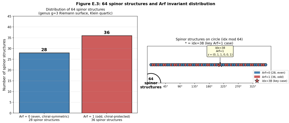
Figure E.3. Distribution of 64 spinor structures on the Klein quartic by Arf-invariant. Left: 28 even ( \text{Arf}=0 , blue) and 36 odd ( \text{Arf}=1 , red). Right: arrangement on the circle \text{idx mod } 64 ; the asterisk marks the key structure \text{idx}=38 with \varepsilon=(0,1,1,0,0,1) and \text{Arf}=1 .
