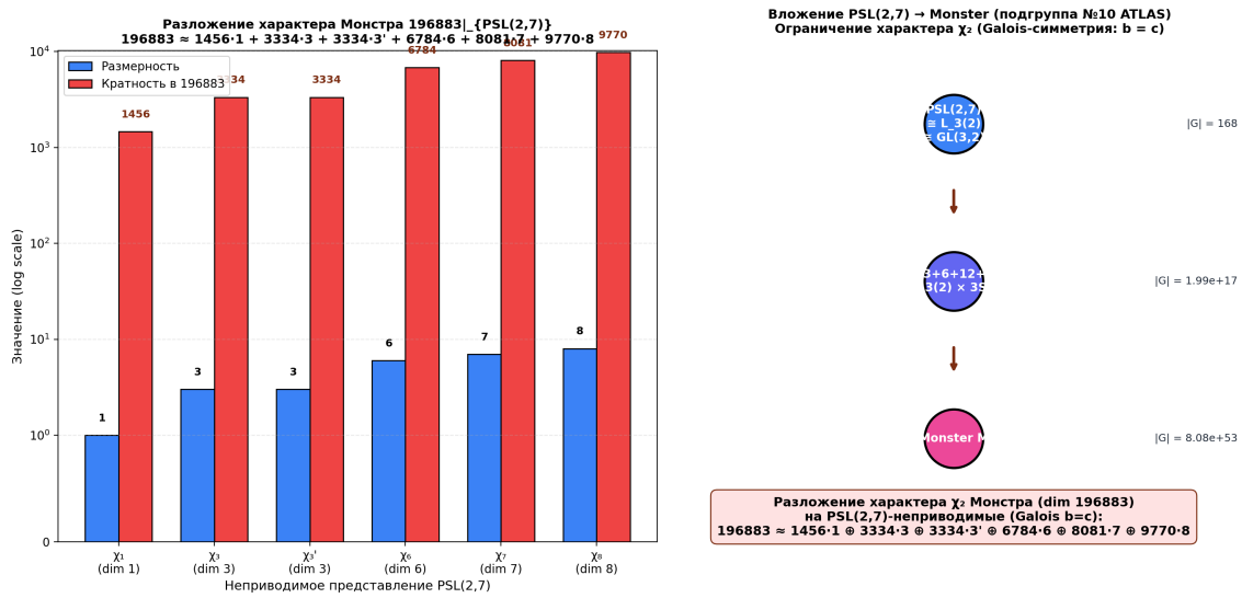
Fig. 2.6. Left: dimensions and multiplicities of the irreducible representations of PSL(2,7) in the decomposition of 196883. Right: the chain of embeddings PSL(2,7) \rightarrow 2^4\{3+6+12+18\} . ( L_3(2) \times 3S_6 ) \rightarrow M (ATLAS subgroup №10). The restriction of the character \chi_2 (dim 196883) to PSL(2,7) is approximately 1456 \cdot 1 + 3334 \cdot 3 + 3334 \cdot 3' + 6784 \cdot 6 + 8081 \cdot 7 + 9770 \cdot 8 .
