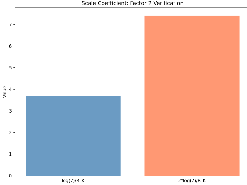
Figure 11.12. Scaling factor: verification of factor 2.
