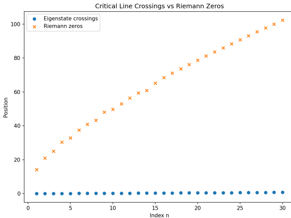
Figure 11.14. Crossings of the critical line by eigenstates vs zeros of \zeta .
