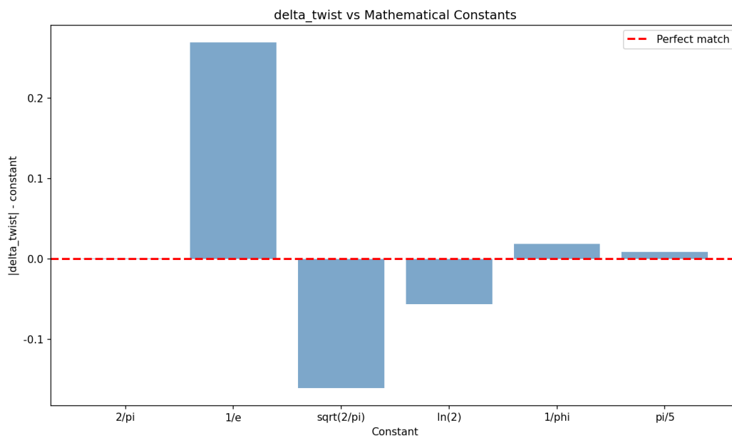
Figure 11.9. \delta_{\text{twist}} vs mathematical constants: 2/\pi — the best approximation.
