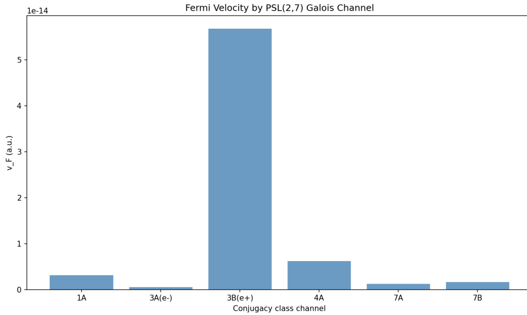
Figure 11.1. Fermi velocity across 6 Galois channels of PSL(2,7) .
