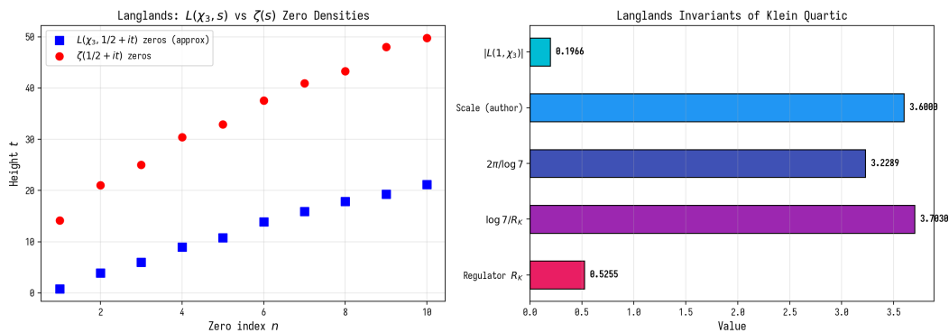
Fig. 8.1. L-functions and Langlands invariants of the Klein quartic.
