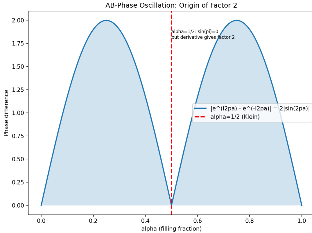
Figure 11.11. AB-phase oscillation: source of factor 2.
