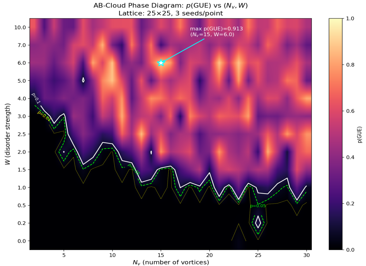
Figure 3. Phase diagram p(\text{GUE})(N_v, W) . GUE — broad plateau at W \geq 2, N_v \geq 5 .
