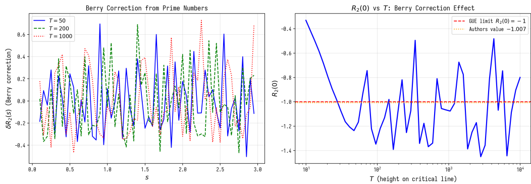
Figure 5.1. Berry corrections to R_2(s) and R_2(0) vs T .
