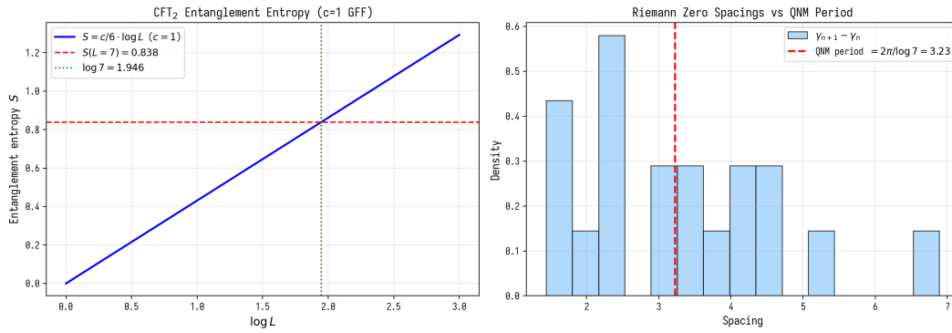
Figure 5.3. Entanglement entropy and QNM-period.
