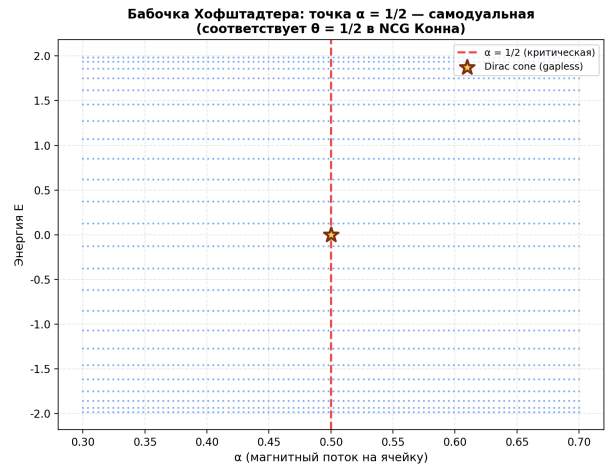
Fig. 6.3. Left: Morita involution \theta \rightarrow 1-\theta with fixed point \theta = 1/2 (self-duality of T_{\{1/2\}} ), parallel to the involution s \rightarrow 1-s with fixed point s = 1/2 (Riemann functional equation). Right: Hofstadter butterfly; the point \alpha = 1/2 is self-dual (Dirac cone without a gap).
