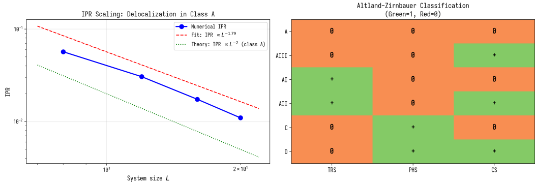
Figure 4.1. IPR-scaling and Altland-Zirnbauer classification.
