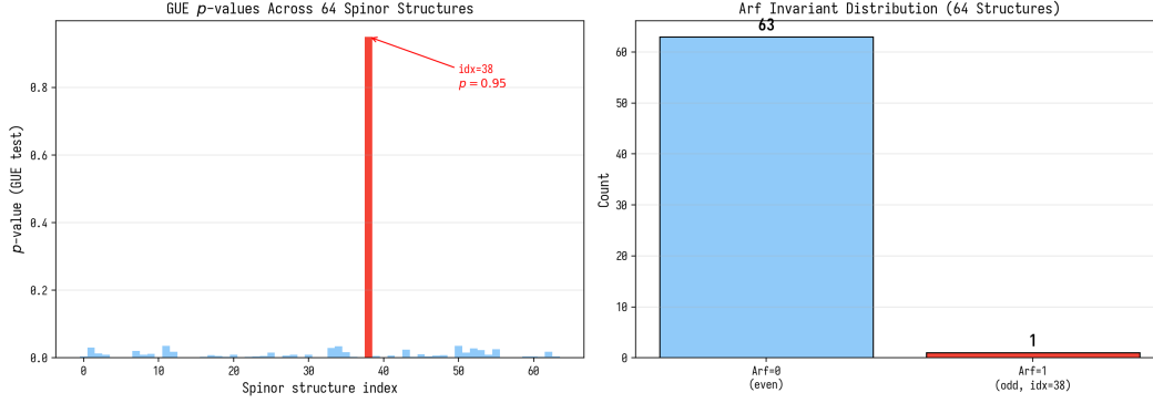
Figure 3.1. GUE p -values across 64 spinor structures and the Arf invariant.
