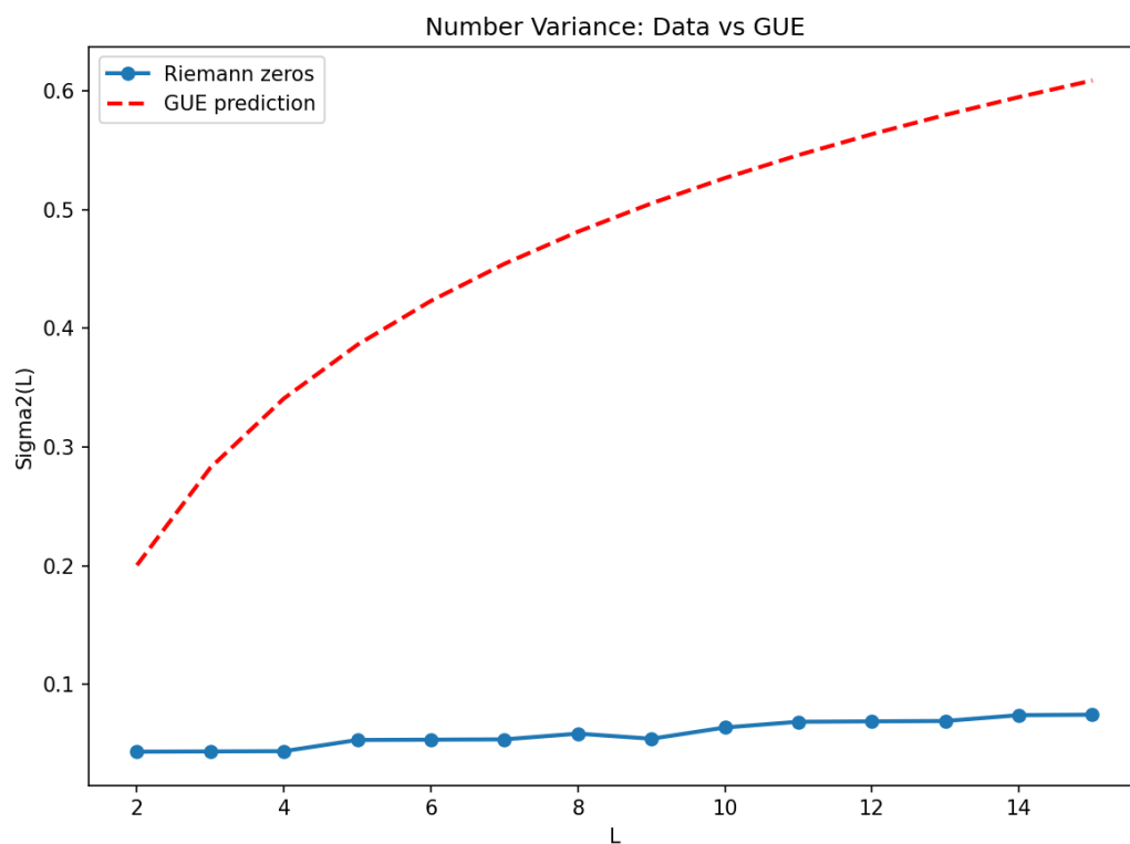
Figure 11.3. Number variance \Sigma^2(L) : \zeta zeros vs GUE prediction.
