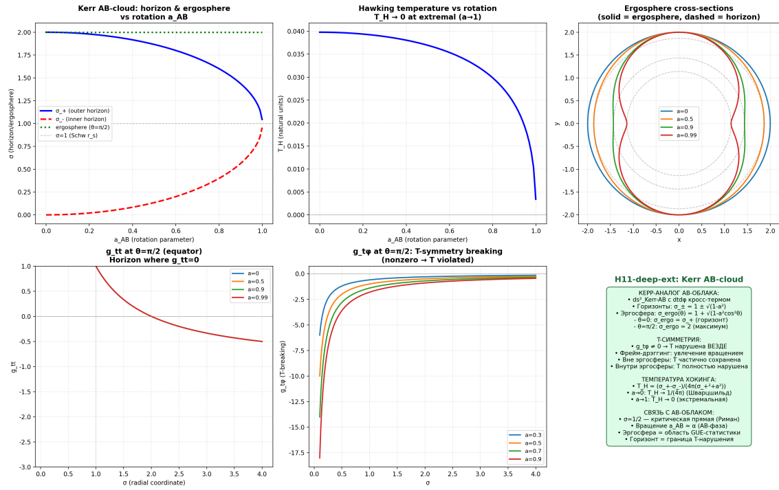
Fig. 13.3. Kerr-AB-cloud: horizons \sigma_{\pm} = 1 \pm \sqrt{1-a^2} , ergosphere \sigma_{ergo}(\theta) = 1 + \sqrt{1-a^2 \cos^2 \theta} , T-violation ( g_{t\phi} \neq 0 ).
