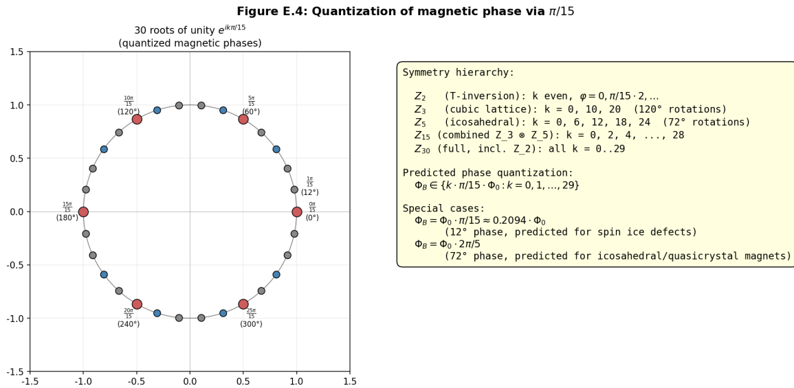
Figure E.4. Quantization of magnetic phase by \pi/15 . Left: 30 roots of 30th unity on the unit circle ( e^{ik\pi/15} , k=0..29 ), special phases Z_2 ( k even), Z_3 ( k \equiv 0 \pmod{10} ), Z_5 ( k \equiv 0 \pmod{6} ) are highlighted. Right: hierarchy of symmetries and predicted quantization of magnetic flux.
