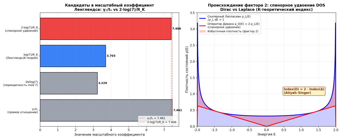
Fig. 11.13. Left: candidates for the Langlands scaling coefficient. Right: the density of states of the Dirac operator \rho_D(E) is twice that of the scalar Laplacian \rho_\Delta(E) — the physical source of the factor 2 (Atiyah-Singer index theorem).
