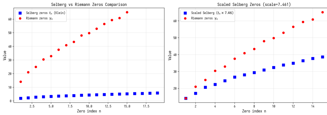
Figure 2.1. Comparison of Selberg zeros (Klein quartic) and Riemann zeros.
