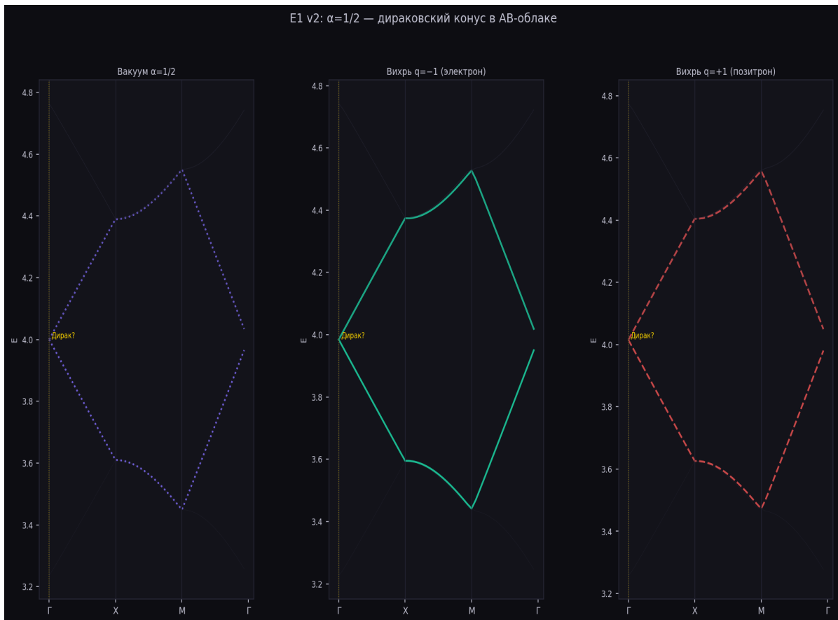
Fig. E1 v2: vortex dispersion at \alpha=1/2 . Dirac cone.
