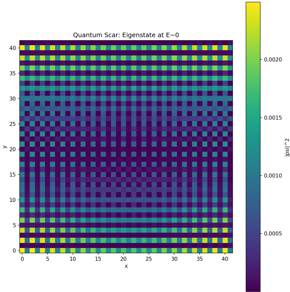
Figure 11.13. Quantum scar: eigenstate at E \approx 0 .
