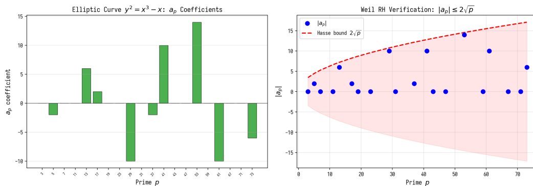
Fig. 7.3. RH for y^{2=x}3-x : a_p and Hasse bound.
