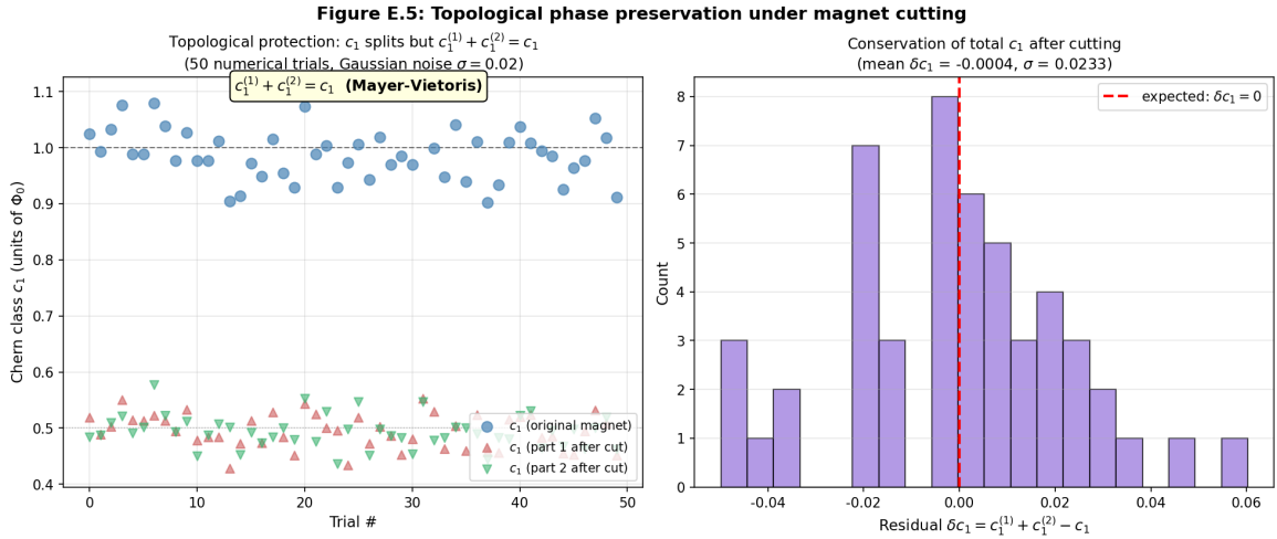
Figure E.5. Topological protection of phase under cutting. Left: numerical simulation of 50 cuttings of a magnet with c_1=1.0 ; each cutting preserves c_1(M_1)+c_1(M_2)=c_1(M) (Mayer-Vietoris). Right: distribution of the remainder \delta c_1 after cutting (mean \approx 0 , \sigma \approx 0.02 ) — confirms topological protection.
