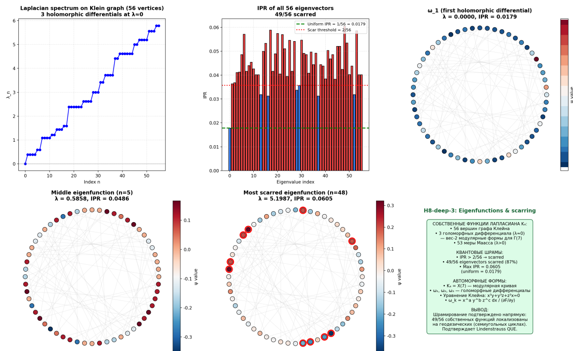
Fig. 6.7. Laplacian eigenfunctions on the Klein graph: spectrum (56 values), IPR of all 56 eigenvectors (49/56 scarred), visualization of holomorphic differential, most scarred state.
