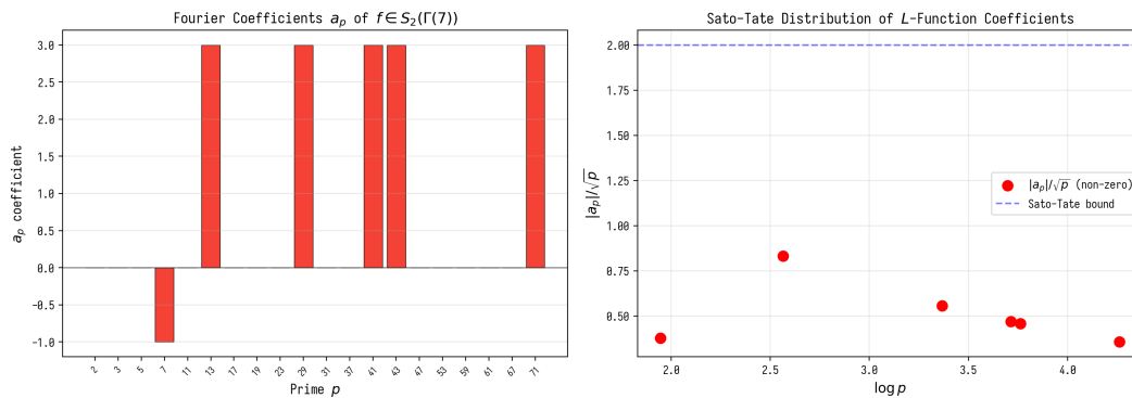
Figure 2.3. Fourier coefficients a_p of the level 7 modular form.
