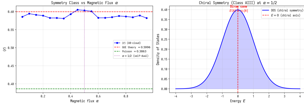
Fig. 6.2. Symmetry class vs \alpha and chiral DOS at \alpha=1/2 .
