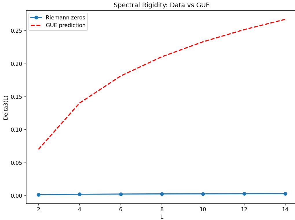
Figure 11.4. Spectral rigidity \Delta_3(L) : \zeta zeros vs GUE prediction.
