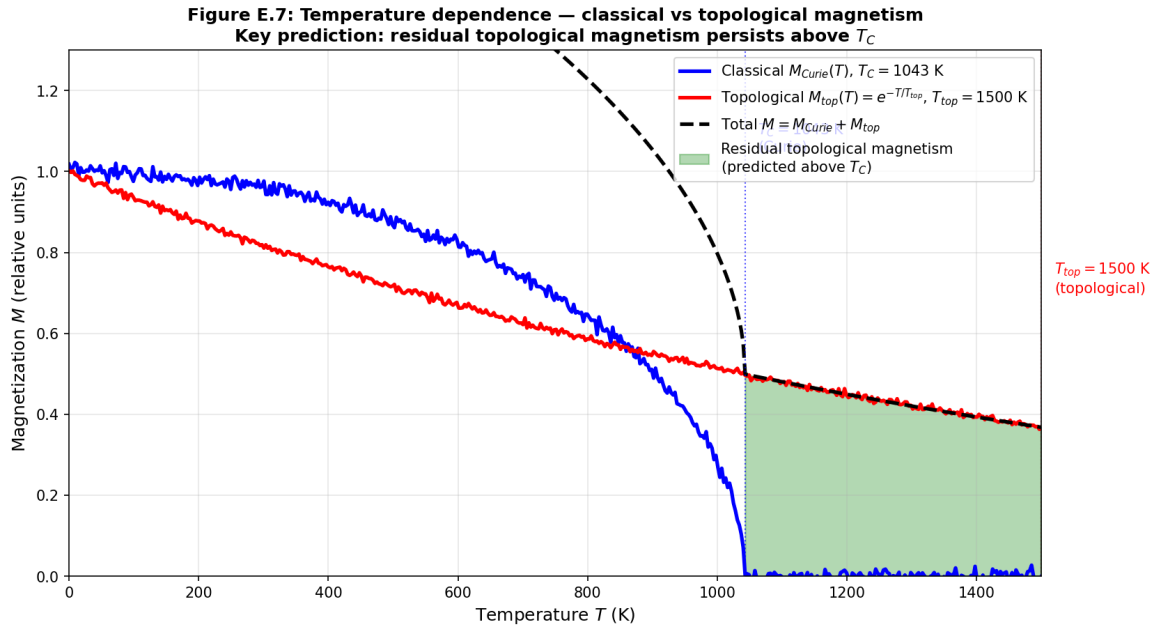
Figure E.7. Temperature dependence of magnetism: classical ( M_{Curie} , blue) and topological ( M_{top} , red) components. The green area is the “topological window” T_C < T < T_{top} , where residual topological magnetization is observed (key prediction).
