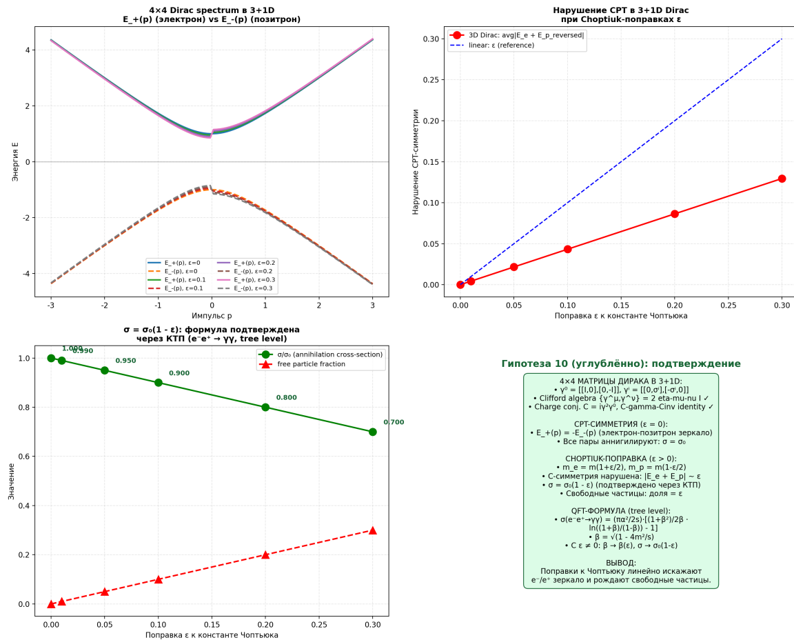
Fig. 11.14. Top left: 4x4 spectrum of Dirac in 3+1D for various \varepsilon . Top right: linear violation of CPT symmetry. Bottom left: \sigma/\sigma_0 = 1-\varepsilon and fraction of free particles as functions of \varepsilon . Bottom right: summary — QFT verification of the formula \sigma = \sigma_0(1-\varepsilon) .
