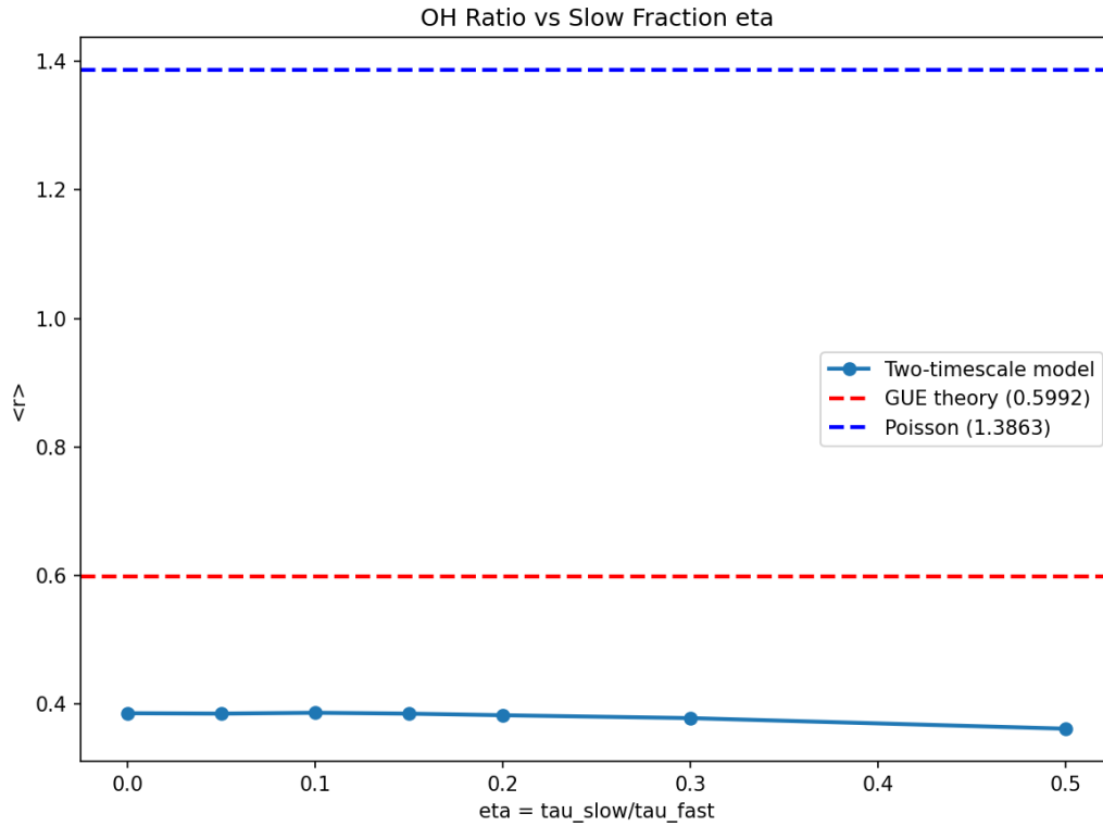
Figure 11.5. Oganessian–Hughes ratio \langle r \rangle vs two-scale model parameter \eta .
