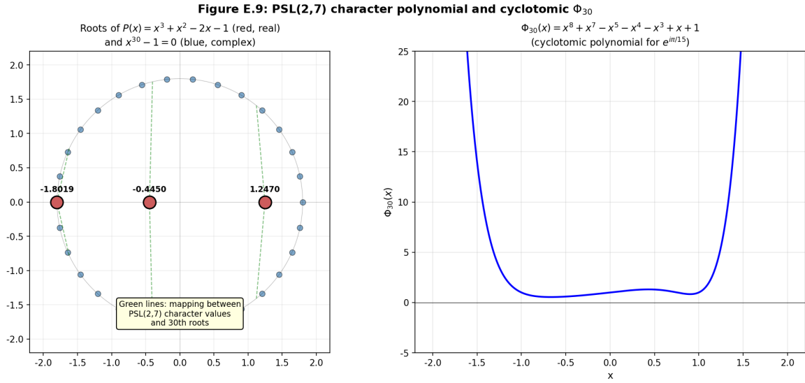
Figure E.9. Connection between PSL(2,7) and cyclotomic theory \Phi_{30} . Left: roots of the polynomial P(x)=x^3+x^2-2x-1 (character of PSL(2,7) , red points) and 30 roots of unity of order 30 (blue). Right: plot of the cyclotomic polynomial \Phi_{30}(x) with real roots.
