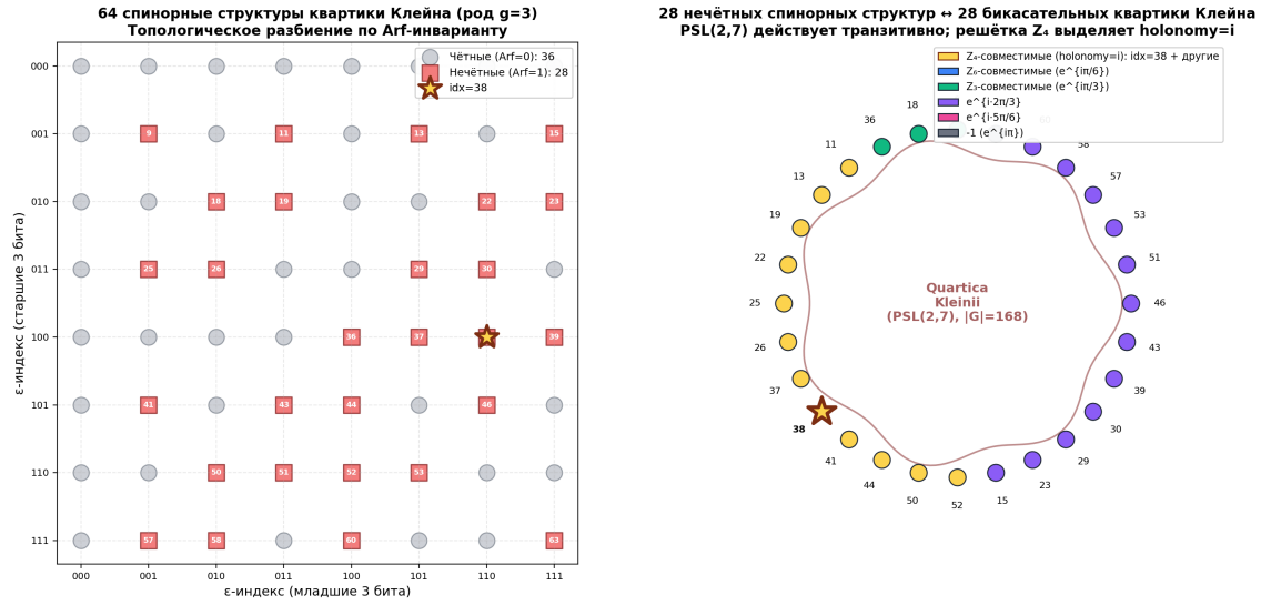
Fig. 3.3. Left: 64 spinor structures of the Klein quartic, colored by Arf invariant (36 even + 28 odd); \text{idx}=38 is marked with a star. Right: 28 odd structures as bitangents on a schematic Klein quartic; color codes Z_k compatibility of holonomy. \text{PSL}(2,7) acts transitively; the Z_4 subgroup of the square lattice selects structures with holonomy i .
