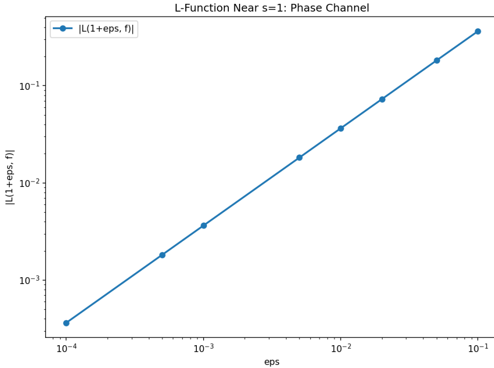
Figure 11.6. L -function near s=1 : linear behavior |L(1+\varepsilon, f)| \approx 3.647\varepsilon .
