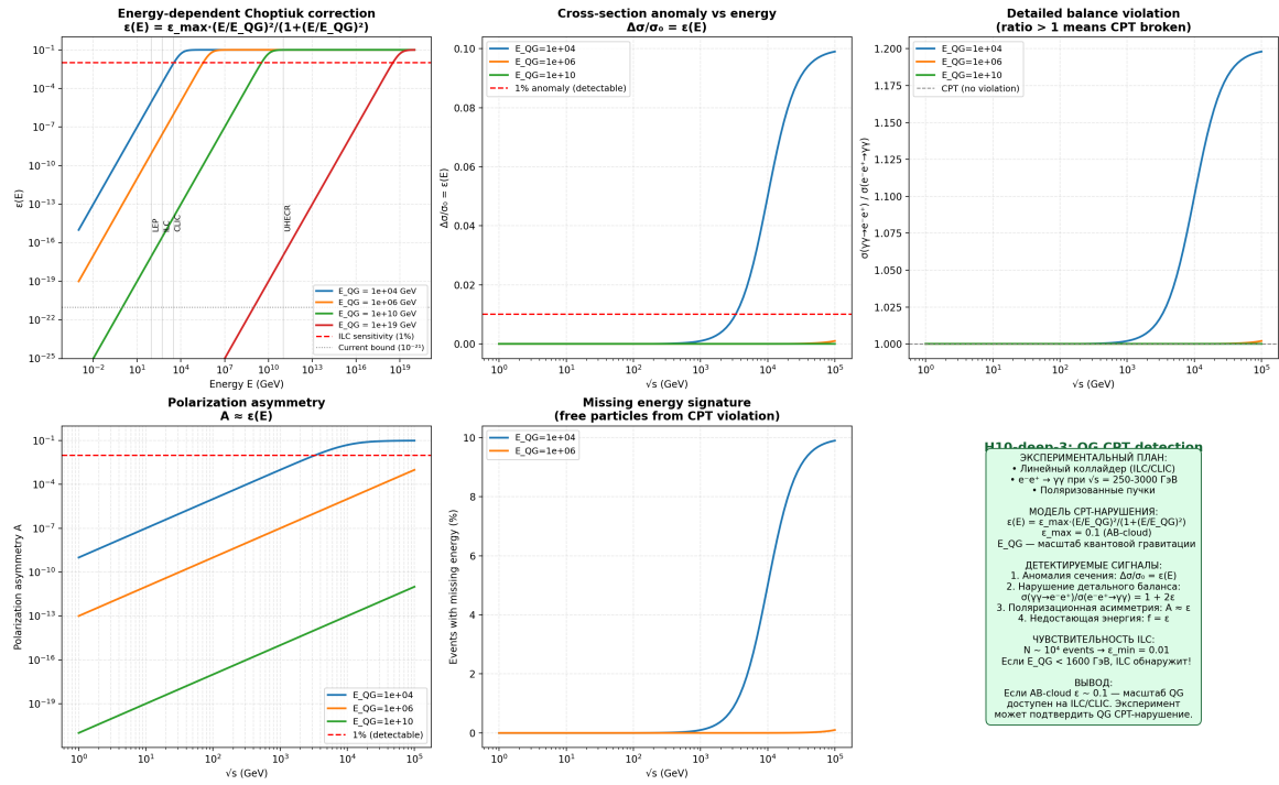
Fig. 11.16. Four signatures of QG-CPT violation at ILC/CLIC: cross-section anomaly, detailed balance, polarization, missing energy.
