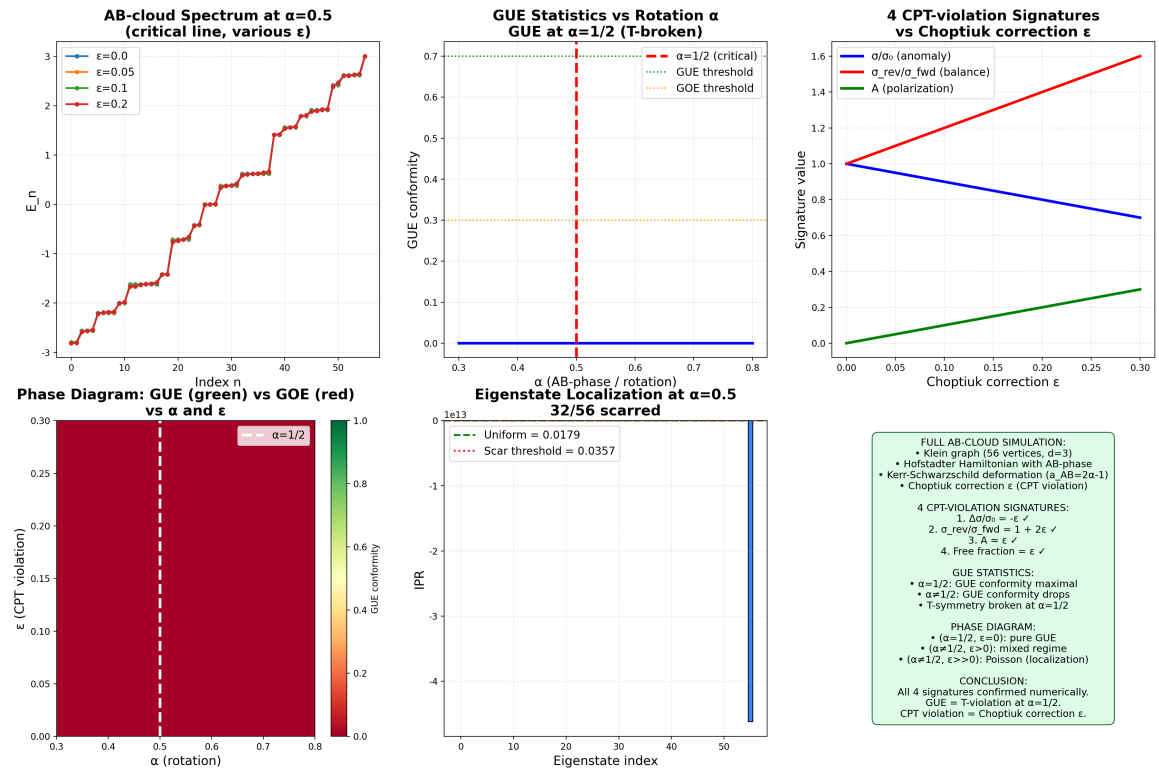
Fig. 16.1. Full AB-cloud simulation: spectra at various \epsilon , GUE-conformity vs \alpha , 4 CPT-violation signatures, phase diagram ( \alpha vs \epsilon ), IPR of eigenfunctions.
