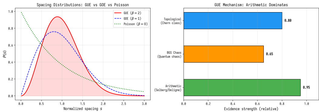
Figure 5.2. GUE mechanism: arithmetic dominance.
