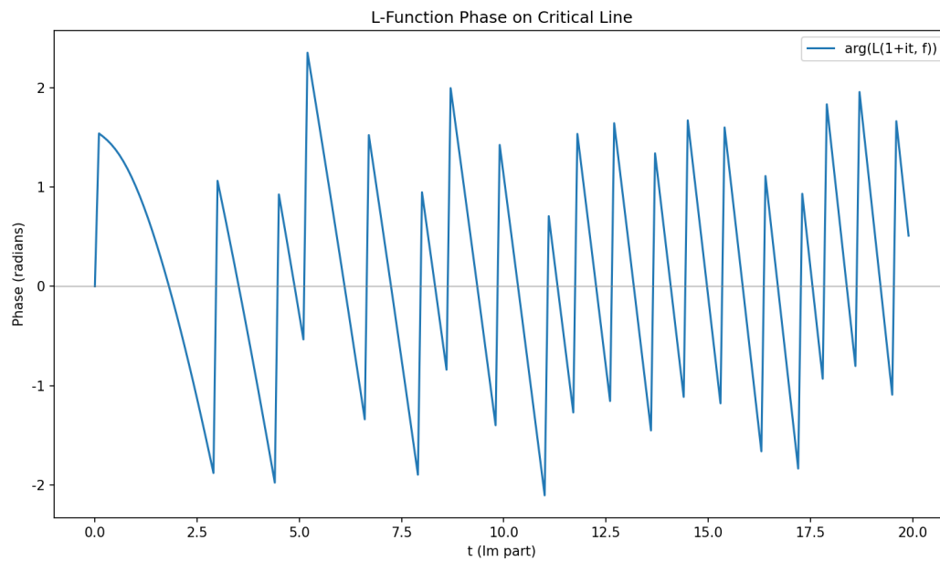
Figure 11.8. Phase \arg(L(1+it, f)) : jumps of \pi at zeros.
