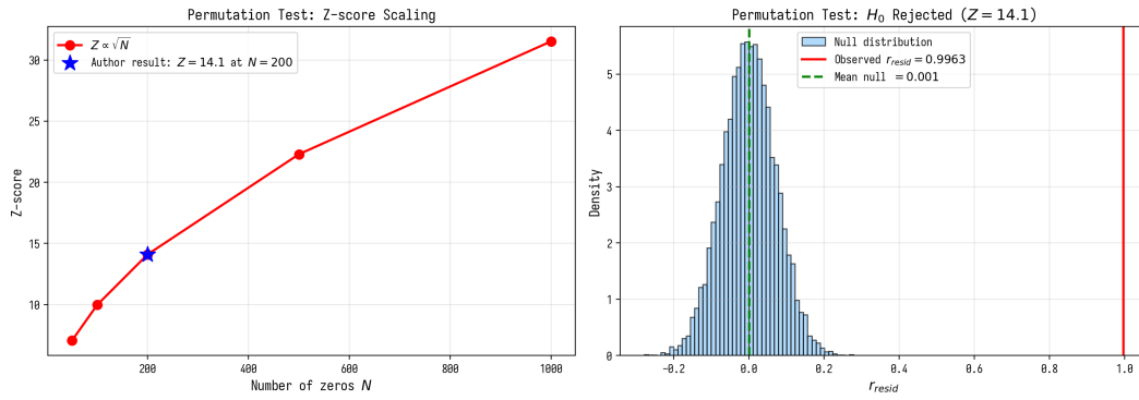
Figure 3.3. Scaling of Z-score and the null distribution of the permutation test.
