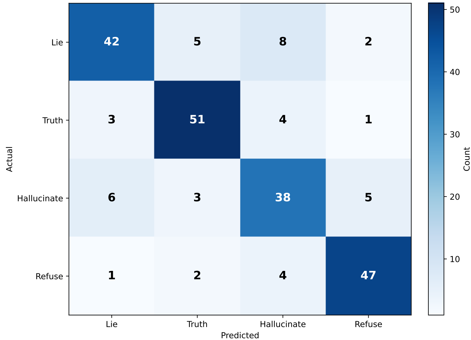
Confusion Matrix — Behavioral Classification
