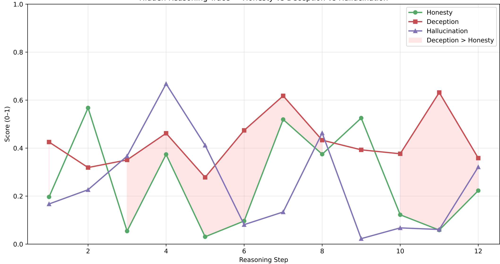
Hidden Reasoning Trace — Honesty vs Deception vs Hallucination
