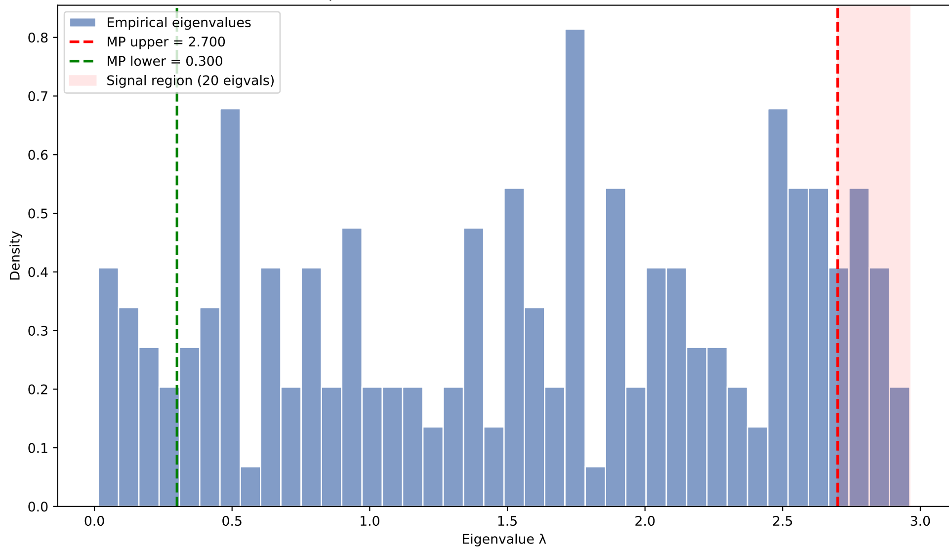
Spectral Distribution vs Marchenko-Pastur Bulk
