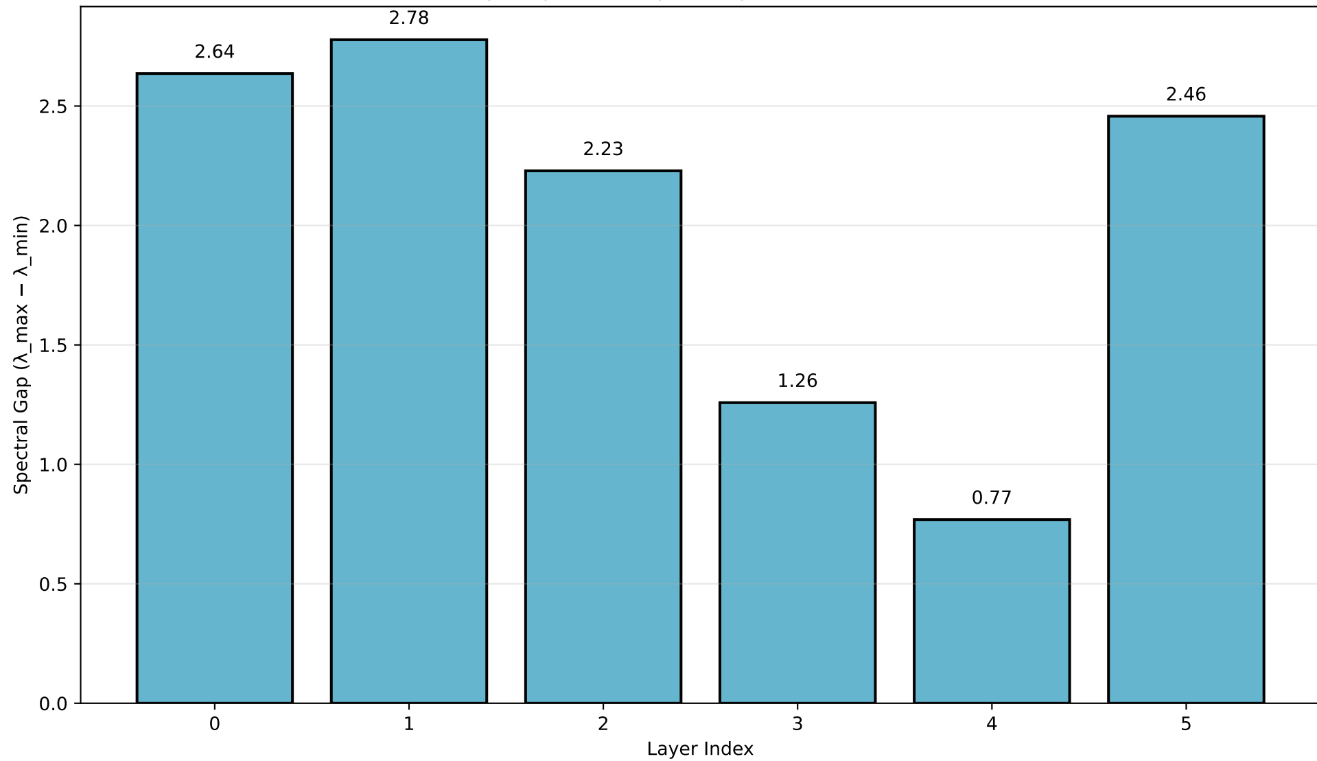
Per-Layer Spectral Gap — Cognitive Mode Indicator
