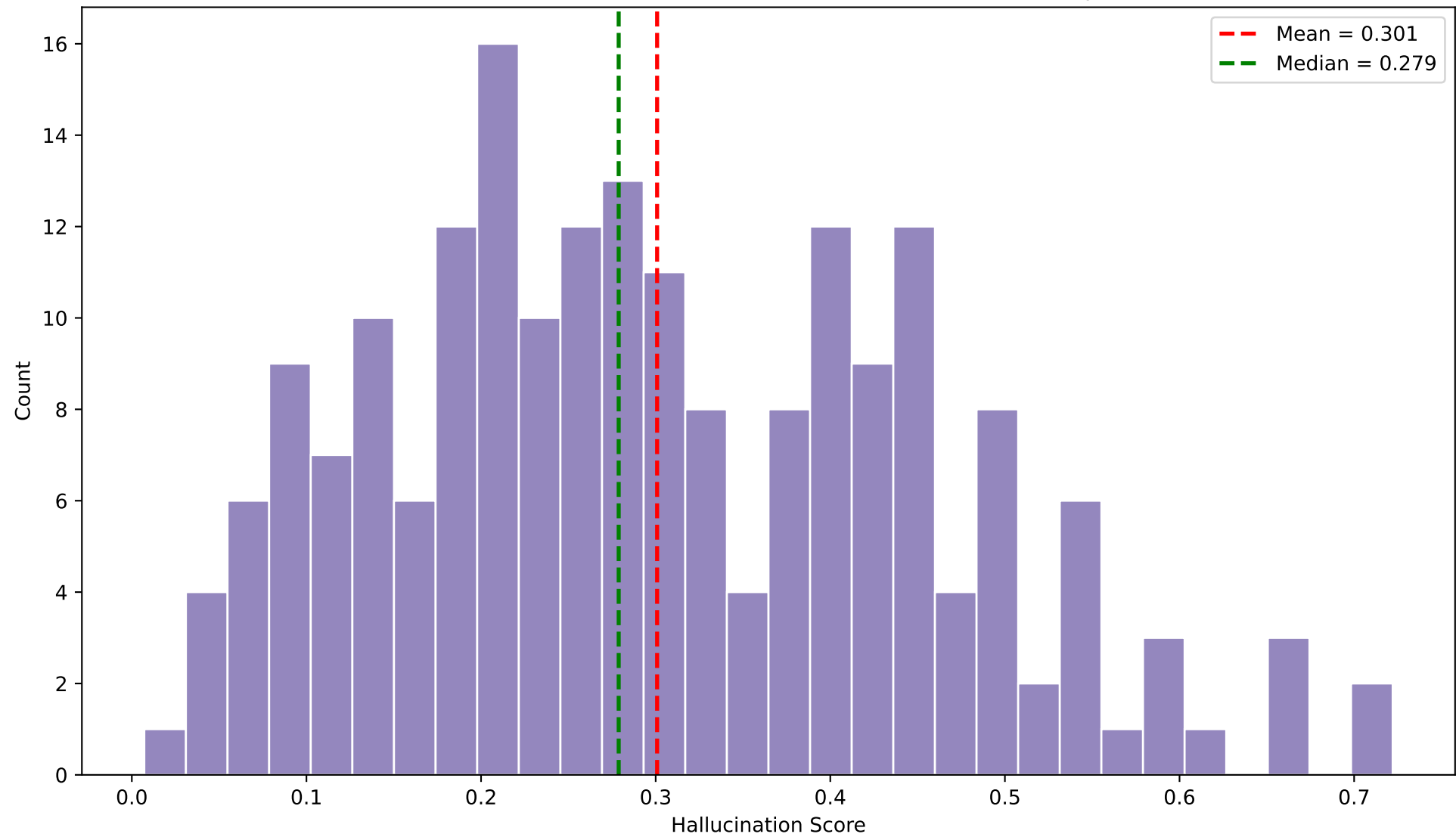
Hallucination Score Distribution Across Generation Steps
