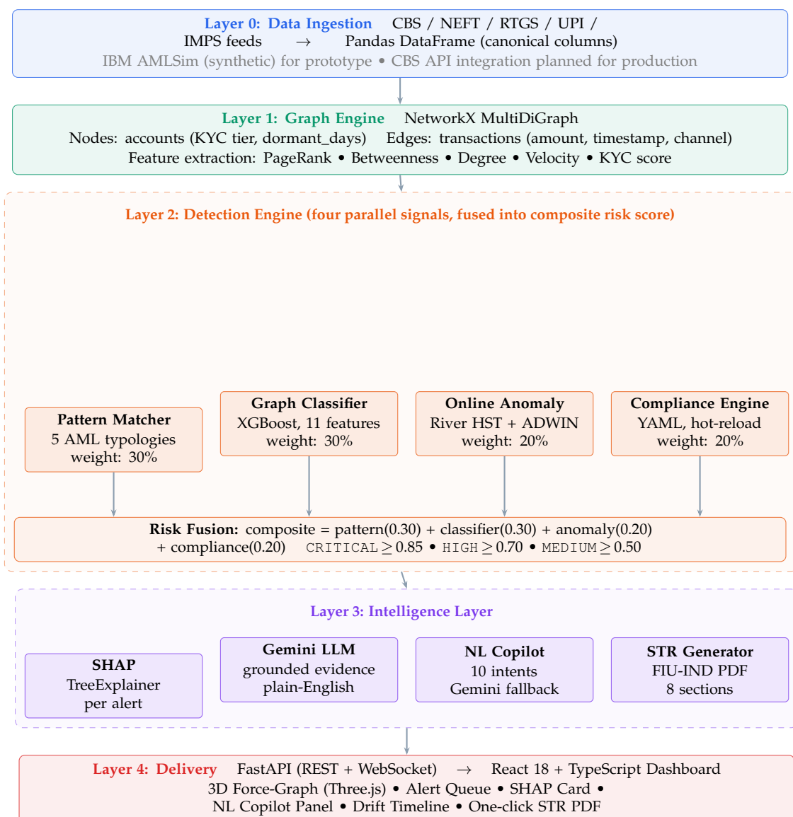
Figure 1: TRACE.ai five-layer architecture with one-directional data flow.
