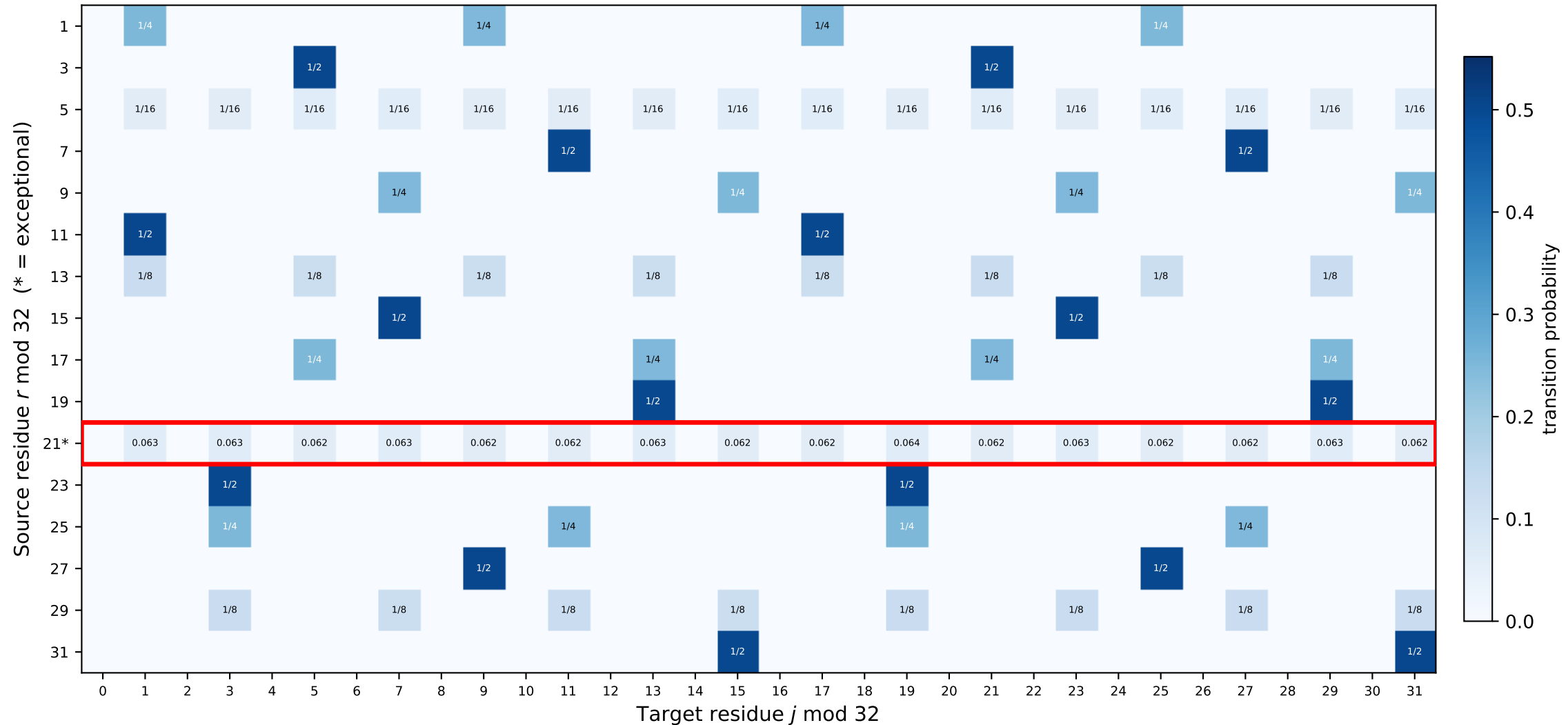
Transition matrix T[32] : exact rows show 0 or 1/2^v ; red border = exceptional row r = 21 ( v_2(64) = 6 > \log_2 32 )
