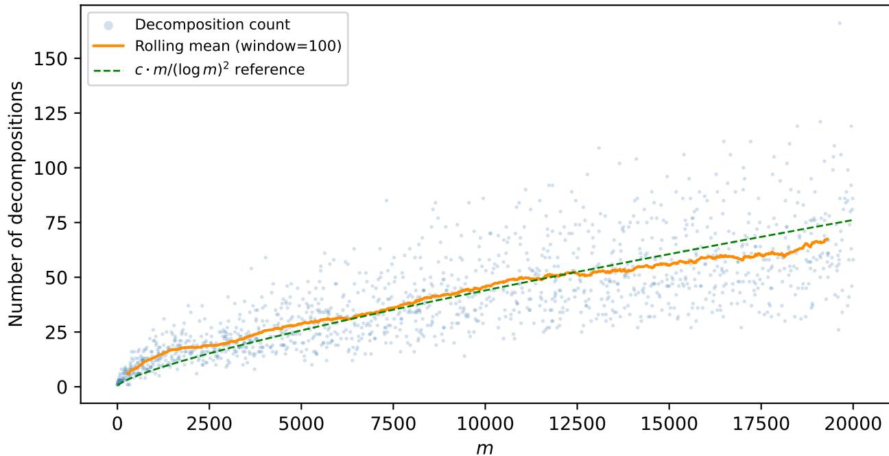
Middle number decomposition count for A002822
