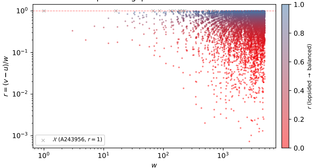
Decomposition gap ratio r for A002822 \cup \mathcal{X}
