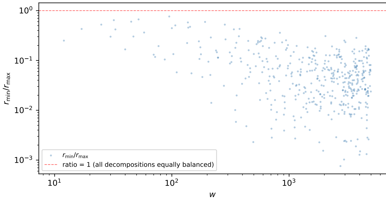
Ratio of smallest to largest gap ratio r for A002822
