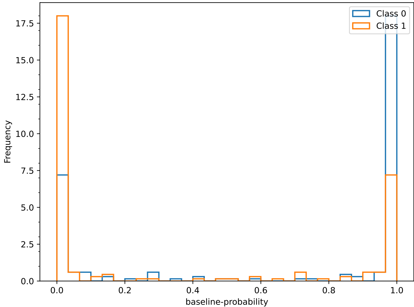
Histogram of baseline-probability
