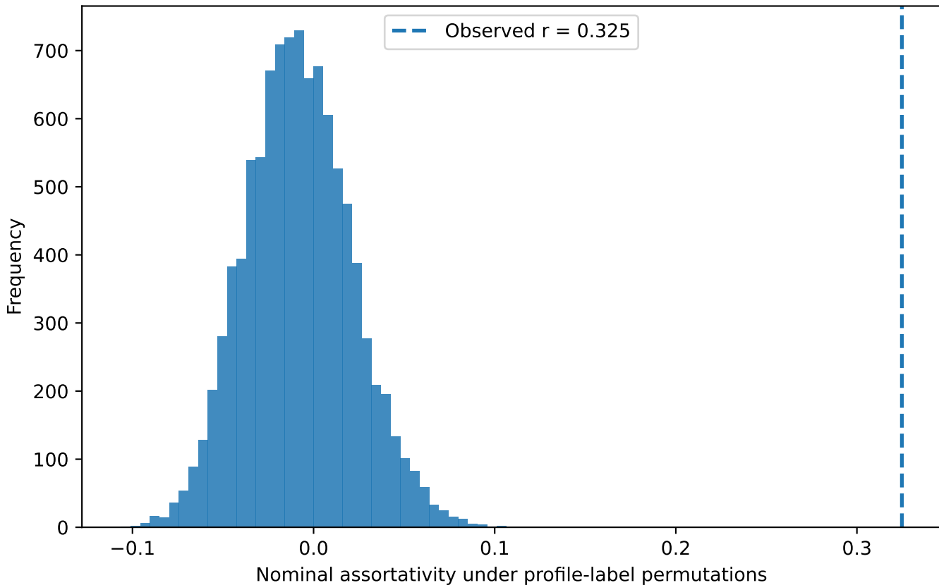
Spatial assortment of SOM profiles on Queen-contiguity graph
