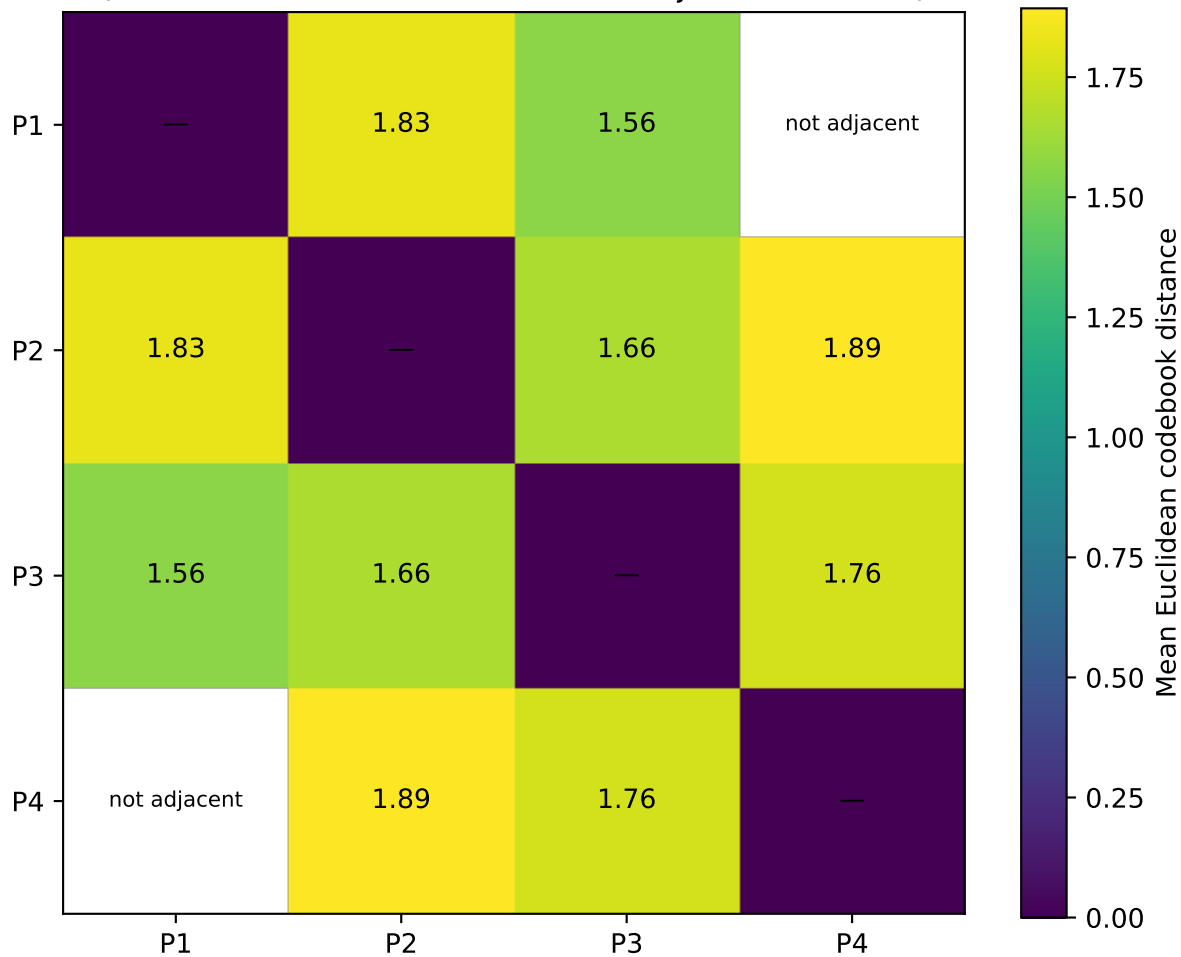
SOM macroprofile boundary strength (mean codebook distance across adjacent neurons)
