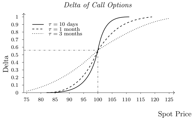
Figure 6.2. Variation of delta of a European call option with respect to S and T . K = 100 , r = 0.05 , \sigma = 0.25 .
