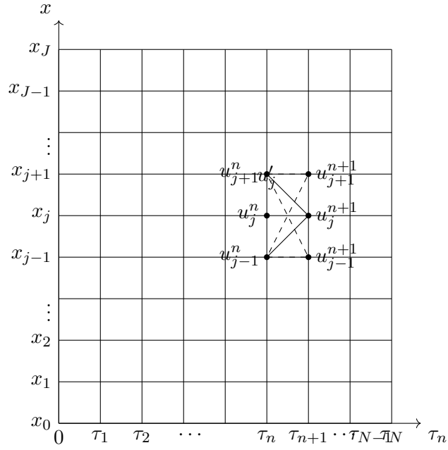
Figure 7.2. Grid of \tau and x for finite difference methods
