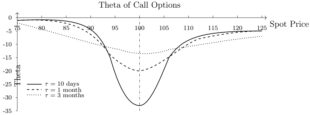
Figure 6.4. Variation of theta of a European call option with respect to S and T . K = 100 , \sigma = 0.25 , r = 0.05 .
