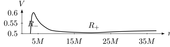
Figure 6.4. The effective potential, V , for timelike geodesics in the case L^2 = 24M^2 . (Note that the scale of V is greatly expanded as compared with Figure 6.3.)
