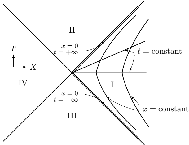
Figure 6.8. Rindler spacetime, displayed as the wedge, I, of two-dimensional Minkowski spacetime.
