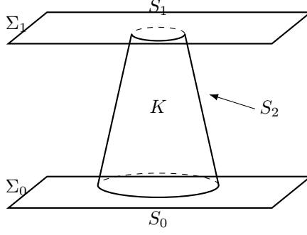
Figure 10.1. A spacetime diagram showing the region K over which Eq. (10.1.9) is integrated to obtain equation (10.1.10).
