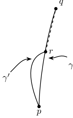
Figure 9.3. A spacetime diagram illustrating the fact that if a timelike geodesic \gamma connecting points p and q has a point r conjugate to p lying between p and q , then a nearby timelike curve \gamma' connecting p and q can be constructed which has greater elapsed proper time than \gamma (see theorem 9.3.3).
