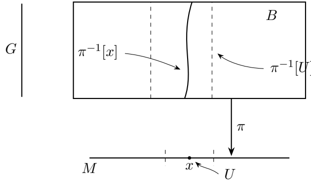
Figure 13.2. A diagram illustrating the structure of a principal fiber bundle (see text).
