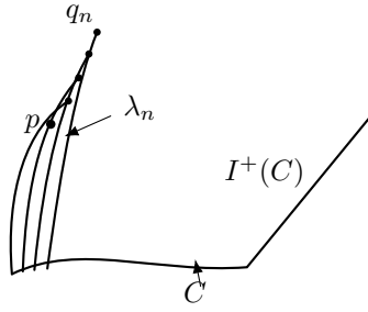
Figure 8.4. A spacetime diagram showing a sequence of points in I^+(C) converging to p \in \partial I^+(C) (see theorem 8.1.6).
