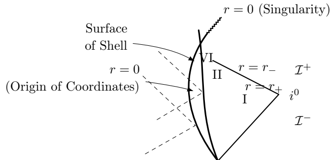
Figure 12.5. A conformal diagram of a spacetime in which a charged spherical shell with M > \mathcal{M} > |e| undergoes gravitational collapse. The dashed lines refer to the extended Reissner–Nordstrom spacetime.
