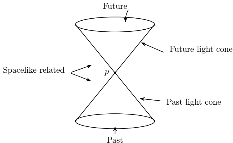
Figure 1.2. A diagram showing the causal structure of spacetime in special relativity. The “light cone” of p rather than a “surface of simultaneity” with p now plays a fundamental role in determining the causal relationship of p to other events.
