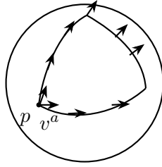
Figure 3.2. The parallel transport of a vector, v^a , around a closed curve on the sphere. In the case shown here of a closed curve composed of three mutually orthogonal segments of great circles, the vector v^a comes back rotated by 90^\circ .
