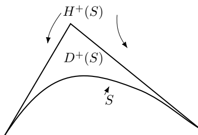
Figure 8.12. A spacetime diagram showing D^+(S) and H^+(S) for a particular closed achronal set S in Minkowski spacetime. Here S is “asymptotically null” to the right and becomes “exactly null” to the left. This example shows that H^+(S) can intersect S even if \text{edge}(S) = \emptyset .
