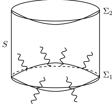
Figure 4.3. Asymptotically null hypersurfaces \Sigma_1 and \Sigma_2 . The gravitational radiation “registers” on \Sigma_1 but does not “register” on \Sigma_2 . The energy, \Delta E , carried off to infinity by gravitational radiation is given by an integral over the timelike hypersurface S .
