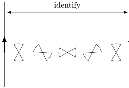
Figure 8.1. A non-time-orientable spacetime.
