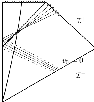
Figure 14.3. A conformal diagram of a spherically symmetric spacetime in which gravitational collapse to a Schwarzschild black hole occurs, showing the oscillations of a wave which behaves as e^{-i\omega u} on \mathcal{I}^+ . If one propagates this wave backward into the past starting from \mathcal{I}^+ , the part of the wave which propagates through the collapsing matter will produce an “infinite blueshift” singularity—of the same nature as shown on the white hole horizon in Figure 14.2—at advanced time v_0 on \mathcal{I}^- .
