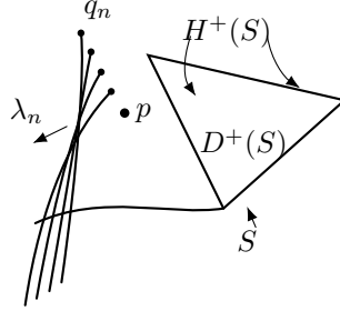
Figure 8.13. A point p \in H^+(S) \cap I^+(S) with a sequence of points q_n \in I^+(p) converging to p (see theorem 8.3.5).
