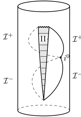
Figure 12.1. A conformal diagram of the same spacetime as shown in Figures 6.11 and 6.12. From this conformal diagram, it is apparent that region II of the physical spacetime lies outside of J^-(\mathcal{I}^+) . In contrast, in Figure 11.1, J^-(\mathcal{I}^+) includes the entire physical spacetime.
