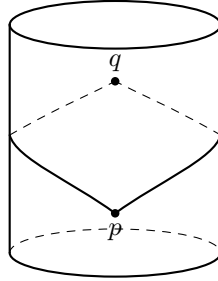
Figure 8.5. A spacetime diagram of a two-dimensional flat spacetime with topology \mathbb{R} \times S^1 . The null geodesic generators of \partial I^+(p) have q as a future endpoint.
