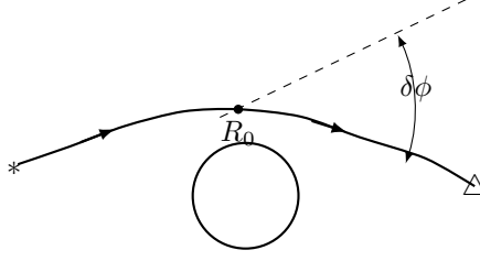
Figure 6.6. Diagram illustrating the bending of light effect.
