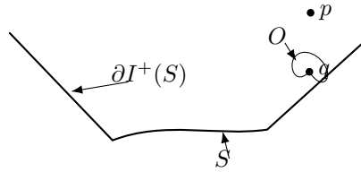
Figure 8.3. A spacetime diagram showing a set S and the boundary of its future, \partial I^+(S) (see theorem 8.1.3).
