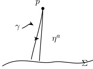
Figure 9.4. A spacetime diagram depicting a point p conjugate to the hypersurface \Sigma along the geodesic \gamma . (The two geodesics shown are supposed to be “infinitesimally nearby.”)
