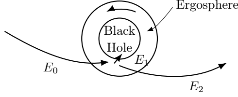
Figure 12.7. A diagram illustrating the Penrose process for extracting energy from a Kerr black hole.
