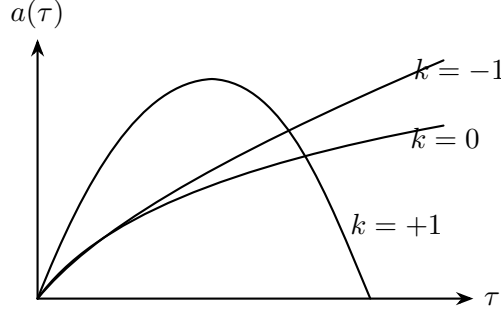
Figure 5.3. The dynamics of dust-filled Robertson–Walker universes.
