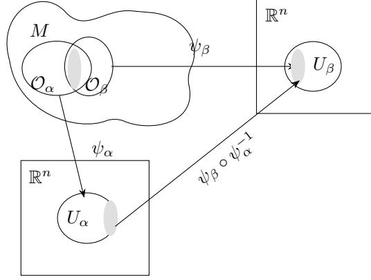
Figure 2.1. An illustration of the map \psi_\beta \circ \psi_\alpha^{-1} arising when two coordinate systems overlap.
