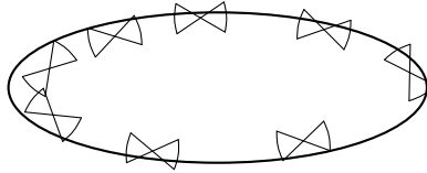
Figure 8.7. A spacetime with topology \mathbb{R}^4 where the light cones “tip over” sufficiently to permit the existence of closed timelike curves.
