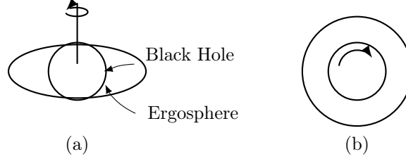
Figure 12.6. A sketch showing (a) a “side view” and (b) a “top view” of the ergosphere of a Kerr black hole.
