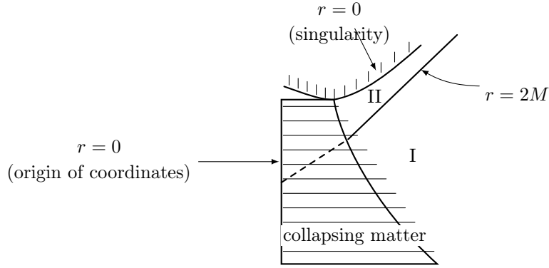
Figure 6.11. The spacetime resulting from the complete gravitational collapse of a spherical body. All of regions III and IV of the extended Schwarzschild spacetime (Figure 6.9) are covered up by the collapsing matter. However, part of the black hole region II is produced.
