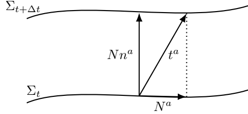
Figure 10.2. A spacetime diagram illustrating the definition of the lapse function, N , and shift vector N^a .
