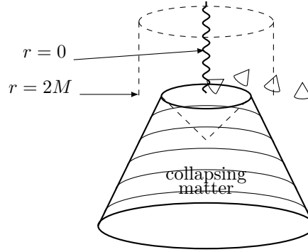
Figure 6.12. Another representation of the spacetime of Figure 6.11. Here, one of the two suppressed spatial dimensions is restored, so each of the circles shown on the collapsing body corresponds to the 2-sphere surface of the body at an instant of time. However, the light cones no longer are represented by 45^\circ lines. Indeed, the spacelike nature of the singularity and the inevitable capture by the singularity of any particle or light ray in the region r < 2M is illustrated here by the tipping over of the future light cones in the strong field region.
