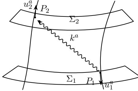
Figure 5.5. A spacetime diagram showing the emission of a light signal at event P_1 and its reception at event P_2 .
