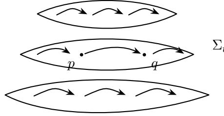
Figure 5.1. The hypersurfaces of spatial homogeneity in spacetime. By definition of homogeneity, for each t and each p, q \in \Sigma_t , there exists an isometry of the spacetime which takes p into q .
