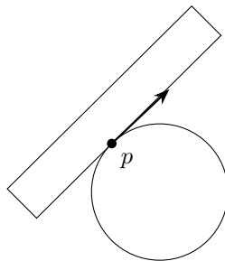
Figure 2.2. The tangent plane at point p of a sphere in \mathbb{R}^3 .
