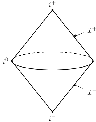
Figure 11.2. The region \bar{\mathcal{O}} of the Einstein static universe represented as two null cones joined at their base. This representation of \bar{\mathcal{O}} is misleading since it shows i^0 as a 2-sphere rather than as a point, but it often is much more convenient to use this representation for drawing spacetime diagrams than that of Figure 11.1.
