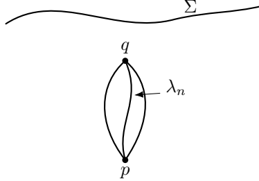
Figure 8.14. A sequence \{\lambda_n\} of causal curves from p to q in the case p, q \in D^-(\Sigma) (see theorem 8.3.9).
