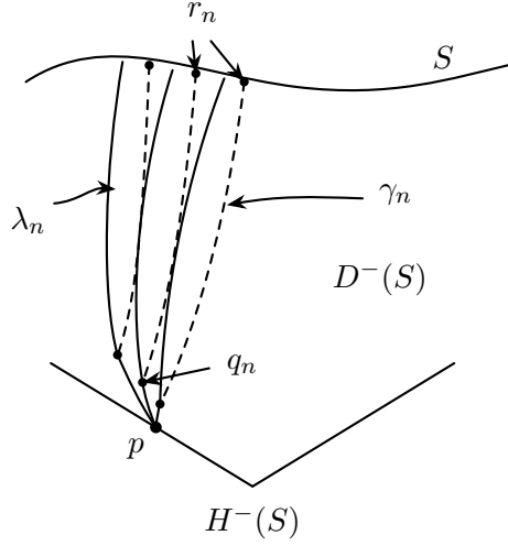
Figure 9.6. A spacetime diagram showing a construction used in the proof of theorem 9.5.2.
