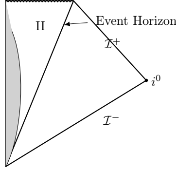
Figure 12.2. Another representation of the closure, \overline{M} , of the physical spacetime depicted in Figure 12.1. As in Figure 12.1, the angular dimensions are suppressed so each point in this diagram (except those at r = 0 and the point i^0 ) represents a 2-sphere.
