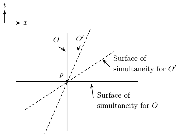
Figure 1.3. A spacetime diagram illustrating the fact that in special relativity the inertial observers O and O' disagree over the definition of simultaneity with event p .
