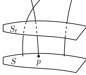
Figure 3.4. The construction of Gaussian normal coordinates starting from the hypersurface S . The geodesics orthogonal to S eventually may cross, but until they do, Gaussian normal coordinates are well defined and the surfaces, S_t , of constant t remain orthogonal to the geodesics.
