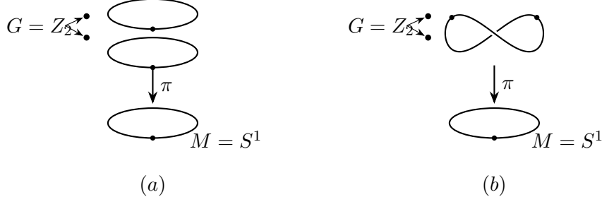
Figure 13.3. (a) The trivial principal fiber bundle Z_2 \times S^1 . (b) The principal bundle (S^1, Z_2, S^1, \phi) constructed in the text.
