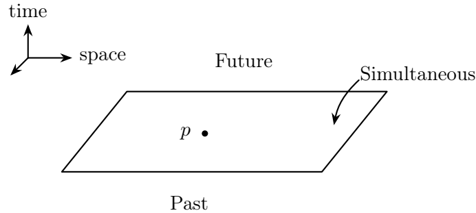
Figure 1.1. A diagram showing the causal structure of spacetime in prerelativity physics. Given an event p , all other events in spacetime either are to the future of p , to the past of p , or simultaneous with p . The simultaneous events form a three-dimensional surface in spacetime.
