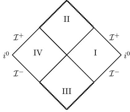
Figure 12.3. A conformal diagram of the extended Schwarzschild spacetime (see Figure 6.9), represented in the same manner as used in Figure 12.2. Note that since the extended Schwarzschild spacetime has two distinct asymptotically flat regions, two distinct conformal boundaries are shown.
