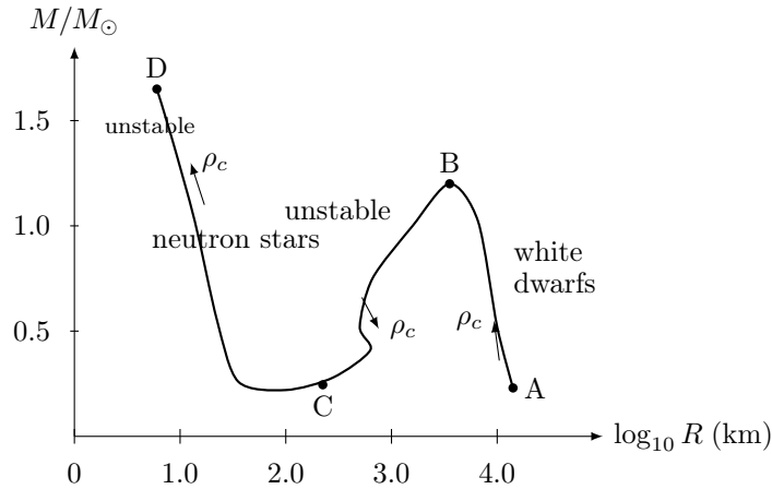
Figure 6.1. The equilibrium configurations of cold matter. Given an equation of state, P = P(\rho) , an equilibrium configuration is uniquely determined by the value of the central density \rho_c . The masses and radii of these configurations are shown for values of \rho_c ranging from \sim 10^5 \text{ g cm}^{-3} at point A to \sim 10^{17} \text{ g cm}^{-3} beyond point D. In the white dwarf regime, the values of M and R depend somewhat upon the assumed composition of the star. In the neutron star regime, the values of M and R depend greatly upon assumptions about the state of matter as well as assumptions about the interactions between the fundamental constituents of matter. In this latter regime, the figure is only a rough sketch of the qualitative features found for most equations of state.
