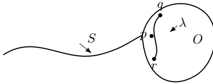
Figure 8.10. A spacetime diagram illustrating the definition of the edge of a closed, achronal set S .
