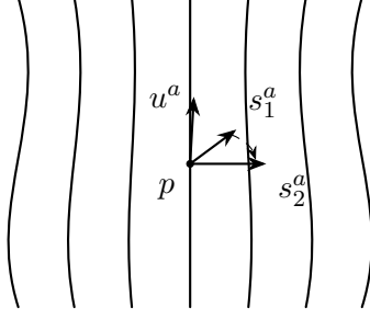
Figure 5.2. The world lines of isotropic observers in spacetime. By definition of isotropy, for any two vectors s_1^a, s_2^a at p which are orthogonal to u^a , there exists an isometry of the spacetime which leaves p fixed and rotates s_1^a into s_2^a .
