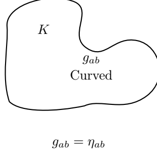
Figure 14.1. A spacetime diagram of a spacetime (\mathbb{R}^4, g_{ab}) which is isometric to Minkowski spacetime (\mathbb{R}^4, \eta_{ab}) outside of a compact region K .
