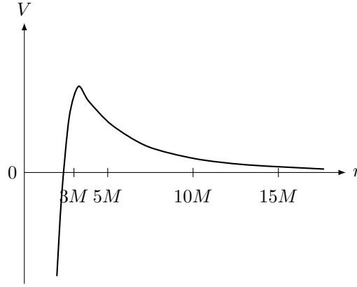
Figure 6.5. The effective potential, V , for null geodesics.
