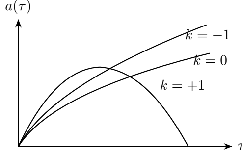
Figure 5.4. The dynamics of radiation-filled Robertson–Walker universes.
