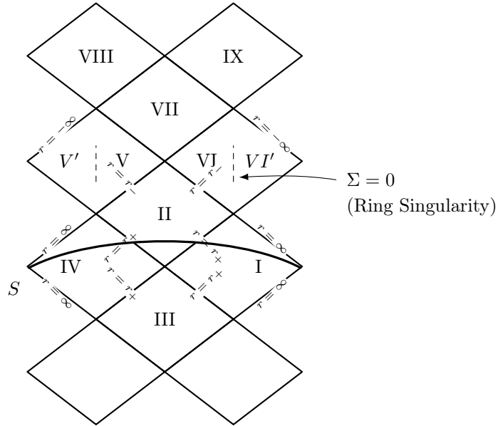
Figure 12.4. A conformal diagram of the extended charged Kerr spacetime in the case a \neq 0 , a^2 + e^2 < M^2 .
