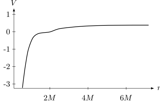
Figure 6.3. The effective potential, V , for timelike geodesics in the case L^2 = 6M^2 .
