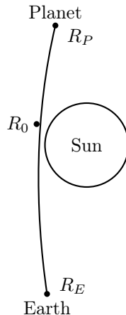
Figure 6.7. Diagram illustrating the time delay of light effect.
