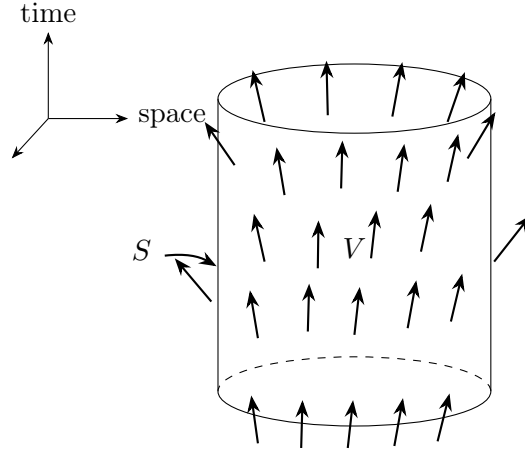
Figure 4.1. A spacetime diagram showing the mass-energy current density J^a in a volume V of spacetime.
