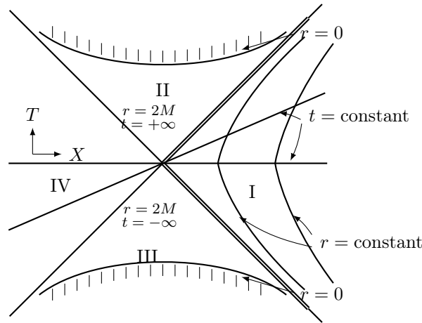
Figure 6.9. The Kruskal extension of Schwarzschild spacetime.
