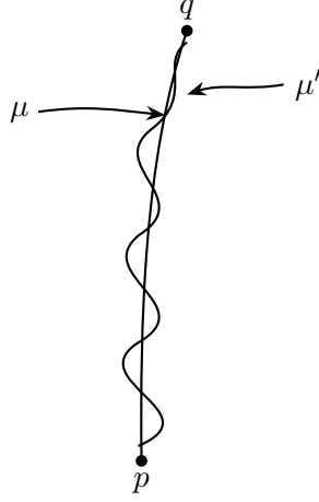
Figure 9.5. A smooth timelike curve \mu from p to q . Arbitrarily close to \mu in the topology of \mathcal{C}(p, q) is a smooth timelike curve \mu' with total elapsed proper time arbitrarily close to zero.
