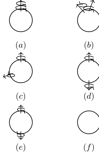
Figure 13.1. A diagram illustrating how a rotation of a sphere by 4\pi about a given axis can be continuously deformed to no rotation. We break up the 4\pi -rotation into two 2\pi -rotations and continuously change the axis of the second 2\pi -rotation until it is opposite the axis of the first rotation, as shown in the sequence (a)–(d). Then we continuously decrease the angle of both rotations to zero, as shown in the sequence (d)–(f).
