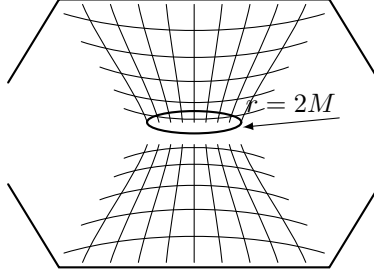
Figure 6.10. The spatial geometry of the hypersurface t = 0 of the Schwarzschild spacetime, shown as it would look if it were embedded in flat space. (One dimension is suppressed, i.e., the topology of the hypersurface is \mathbb{R} \times S^2 , not \mathbb{R} \times S^1 , so each circle—such as the one shown at r = 2M —really represents a two-sphere.) The portion of the surface lying above the throat at r = 2M in the figure corresponds to the portion lying in region I of Figure 6.9; the portion below r = 2M lies in region IV of Figure 6.9.
