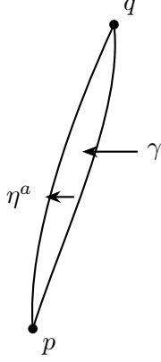
Figure 9.2. A spacetime diagram illustrating the notion of conjugate points along the geodesic \gamma .
