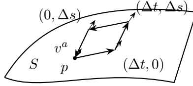
Figure 3.3. The parallel transport of a vector v^a around a small closed loop. As derived in the text, to second order in \Delta t and \Delta s , the change in v^a is governed by the Riemann tensor at p .
