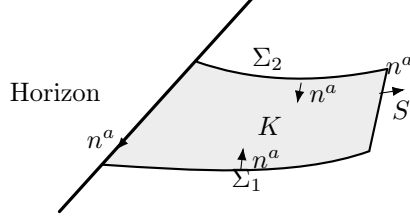
Figure 12.8. A spacetime diagram showing the region K over which \nabla_a f^a = 0 is integrated to derive the conclusion in the text concerning superradiant scattering. Here the spacelike hypersurface \Sigma_2 is a “time translate” of \Sigma_1 by \Delta t , and the timelike hypersurface S represents a “large sphere” at infinity. The integral of f^a n_a over S represents the net energy flow out of K to infinity (i.e., the outgoing minus incoming energy) during the time \Delta t , whereas the integral of f^a n_a over the horizon represents the net energy flow into the black hole. By Gauss’s law (see appendix B) the integral of f^a n_a over the entire boundary vanishes. (The appropriate directions of n^a on each part of the boundary are shown.) However, for a wave with time dependence e^{-i\omega t} the integrals over \Sigma_1 and \Sigma_2 cancel by time translation symmetry. Hence, the integral of f^a n_a over S equals minus the integral of f^a n_a over the horizon.
