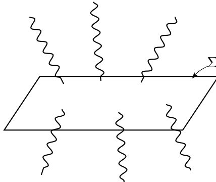
Figure 4.2. A spacelike hyperplane, \Sigma . The total energy contained in gravitational radiation is obtained by integrating t_{00} over \Sigma .
