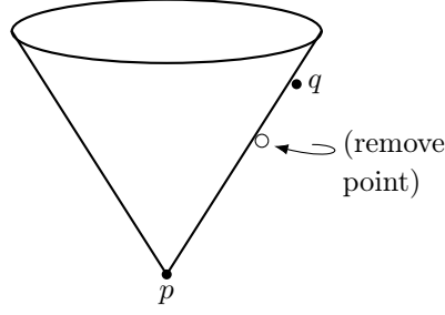
Figure 8.2. Minkowski spacetime with a point on the future light cone of p removed. In this spacetime, no causal curve connects p and q so q \notin J^+(p) but q \in \overline{J^+(p)} . Thus, J^+(p) is not closed.
