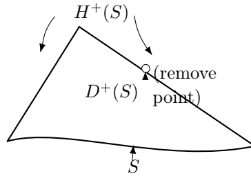
Figure 8.11. A spacetime diagram showing the future domain of dependence, D^+(S) , and Cauchy horizon H^+(S) of a particular closed achronal set S in Minkowski spacetime with a point removed.
