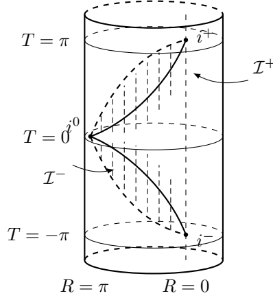
Figure 11.1. A spacetime diagram of the Einstein static universe. As described in the text, Minkowski spacetime is conformally isometric to the region \mathcal{O} = I^+(i^-) \cap I^-(i^+) of this spacetime. The boundary of \mathcal{O} —consisting of the points i^- , i^+ , and i^0 and the null hypersurfaces \mathcal{I}^- and \mathcal{I}^+ —defines a precise notion of “infinity” for Minkowski spacetime.
