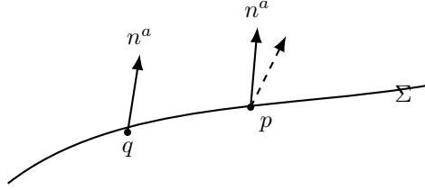
Figure 10.3. A spacetime diagram illustrating the notion of the extrinsic curvature of a hypersurface \Sigma . The dashed arrow at p represents the parallel transport of the normal vector, n^a , at q along a geodesic connecting q to p . The failure of this vector to coincide with n^a at p corresponds intuitively to the bending of \Sigma in the spacetime in which it is embedded. The formula K_{ab} = h_a{}^c \nabla_c n_b shows that K_{ab} directly measures this failure of the two vectors at p to coincide for q near p .
