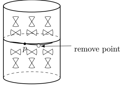
Figure 8.8. A spacetime which violates strong causality. The light cones “tip over” sufficiently that the curve drawn through p is a null geodesic (which, however, is not a closed curve because of the point removed from the manifold). There exist no closed causal curves in this spacetime, but there are causal curves through p which come “arbitrarily close” to intersecting themselves.
