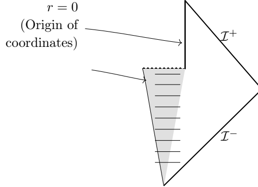
Figure 14.4. A conformal diagram of a spacetime in which a black hole is produced by the collapse of matter and “evaporates” as a result of the particle creation process.
