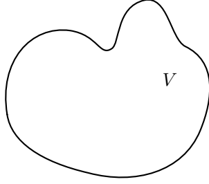
Figure 8.9. The neighborhood, V , of p used in the proof of the corollary to theorem 8.2.2.
