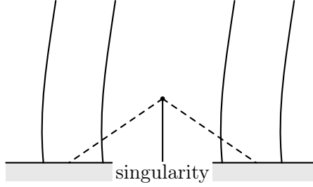
Figure 5.6. The causal structure of the Robertson–Walker solutions near the big-bang singularity. Particle horizons exist since an observer cannot “see” all other isotropic observers in the universe.
