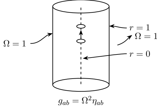
Figure 9.1. A spacetime diagram of a spacetime (\mathbb{R}^4, g_{ab}) conformal to Minkowski spacetime (\mathbb{R}^4, \eta_{ab}) , i.e., we have g_{ab} = \Omega^2 \eta_{ab} (see appendix D). The conformal factor \Omega is chosen to be spherically symmetric with \Omega = 1 for r > 1 . From the spherical symmetry of \Omega , it follows that the curve labeled r = 0 is a timelike geodesic of g_{ab} . If we choose \Omega so that \Omega(r = 0, t) \rightarrow 0 sufficiently rapidly as t \rightarrow \infty , this timelike geodesic will be incomplete. However, all spacelike and null geodesics simply “pass through” the world tube of nonzero curvature and thus are complete.
