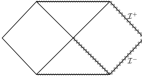
Figure 14.2. A conformal diagram of the extended Schwarzschild spacetime (see Figure 12.3) showing the oscillations of a wave of frequency \omega , i.e., \mathcal{L}_\xi \phi = -i\omega \phi . The apparent increase in oscillation frequency shown in the figure on \mathcal{I}^+ at late retarded time (which also occurs on \mathcal{I}^+ at early retarded time and on \mathcal{I}^- at late and early advanced times) is merely an artifact of the conformal diagram caused by the behavior of the conformal factor there. However, the increase in frequency shown on the white hole horizon near its crossing point with the black hole horizon represents a physical “infinite blueshift” singularity of the wave.
