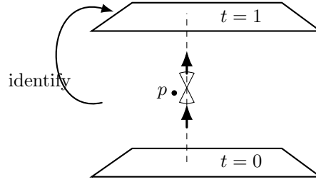
Figure 8.6. Minkowski spacetime with the hyperplanes t = 0 and t = 1 identified. A closed timelike curve through point p is shown.
