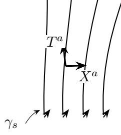
Figure 3.5. A one-parameter family of geodesics \gamma_s , with tangent T^a and deviation vector X^a .
