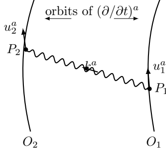
Figure 6.2. A spacetime diagram showing a light signal sent from static observer O_1 to static observer O_2 .
