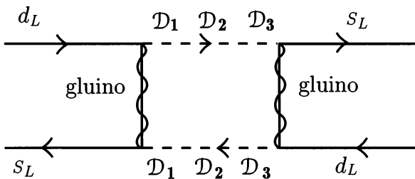
Figure 28.1. A one-loop diagram that can contribute to the \Delta S = 2 effective interaction (\bar{s}_L \gamma^\mu d_L)(\bar{s}_L \gamma_\mu d_L) in the supersymmetric standard model. Here solid lines are quarks; dashed lines are squarks; and combined solid and wavy lines are gluinos.
