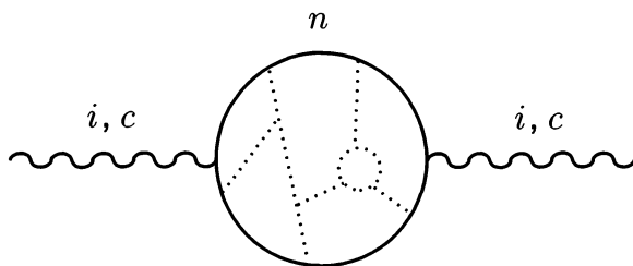
Figure 28.5. A diagram of the sort that introduces a breakdown of supersymmetry into the propagator of the gauge superfields. Here wavy lines are any component fields of the gauge superfields; solid lines are component fields of the messenger superfields; and dotted lines are component fields of the SU(3) \times SU(2) \times U(1) -neutral superfields of the supersymmetry-breaking sector.
