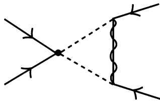
Figure 28.7. A diagram that can produce a four-fermion interaction among quarks and/or leptons that violates baryon and lepton number conservation. Here solid lines are quarks and/or leptons; dashed lines are squarks and/or sleptons; the combined solid and wavy line is a gaugino; and the dot is a vertex arising directly from the \mathcal{F} -term interactions (28.7.3).
