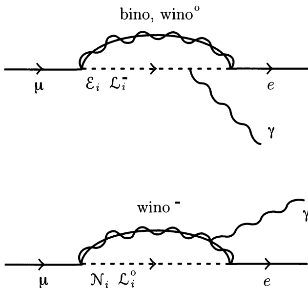
Figure 28.3. One-loop diagrams for the process \mu \rightarrow e + \gamma . Here solid lines are leptons; dashed lines are sleptons; combined solid and wavy lines are gauginos; and wavy lines are photons.
