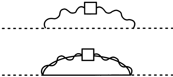
Figure 28.6. Diagrams that communicate supersymmetry breaking to the squarks and sleptons. Here dashed lines are squarks or sleptons; wavy lines are SU(3) \times SU(2) \times U(1) gauge bosons or auxiliary D fields; solid lines are quarks or leptons; combined solid and wavy lines are SU(3) \times SU(2) \times U(1) gauginos; and the squares represent insertions of the supersymmetry-breaking propagator correction shown in Figure 28.5.
