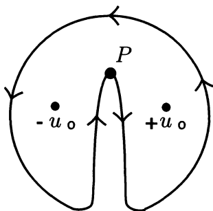
Figure 29.1. Deformation of a contour that circles the complex u plane counterclockwise at large |u| into a contour that starts at a base point P , circles the singularity at u = -u_0 counterclockwise back to P , and then circles the singularity at u = +u_0 counterclockwise back to P .
