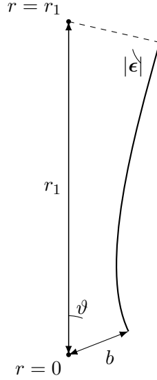
Figure 14.1. Quantities used in the calculation of parallaxes and apparent luminosities. The angles and the curvature of the light ray are greatly exaggerated.
