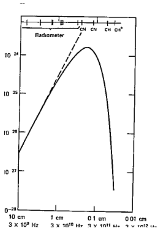
Figure 15.4. Energy density per frequency interval for 2.7°K black-body radiation. The solid curve gives the Planck spectrum (15.5.4); the dashed line gives the Rayleigh–Jeans spectrum (15.5.7) for an antenna temperature of 2.7°K. The short vertical lines mark frequencies at which the black-body temperature has been measured or bounded by radiometer or interstellar absorption observations.
