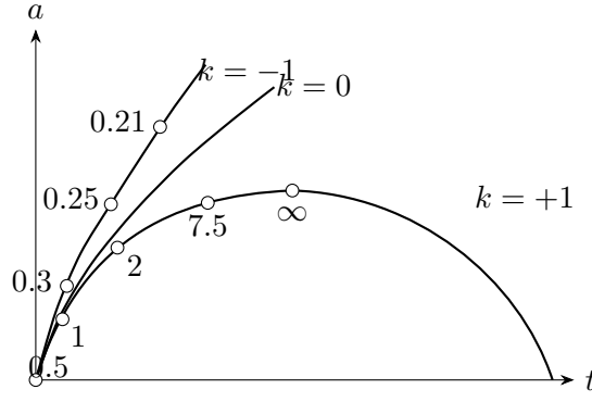
Figure 15.1. Solutions of Einstein's equations for a Robertson-Walker universe with curvature k = +1 , k = 0 , and k = -1 . The numbers along the curves k = \pm 1 give the values of the deceleration parameter q at various epochs.
