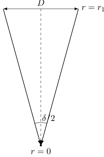
Figure 14.2. Quantities used in the calculation of angular diameters and proper motions. The angle \delta is greatly exaggerated.
