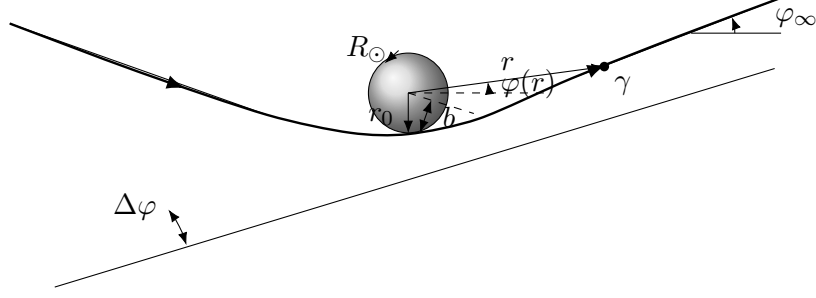
Figure 8.1. Quantities referred to in the calculation of the deflection of light by the sun. (Deflection greatly exaggerated.)
